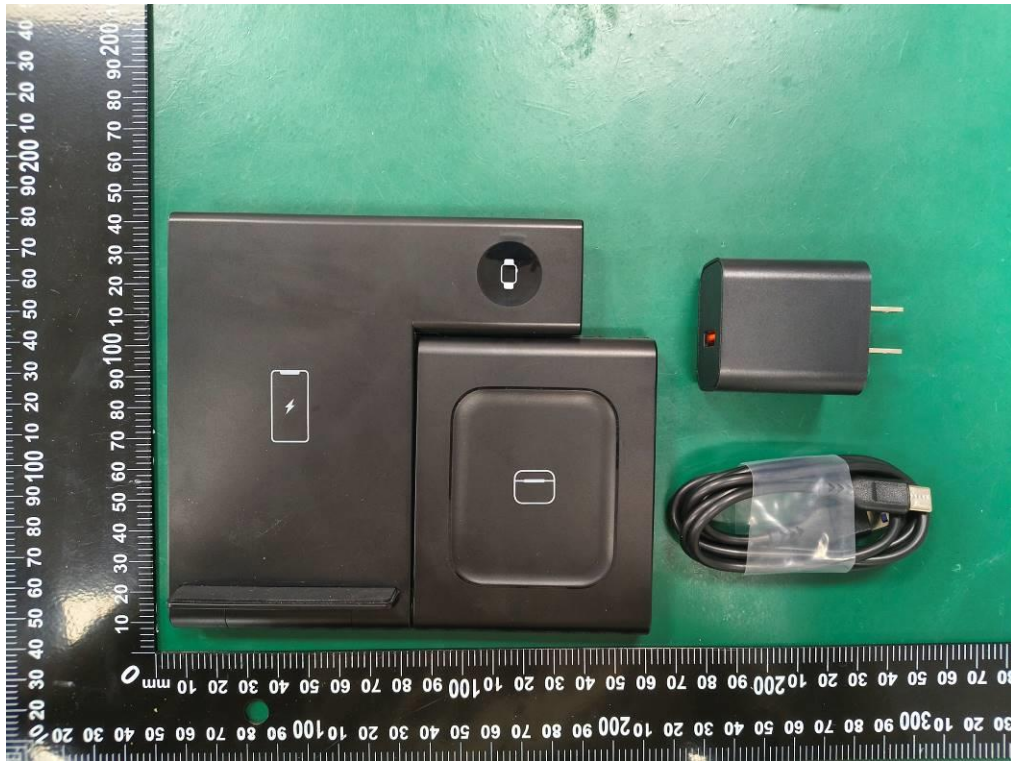
External Photo FCC ID: 2BBEH-W335B
