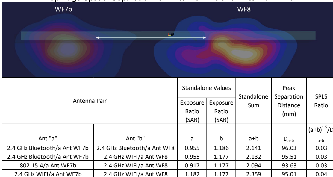
Top Edge Spatial Separation for Antenna WF8 and Antenna WF7b
