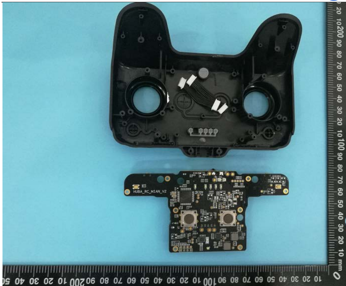
2. Mainboard front view
