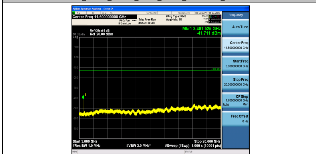
Band4_15MHz_16QAM_20325_1RB#0_3000~20000_3000~20000
