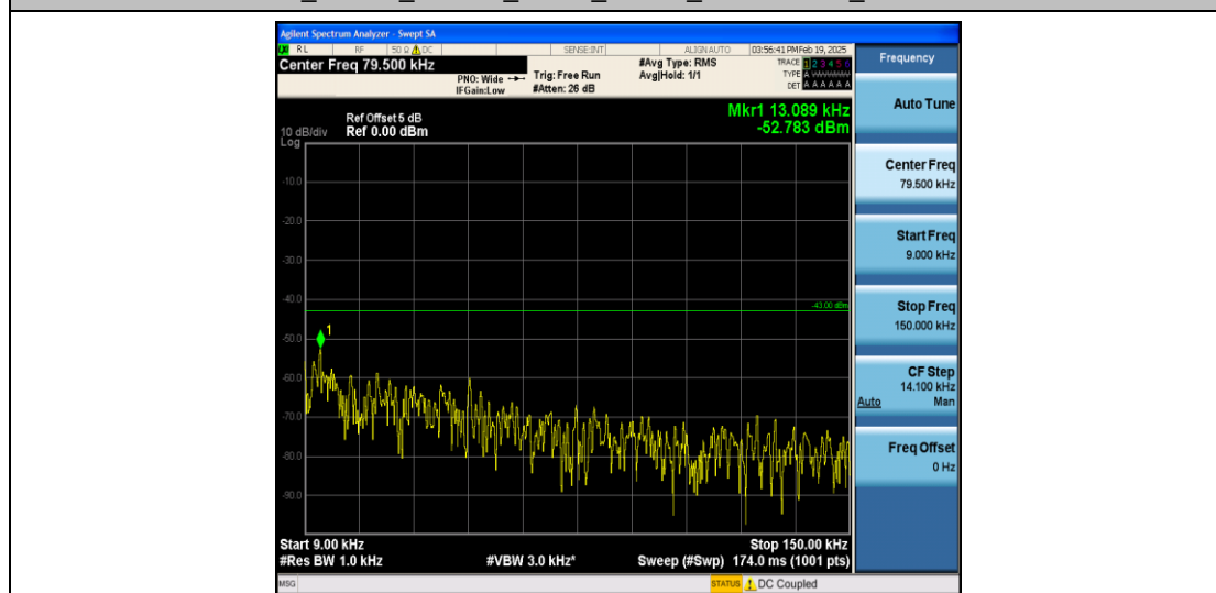
Band4_20MHz_QPSK_20300_1RB#0_0.009~0.15_0.009~0.15
