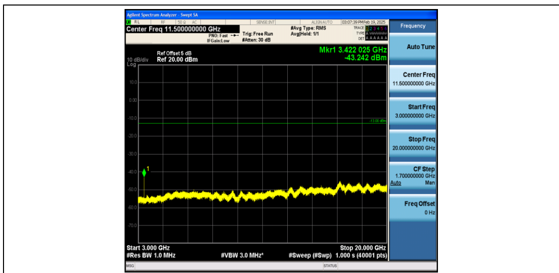
Band4_15MHz_QPSK_20025_1RB#0_3000~20000_3000~20000
