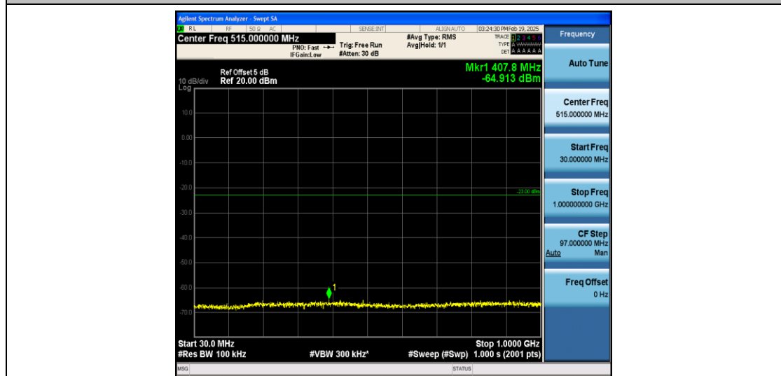
Band4_20MHz_QPSK_20050_1RB#0_30~1000_30~1000
