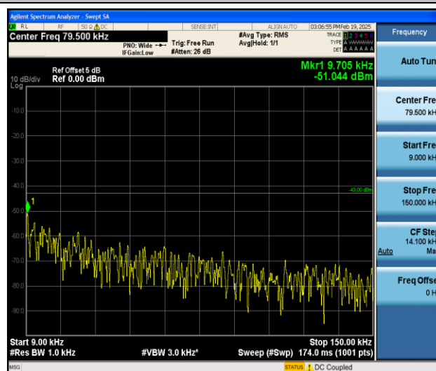
Band4_15MHz_QPSK_20025_1RB#0_0.009~0.15_0.009~0.15
