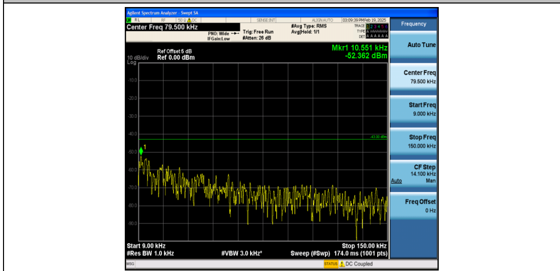
Band4_15MHz_16QAM_20175_1RB#0_0.009~0.15_0.009~0.15
