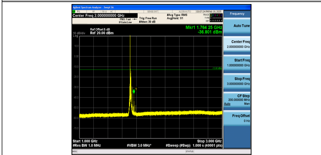
Band4_15MHz_QPSK_20025_1RB#0_1000~3000_1000~3000
