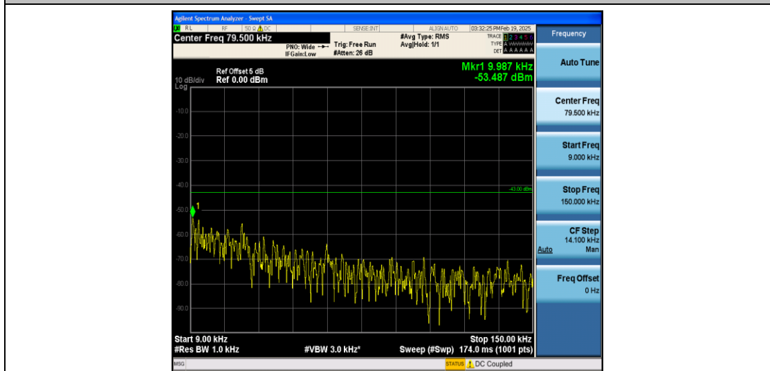
Band4_20MHz_16QAM_20050_1RB#0_0.009~0.15_0.009~0.15
