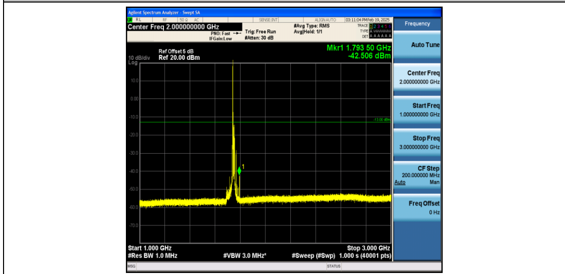
Band4_15MHz_QPSK_20325_1RB#0_1000~3000_1000~3000
