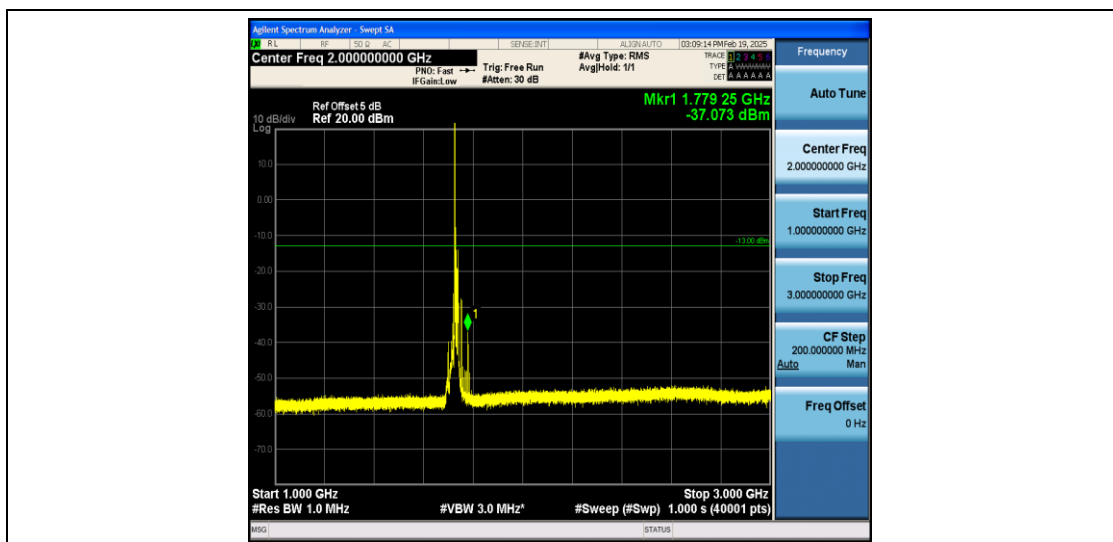
Band4_15MHz_QPSK_20175_1RB#0_1000~3000_1000~3000
