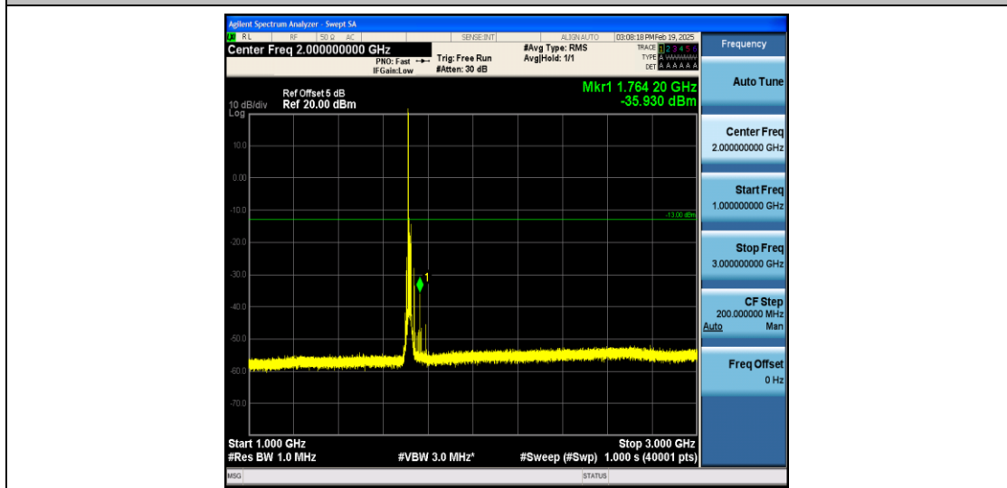
Band4_15MHz_16QAM_20025_1RB#0_1000~3000_1000~3000
