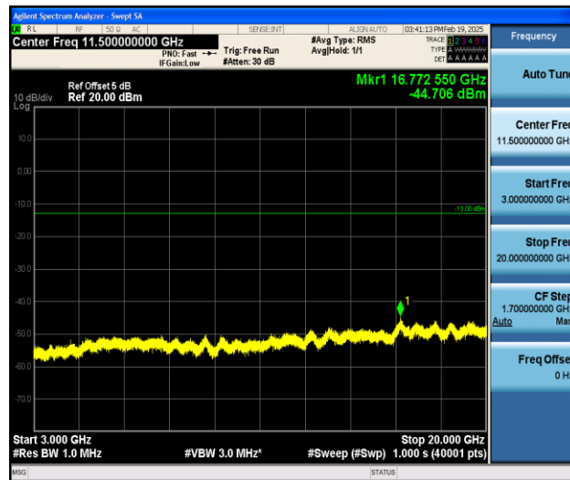
Band4_20MHz_QPSK_20175_1RB#0_3000~20000_3000~20000
