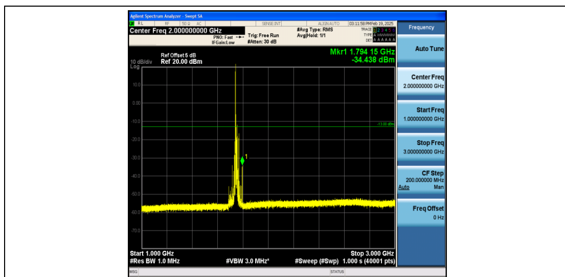
Band4_15MHz_16QAM_20325_1RB#0_1000~3000_1000~3000
