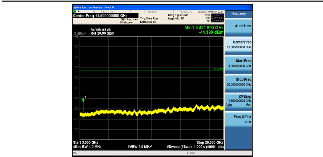
Band4_15MHz_16QAM_20025_1RB#0_3000~20000_3000~20000
