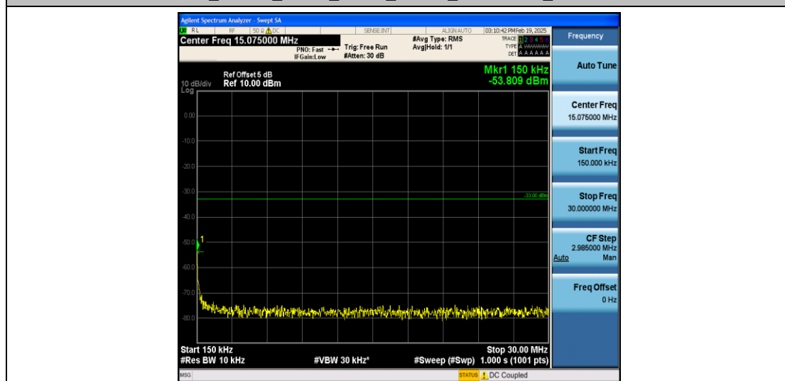
Band4_15MHz_QPSK_20325_1RB#0_0.15~30_0.15~30
