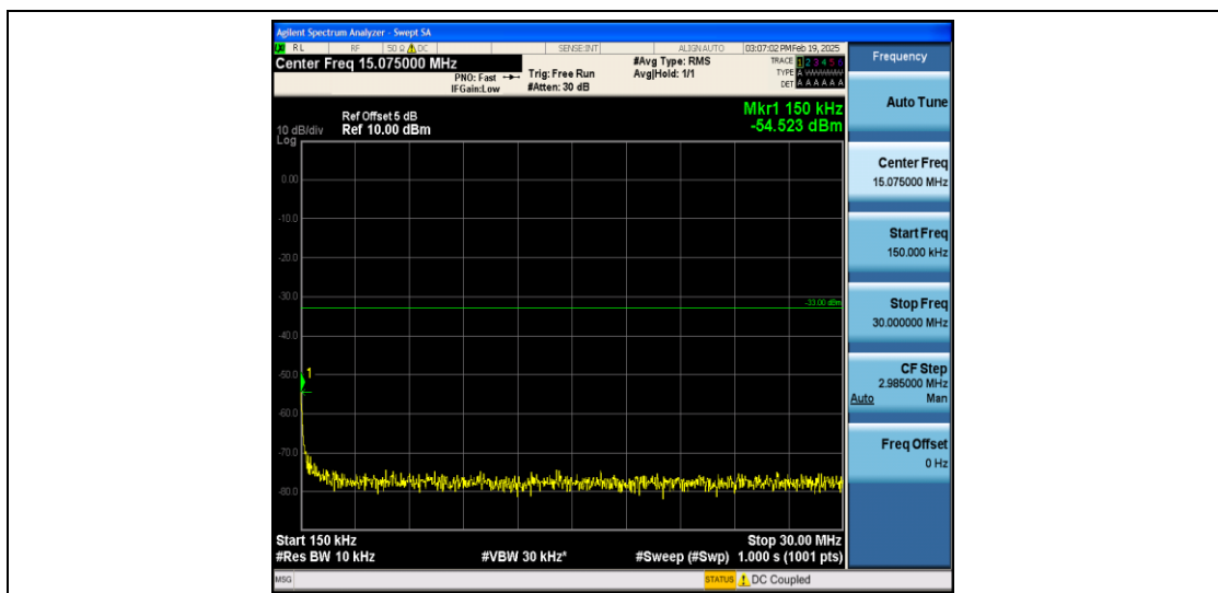
Band4_15MHz_QPSK_20025_1RB#0_0.15~30_0.15~30
