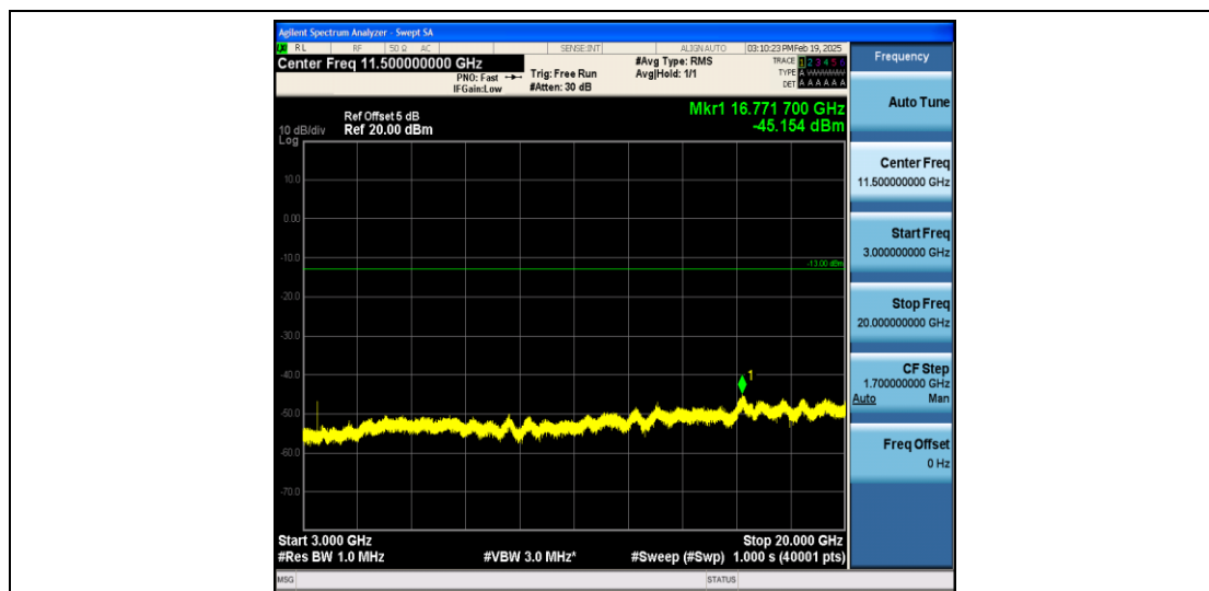
Band4_15MHz_16QAM_20175_1RB#0_3000~20000_3000~20000
