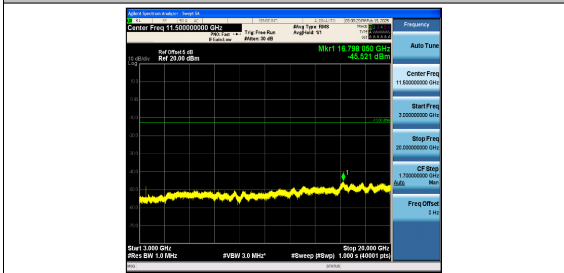
Band4_15MHz_QPSK_20175_1RB#0_3000~20000_3000~20000
