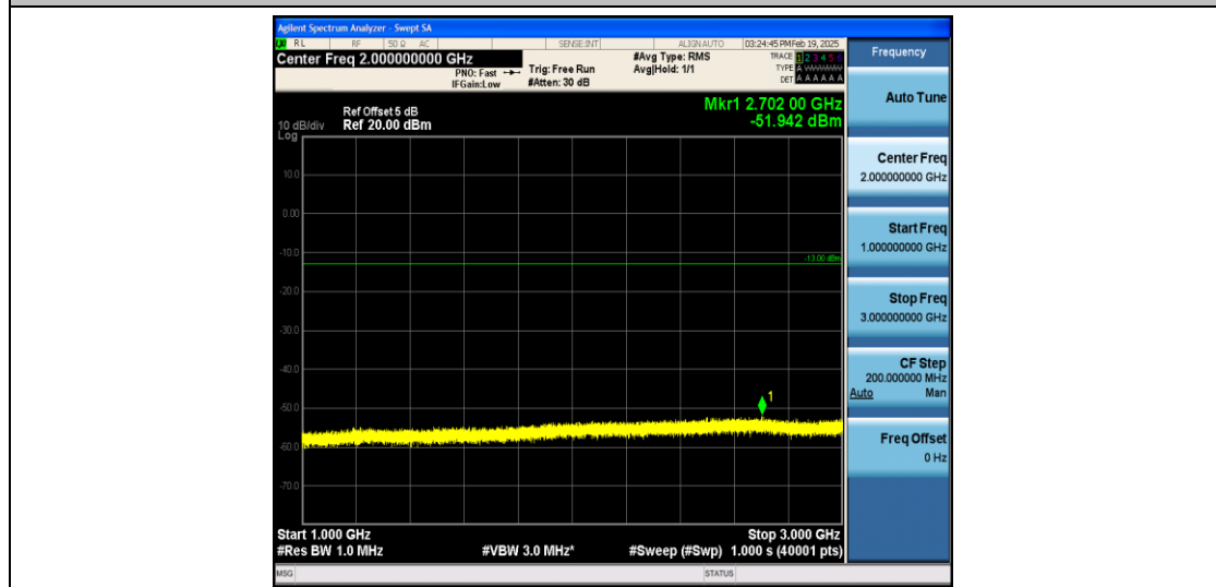
Band4_20MHz_QPSK_20050_1RB#0_1000~3000_1000~3000
