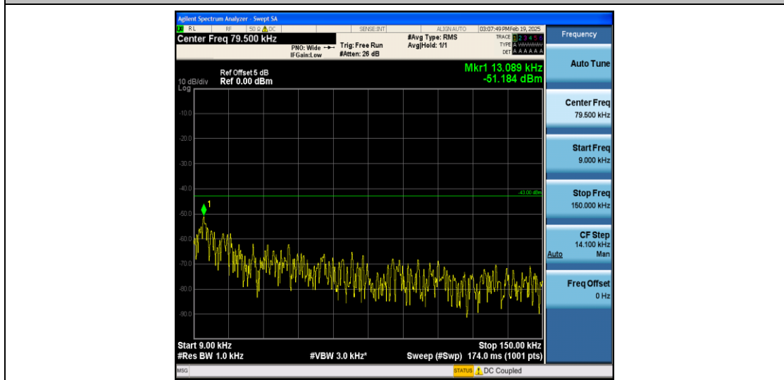
Band4_15MHz_16QAM_20025_1RB#0_0.009~0.15_0.009~0.15
