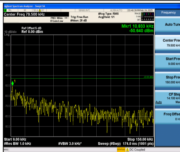
Band4_20MHz_16QAM_20175_1RB#0_0.009~0.15_0.009~0.15
