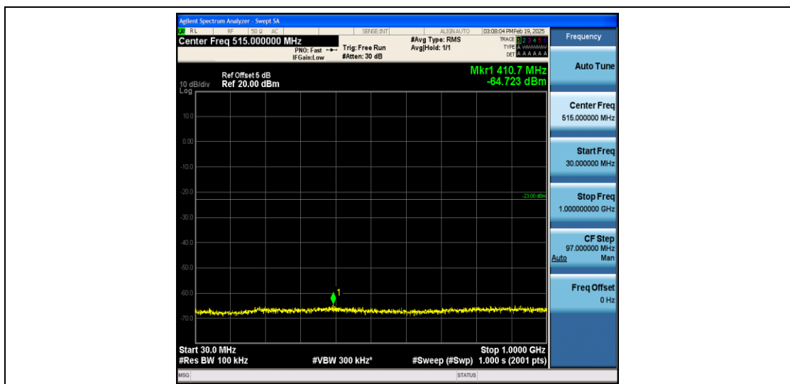
Band4_15MHz_16QAM_20025_1RB#0_30~1000_30~1000
