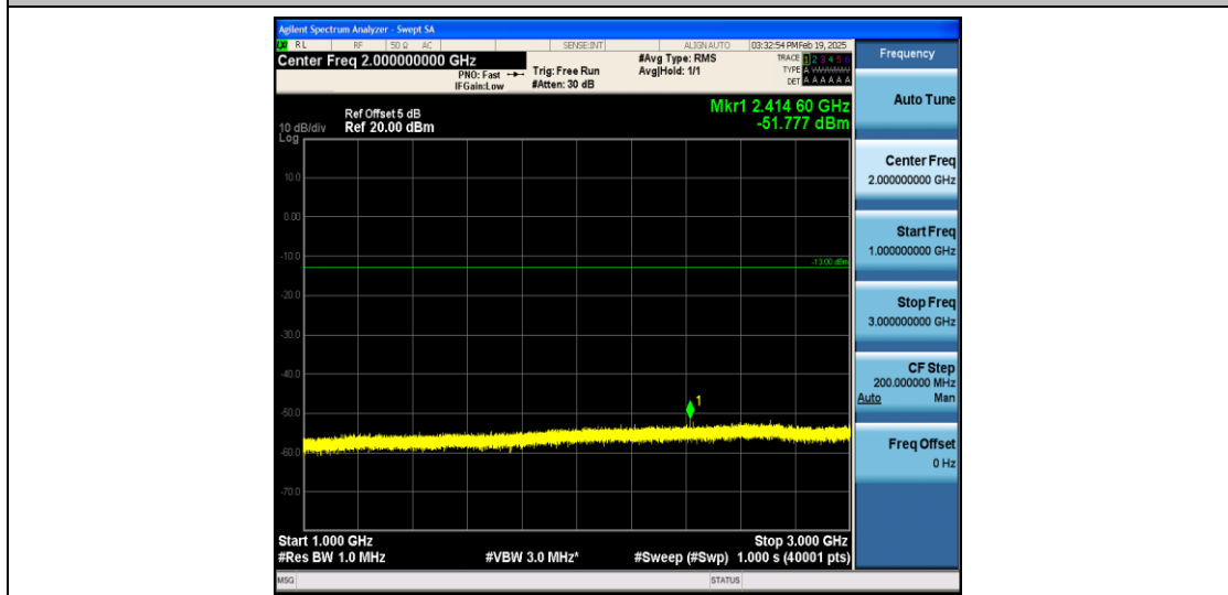
Band4_20MHz_16QAM_20050_1RB#0_1000~3000_1000~3000
