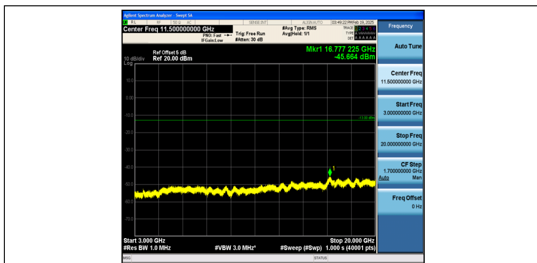
Band4_20MHz_16QAM_20175_1RB#0_3000~20000_3000~20000
