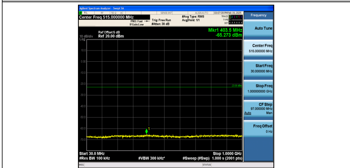
Band4_15MHz_QPSK_20025_1RB#0_30~1000_30~1000
