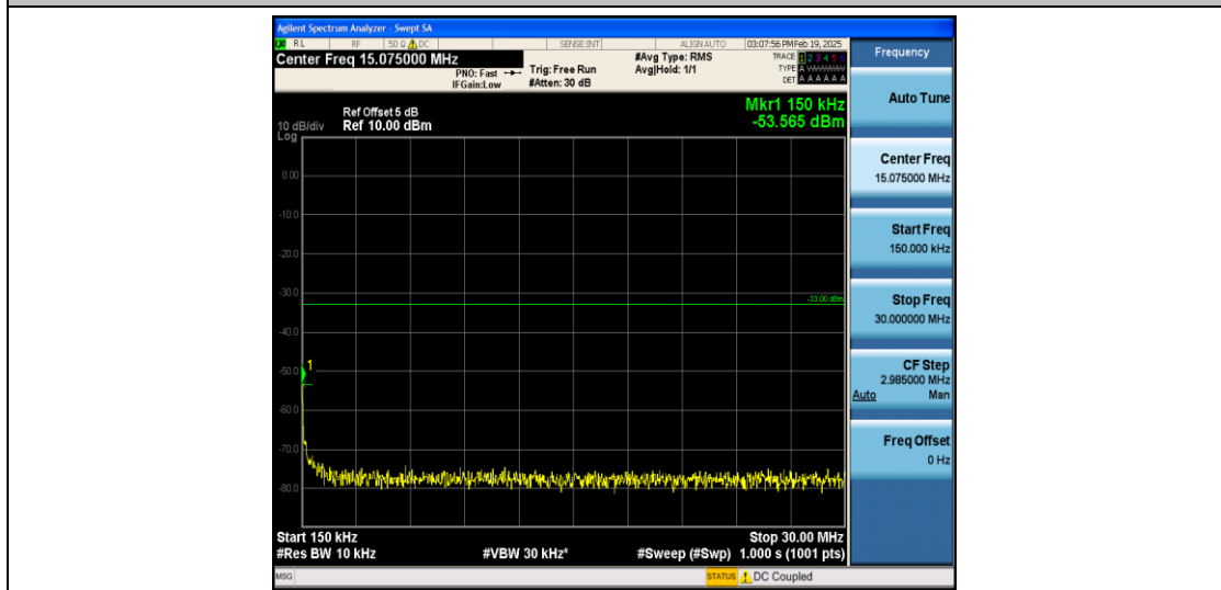
Band4_15MHz_16QAM_20025_1RB#0_0.15~30_0.15~30
