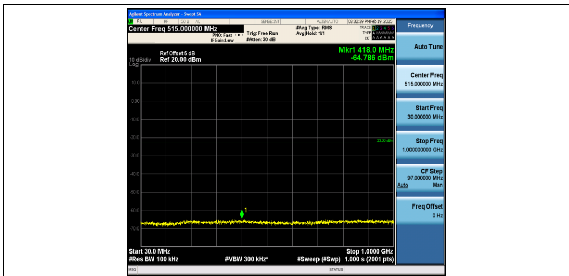
Band4_20MHz_16QAM_20050_1RB#0_30~1000_30~1000
