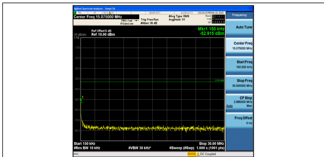
Band4_20MHz_QPSK_20050_1RB#0_0.15~30_0.15~30
