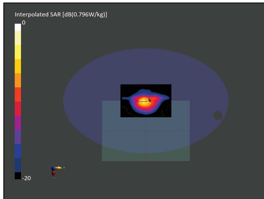
Figure C.15: SAR Testing Results for the A2992 at 2440.0 MHz
