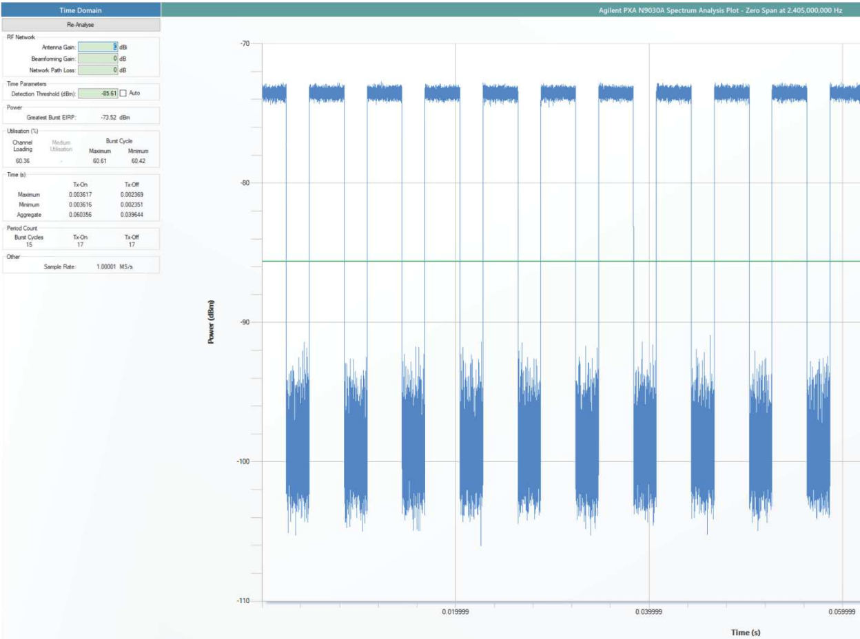
Figure 2 - Thread ePA - Frequency of 2405 MHz (60.61% Duty Cycle)
