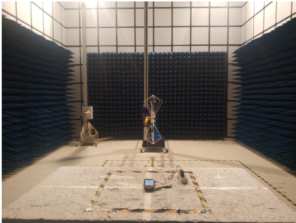
Radiated Emission
