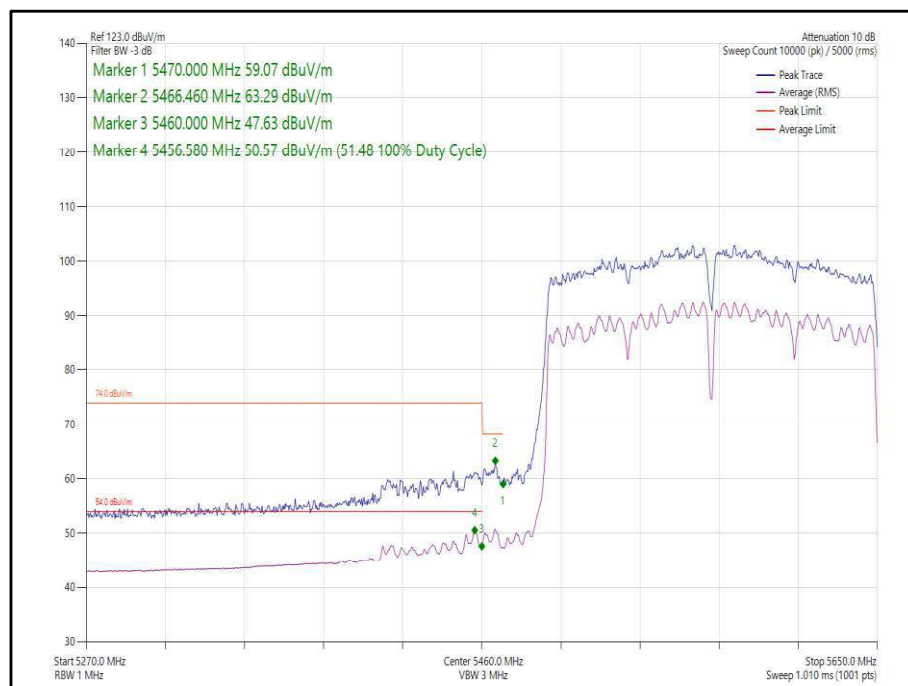
Figure 166 - 802.11ac, VHT160, SDM, Core 0-1 - 5570 MHz, Band Edge Frequency 5460 MHz
