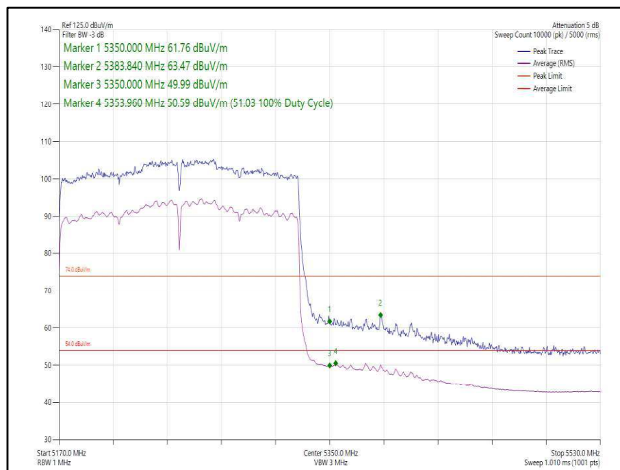
Figure 164 - 802.11ax, HE160, SU, SDM, Core 0-1 - 5250 MHz, Band Edge Frequency 5350 MHz
