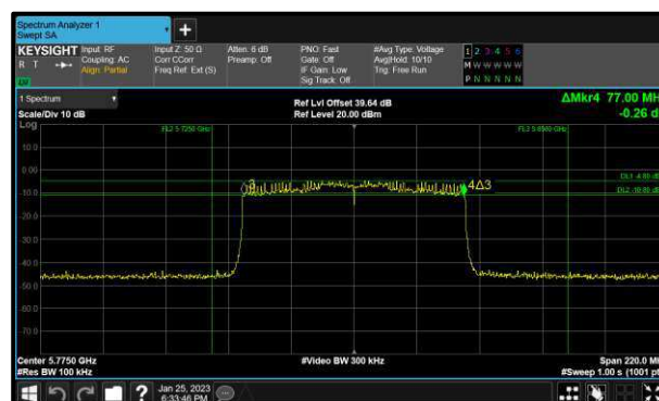
Figure 240 - 802.11ax HE80 SU Maximum 6 dB EBW
