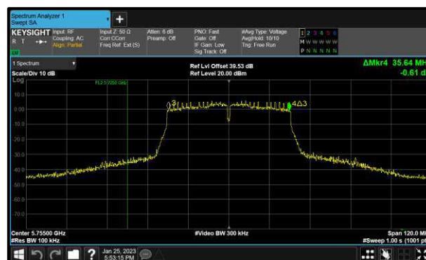
Figure 232 - 802.11n HT40 Maximum 6 dB EBW
