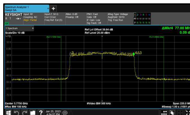
Figure 212 - 802.11ax HE80 SU Maximum 6 dB EBW
