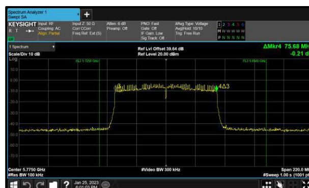
Figure 234 - 802.11ac VHT80 Maximum 6 dB EBW
