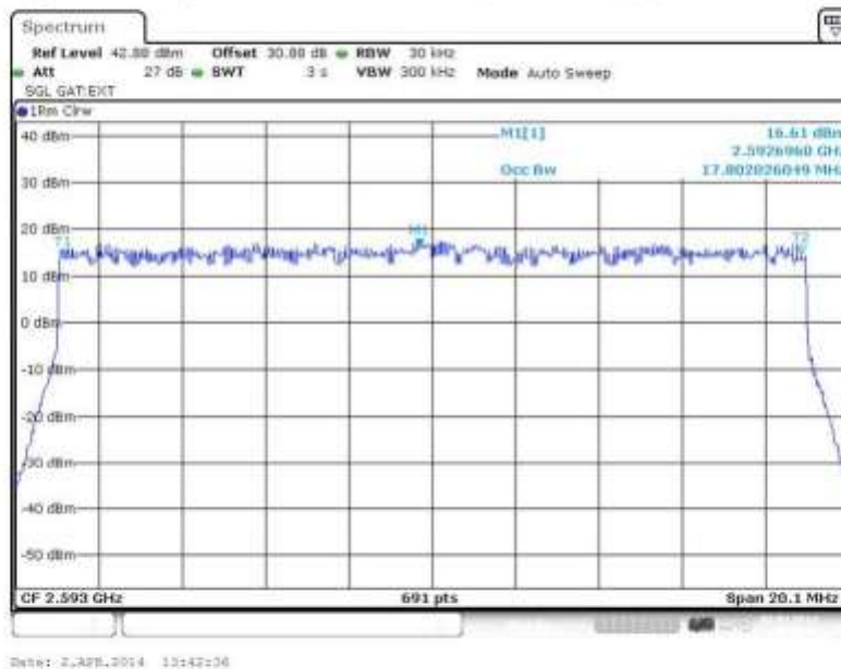
Figure 33 Occupied Bandwidth – 16QAM (2593.0 MHz) (20MHz Channel BW)
