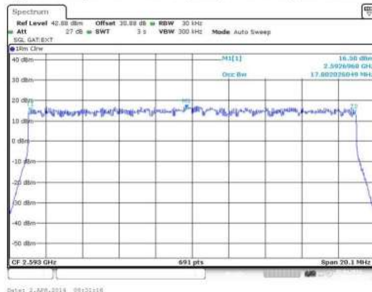
Figure 15 Occupied Bandwidth – 16QAM (2593.0 MHz) (20MHz Channel BW)
