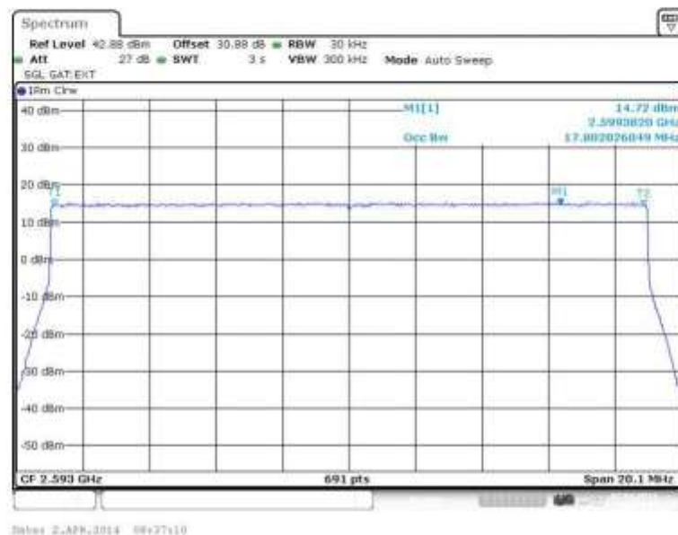
Figure 16 Occupied Bandwidth – 64QAM (2593.0 MHz) (20MHz Channel BW)
