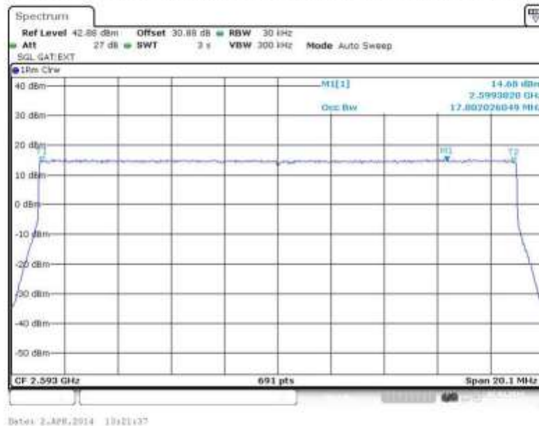
Figure 31 Occupied Bandwidth – 64QAM (2593.0 MHz) (20MHz Channel BW)
