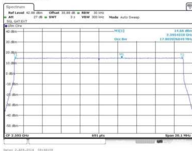
Figure 17 Occupied Bandwidth – QPSK (2593.0 MHz) (20MHz Channel BW)
