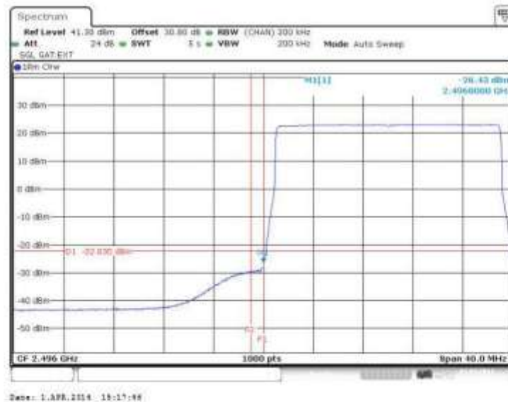
Figure 35 Spurious Emissions (Lower Band Edge) – QPSK (2506.0 MHz) (20MHz Channel BW)
