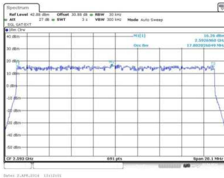
Figure 30 Occupied Bandwidth – 16QAM (2593.0 MHz) (20MHz Channel BW)
