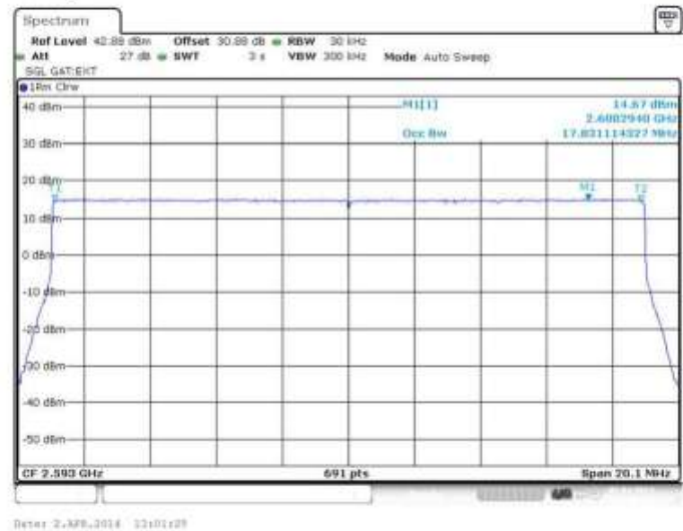
Figure 29 Occupied Bandwidth – QPSK (2593.0 MHz) (20MHz Channel BW)
