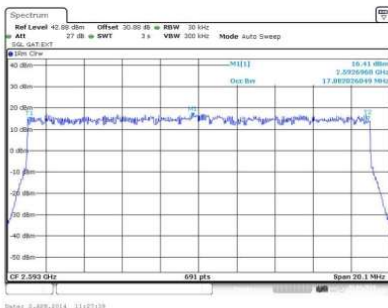
Figure 24 Occupied Bandwidth – 16QAM (2593.0 MHz) (20MHz Channel BW)
