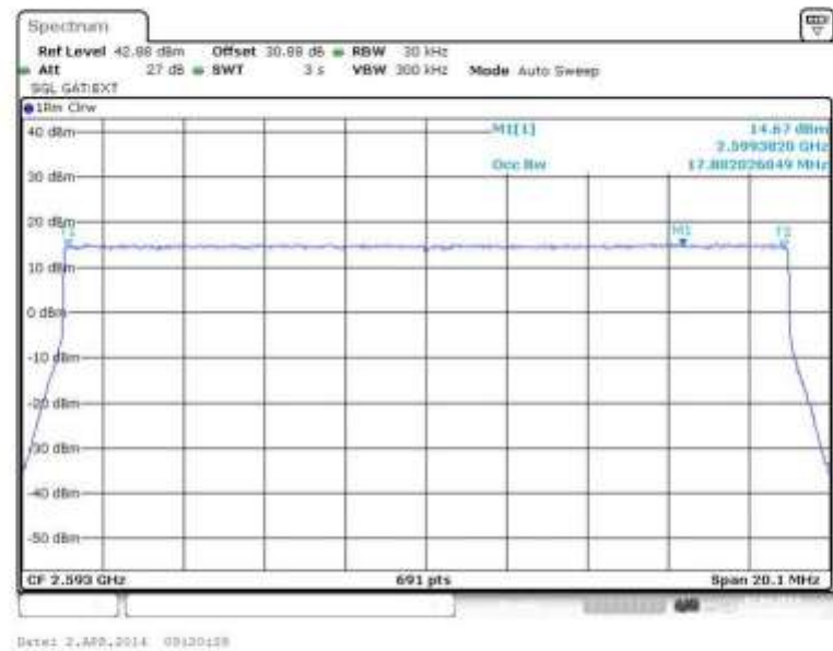
Figure 22 Occupied Bandwidth – 64QAM (2593.0 MHz) (20MHz Channel BW)
