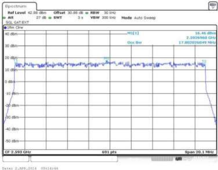
Figure 21 Occupied Bandwidth – 16QAM (2593.0 MHz) (20MHz Channel BW)
