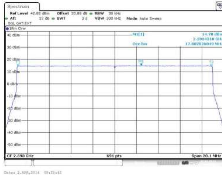
Figure 14 Occupied Bandwidth – QPSK (2593.0 MHz) (20MHz Channel BW)
