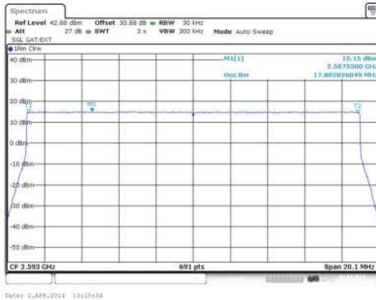
Figure 32 Occupied Bandwidth – QPSK (2593.0 MHz) (20MHz Channel BW)
