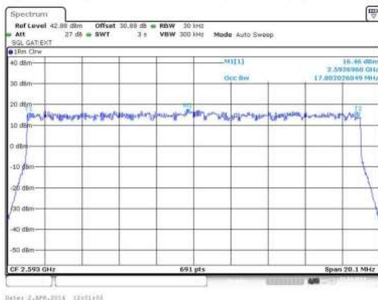
Figure 27 Occupied Bandwidth – 16QAM (2593.0 MHz) (20MHz Channel BW)
