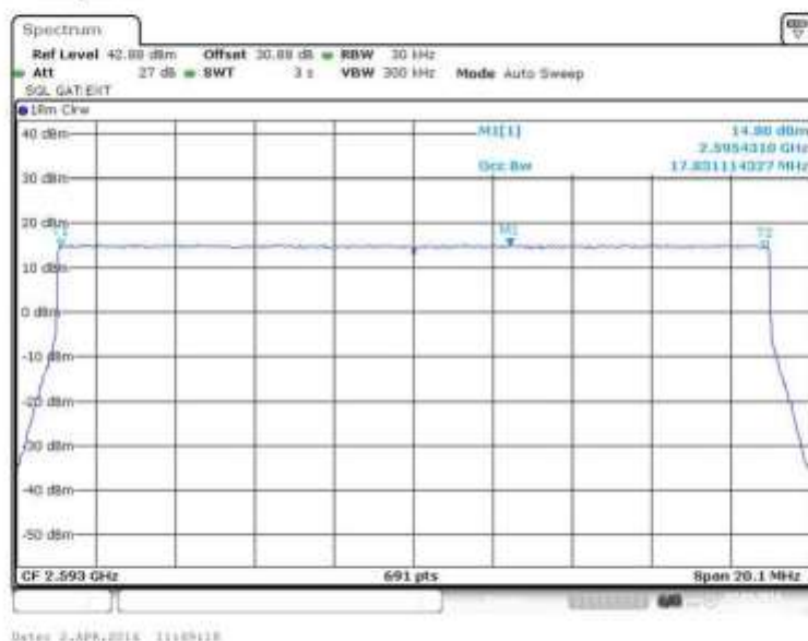
Figure 26 Occupied Bandwidth – QPSK (2593.0 MHz) (20MHz Channel BW)
