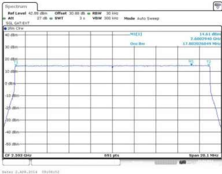
Figure 20 Occupied Bandwidth – QPSK (2593.0 MHz) (20MHz Channel BW)
