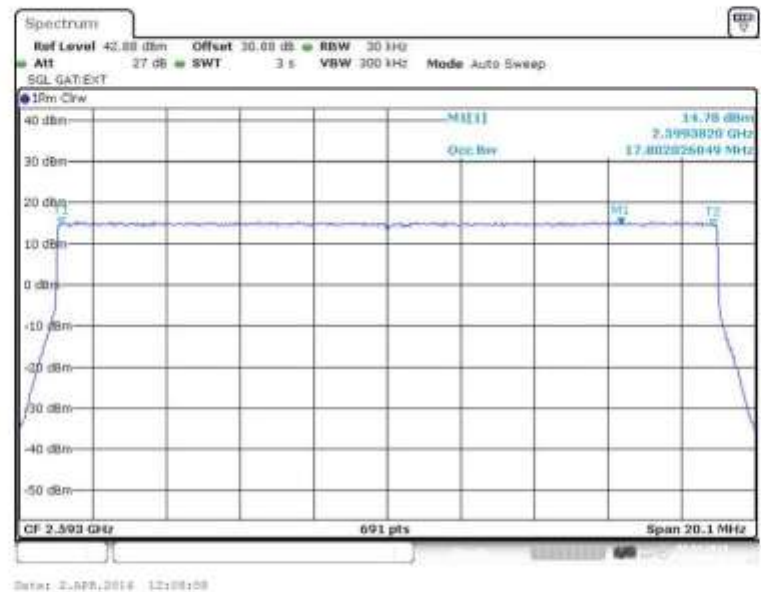
Figure 28 Occupied Bandwidth – 64QAM (2593.0 MHz) (20MHz Channel BW)
