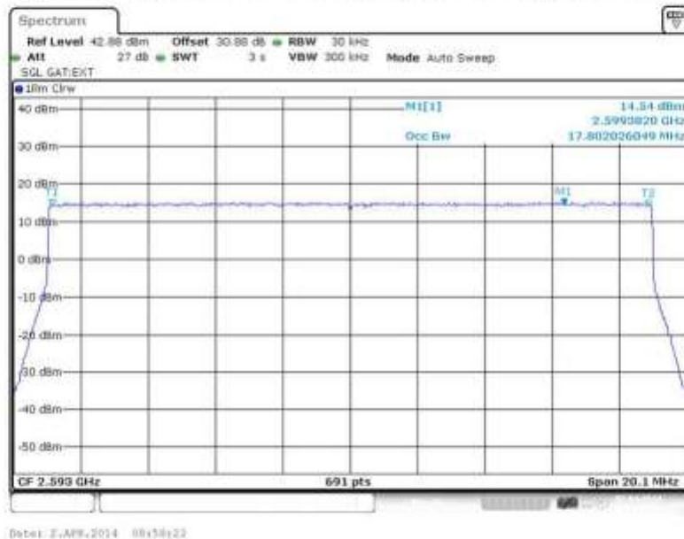
Figure 19 Occupied Bandwidth – 64QAM (2593.0 MHz) (20MHz Channel BW)
