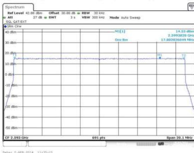
Figure 25 Occupied Bandwidth – 64QAM (2593.0 MHz) (20MHz Channel BW)
