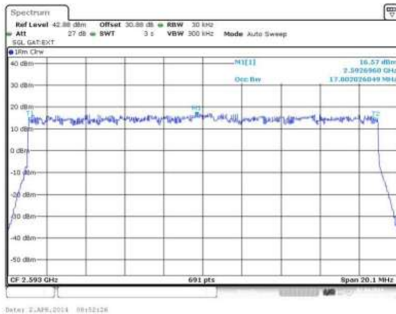
Figure 18 Occupied Bandwidth – 16QAM (2593.0 MHz) (20MHz Channel BW)
