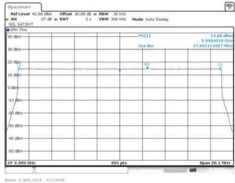
Figure 23 Occupied Bandwidth – QPSK (2593.0 MHz) (20MHz Channel BW)
