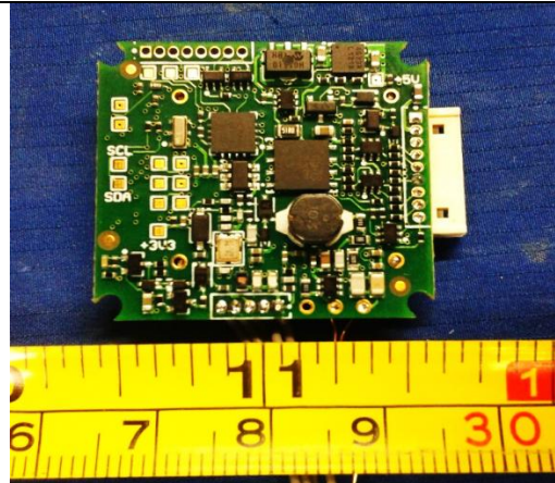
SE3200 Bottom View
