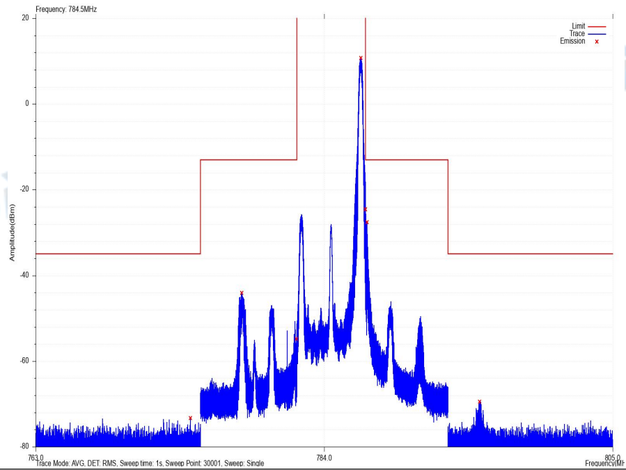
UP_EDGE_65_NT_NV_0_Band_13_QPSK_5M_CH23255_25_0
