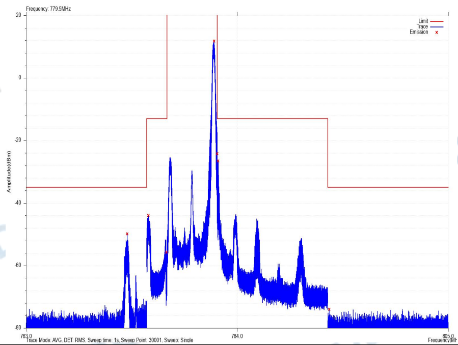
LOW_EDGE_65_NT_NV_0_Band_13_16QAM_5M_CH23205_1_24
