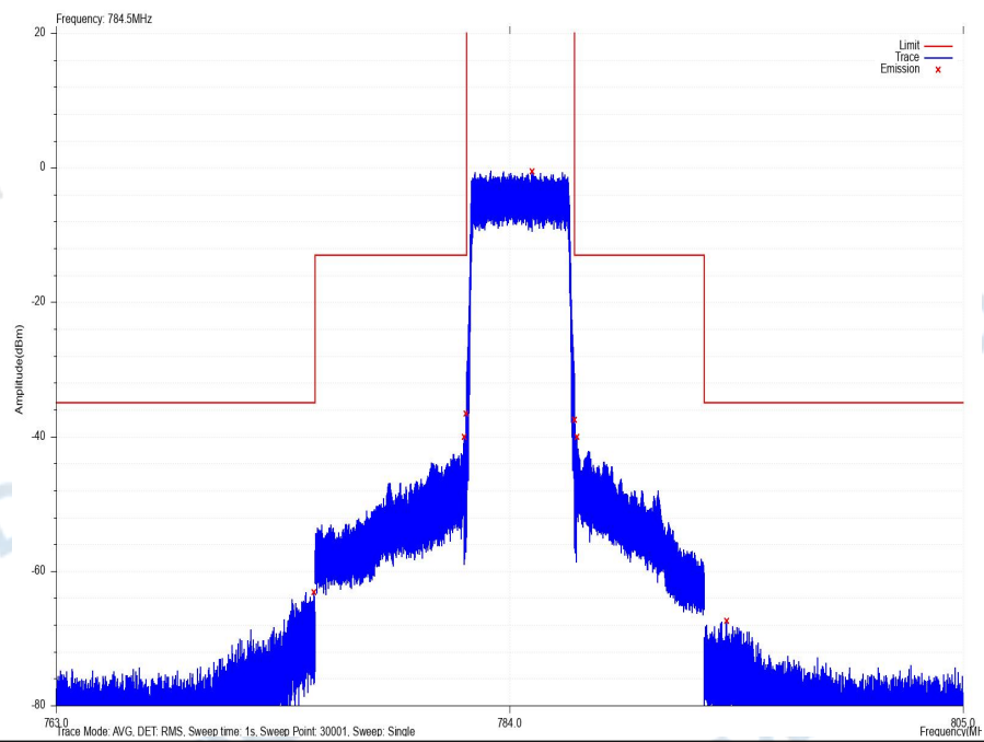
UP_EDGE_65_NT_NV_0_Band_13_QPSK_5M_CH23255_25_0
