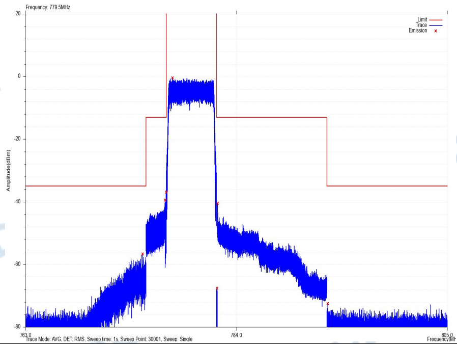
LOW_EDGE_65_NT_NV_0_Band_13_QPSK_5M_CH23205_25_0
