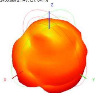
2430.0MHz H+V, Eff: 54.1%
