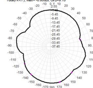
Total(H-XY), Max= -0.80dBi, CirD=9.15
