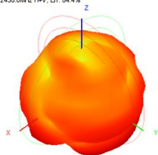
2435.0MHz H+V, Eff: 54.4%
