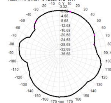
Total(H-XY), Max= 0.12dBi, CirD=9.11
