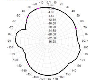
Total(H+V), Max= 0.55dBi, CirD=11.47
