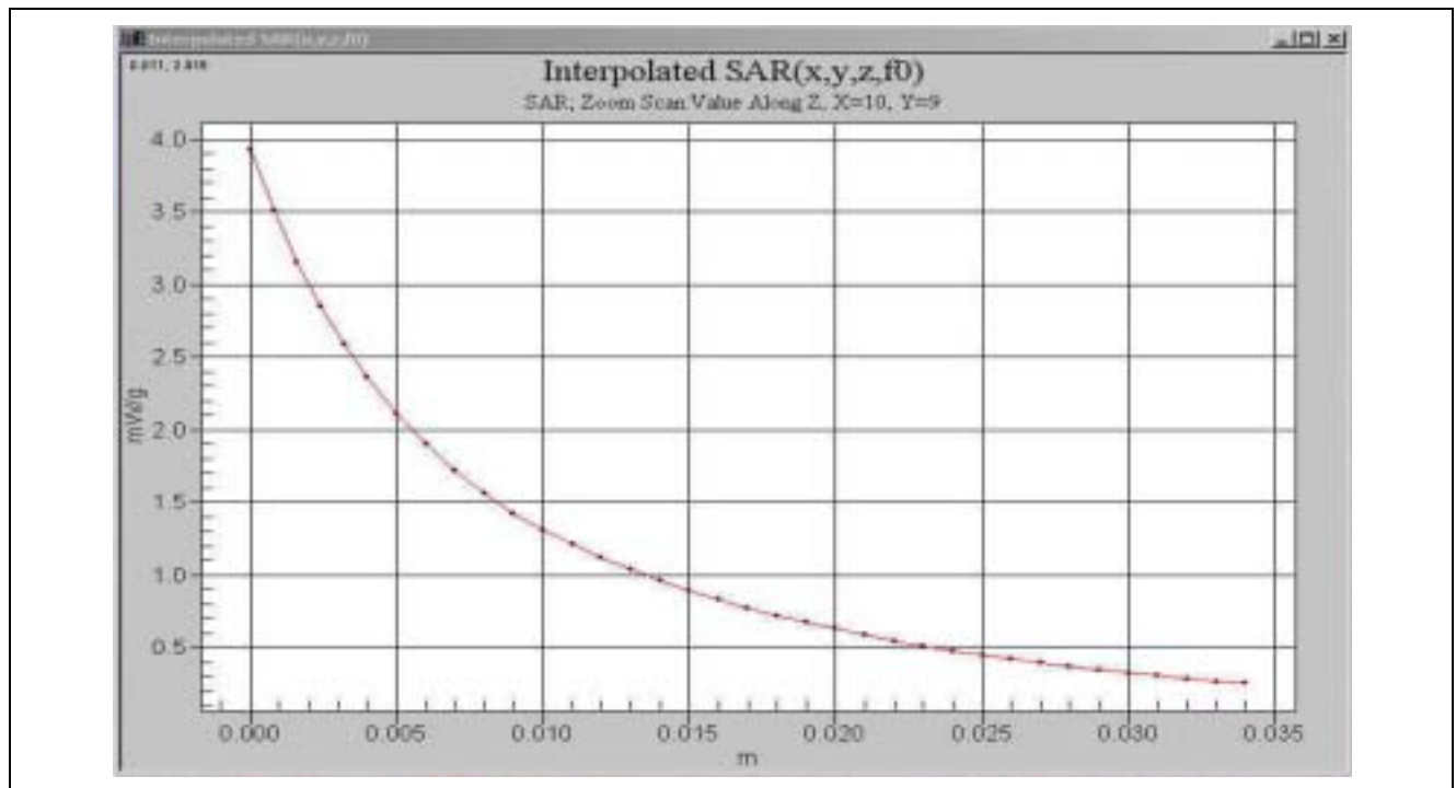
Muscle-Tissue-Simulating-Liquid 450MHz (2005/04/07)
