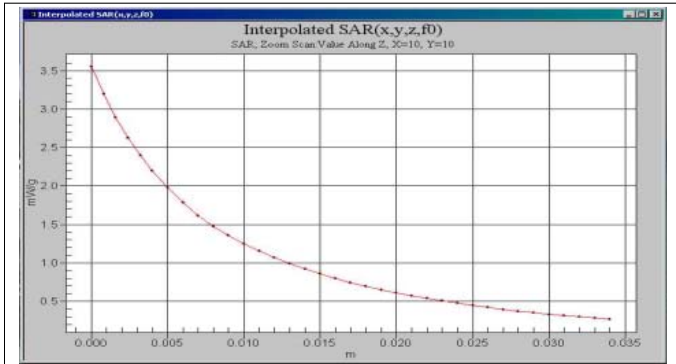
Head-Tissue-Simulating-Liquid 450MHz (2005/03/24)
