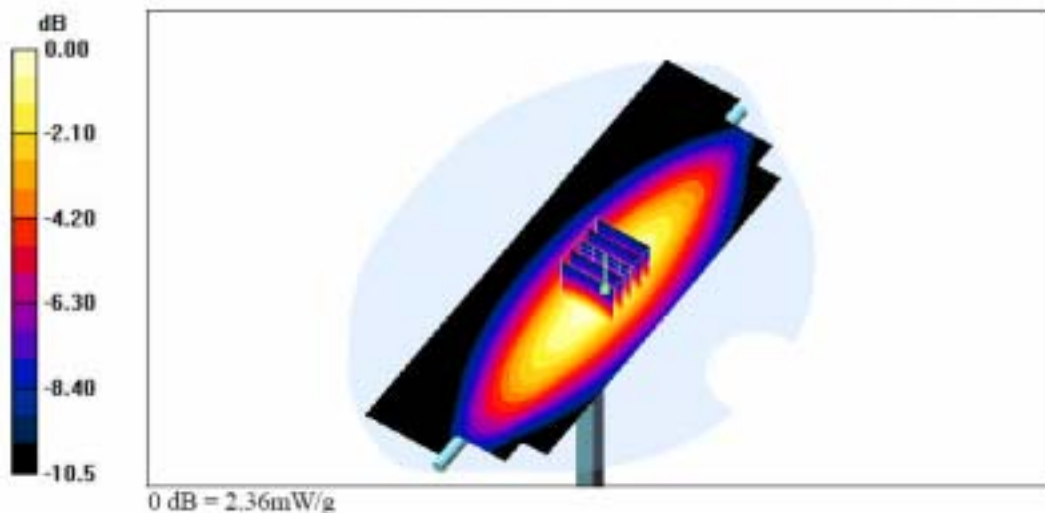
Muscle-Tissue-Simulating-Liquid 450MHz (2005/04/07)
