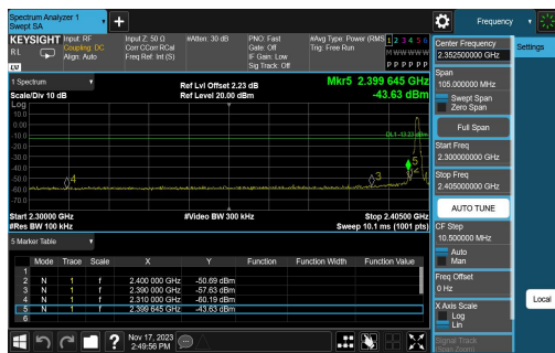
BLE_500K-Ant1-2402-PASS
