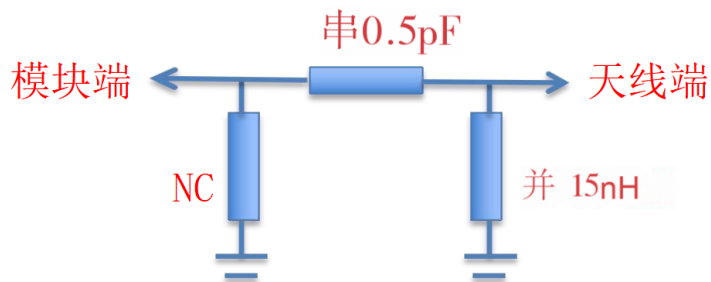
Antenna Matching Circuit Diagram
