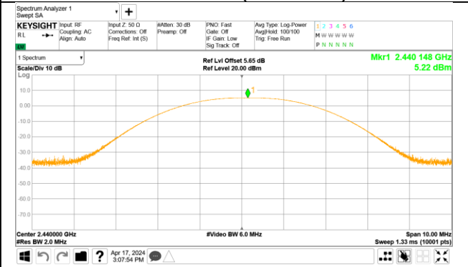
Channel 19 (2440MHz)
