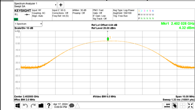
Channel 0 (2402MHz)
