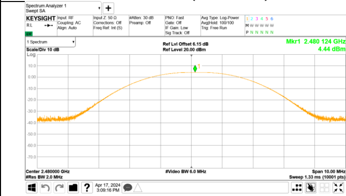
Channel 39 (2480MHz)
