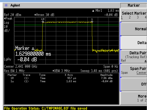
8-DPSK DH3
