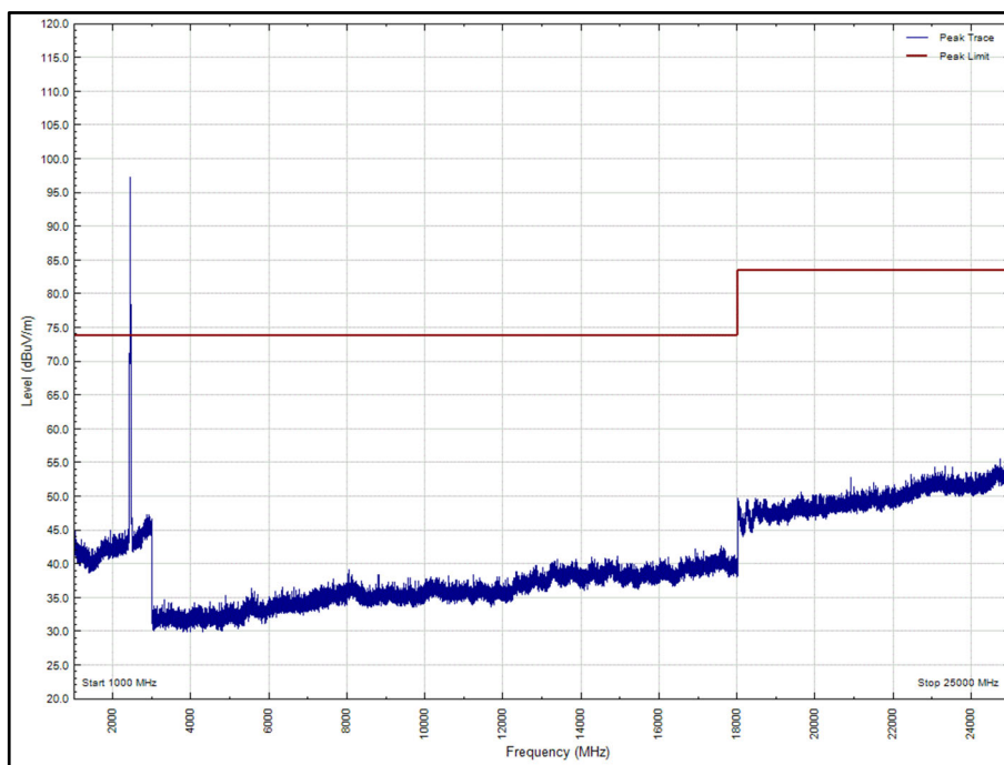
Figure 116 - 2437 MHz - 1 GHz to 25 GHz, Vertical, EUT Orientation: X, Peak
