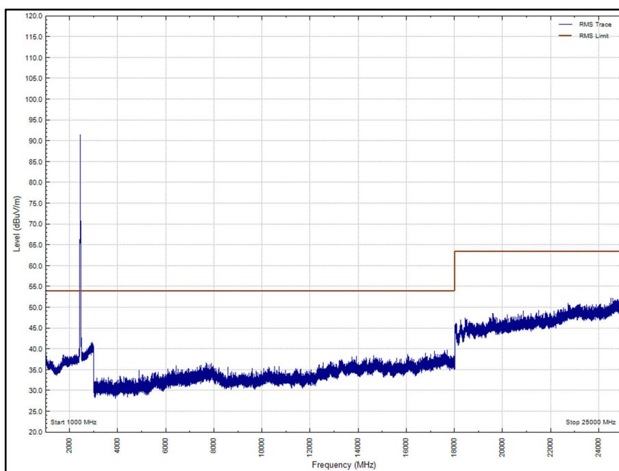
Figure 117 - 2437 MHz - 1 GHz to 25 GHz, Vertical, EUT Orientation: X, Average
