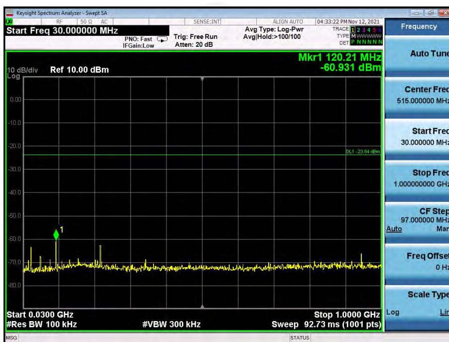
30MHz~1GHz
