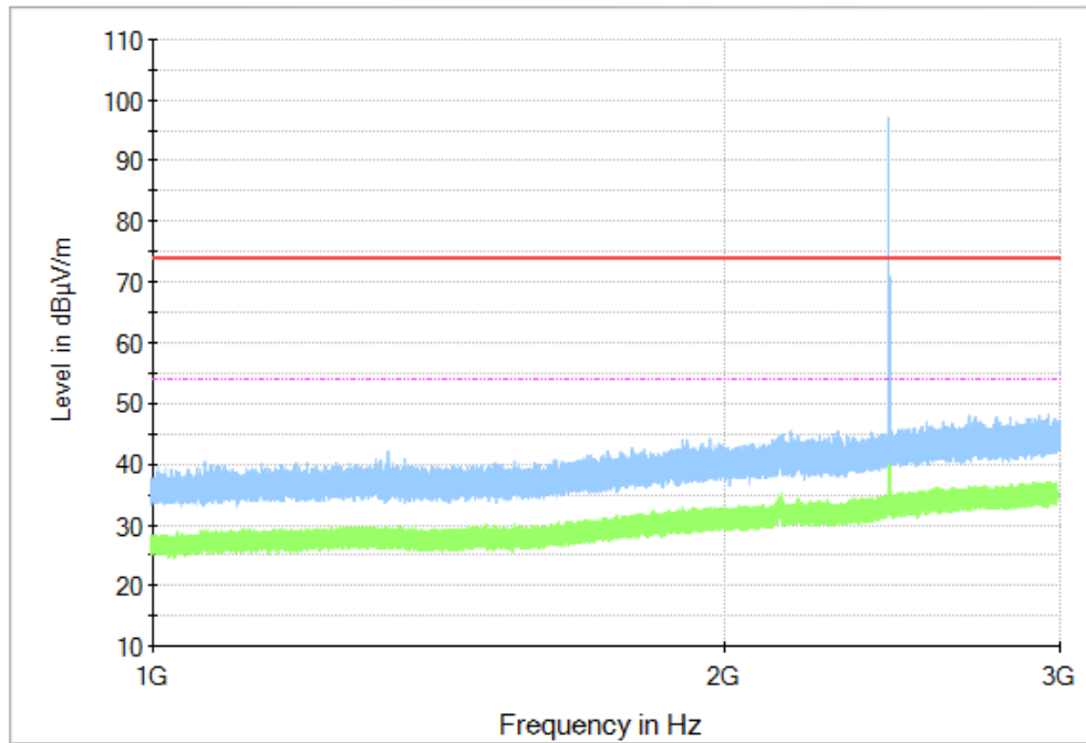
Fig. 33 Radiated Spurious Emission (GFSK, Ch0, 1 GHz ~3 GHz)
