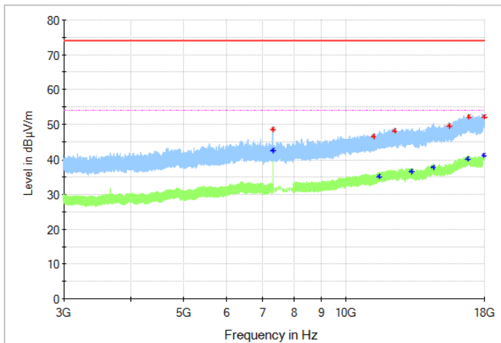
Fig. 36 Radiated Spurious Emission (GFSK, Ch39, 3 GHz ~18 GHz)
