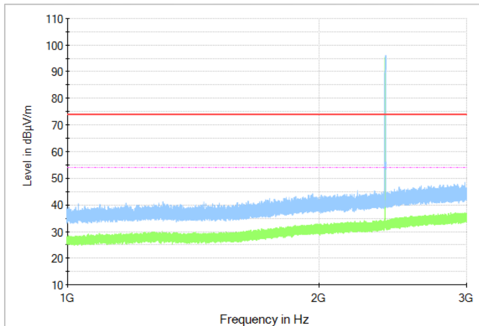
Fig. 49 Radiated Spurious Emission (8DPSK, Ch0, 1 GHz ~3 GHz)
