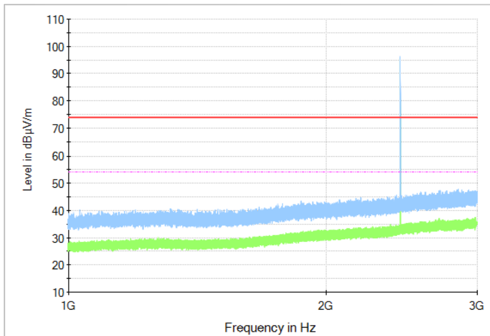
Fig. 35 Radiated Spurious Emission (GFSK, Ch39, 1 GHz ~3 GHz)
