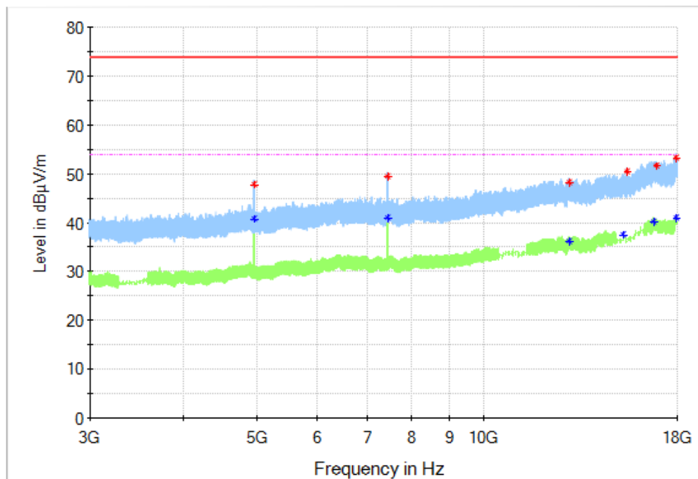
Fig. 54 Radiated Spurious Emission (8DPSK, Ch78, 3 GHz ~18 GHz)
