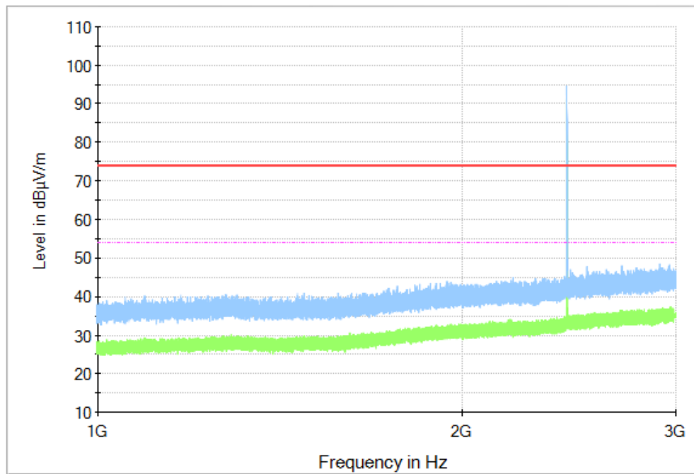
Fig. 51 Radiated Spurious Emission (8DPSK, Ch39, 1 GHz ~3 GHz)
