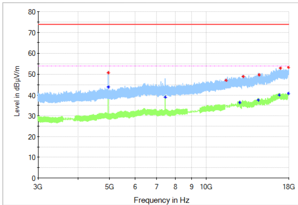
Fig. 46 Radiated Spurious Emission ( \pi/4 DQPSK, Ch78, 3 GHz ~18 GHz)
