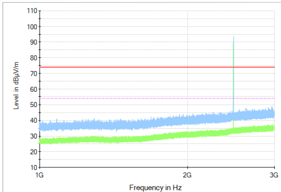
Fig. 53 Radiated Spurious Emission (8DPSK, Ch78, 1 GHz ~3 GHz)
