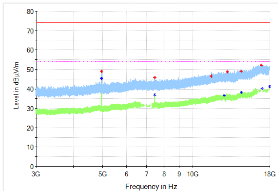
Fig. 38 Radiated Spurious Emission (GFSK, Ch78, 3 GHz ~18 GHz)
