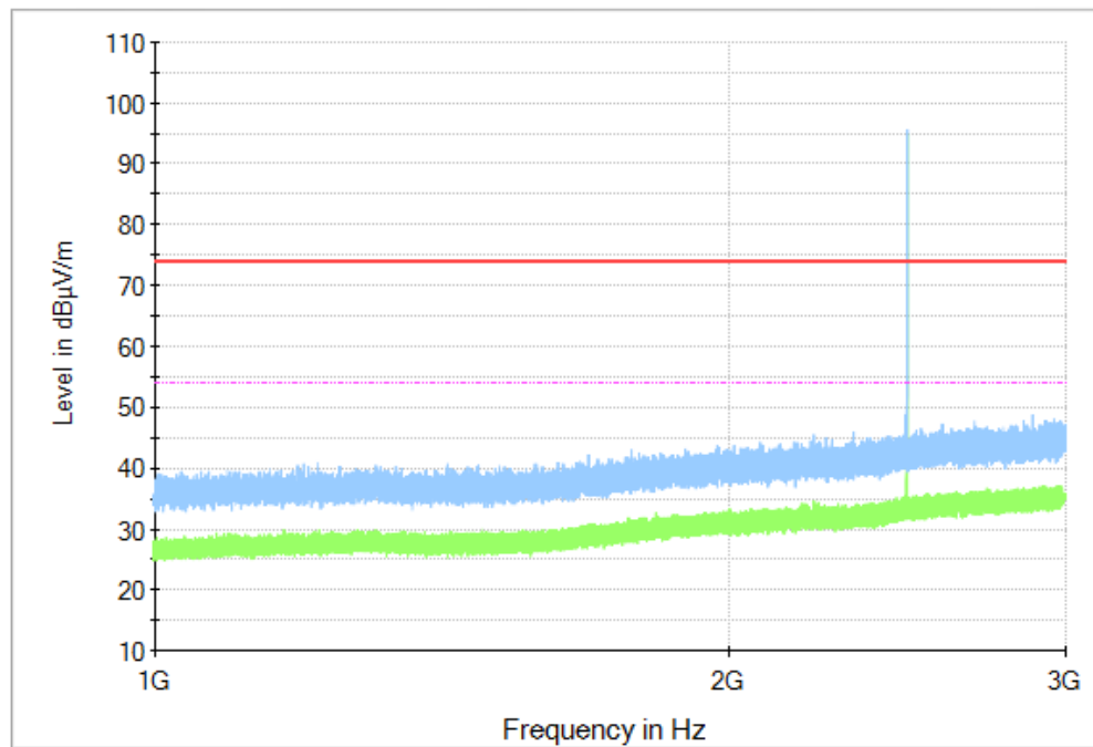
Fig. 37 Radiated Spurious Emission (GFSK, Ch78, 1 GHz ~3 GHz)
