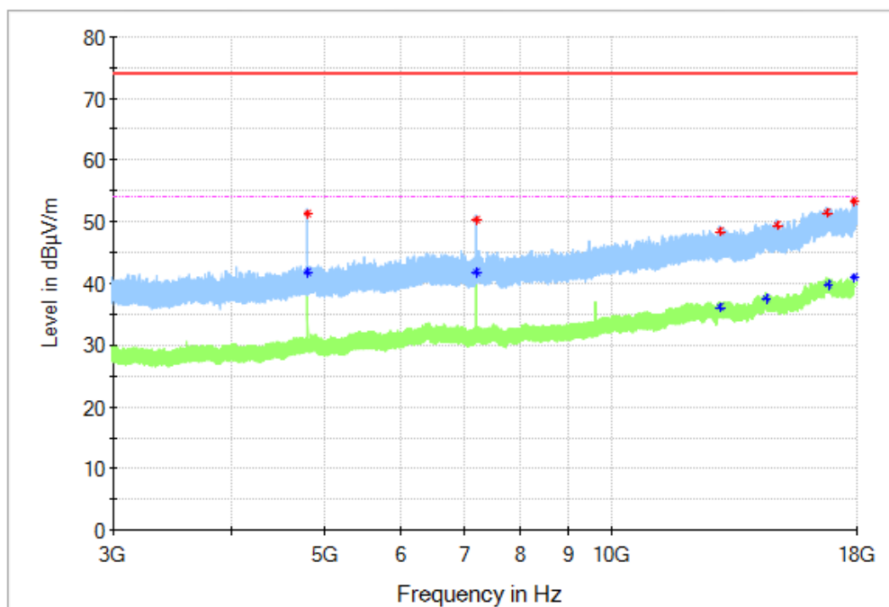
Fig. 50 Radiated Spurious Emission (8DPSK, Ch0, 3 GHz ~18 GHz)
