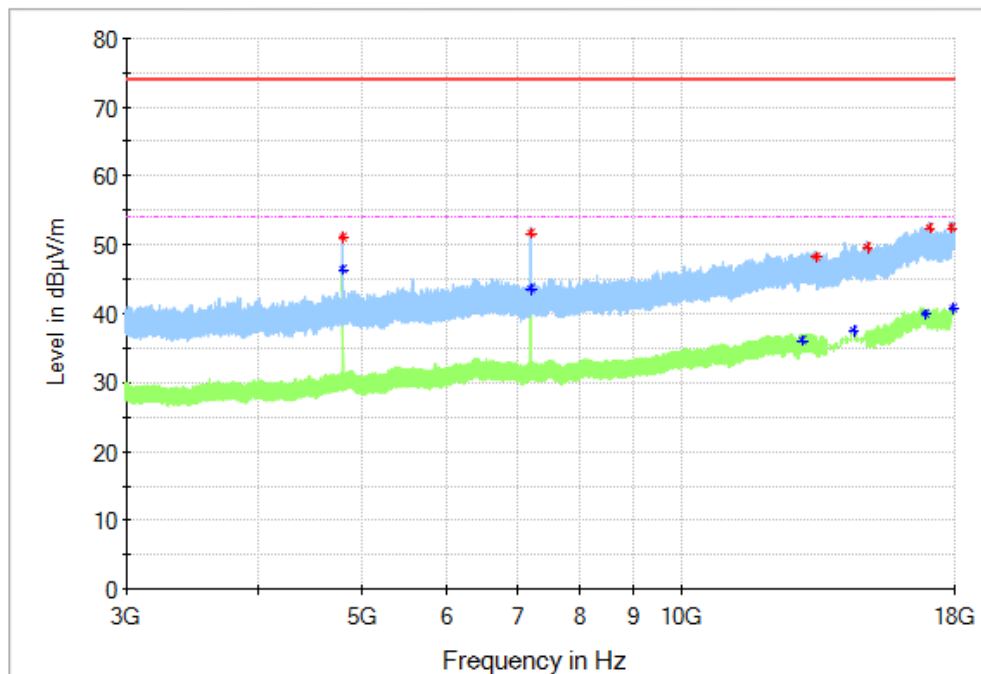
Fig. 34 Radiated Spurious Emission (GFSK, Ch0, 3 GHz ~18 GHz)
