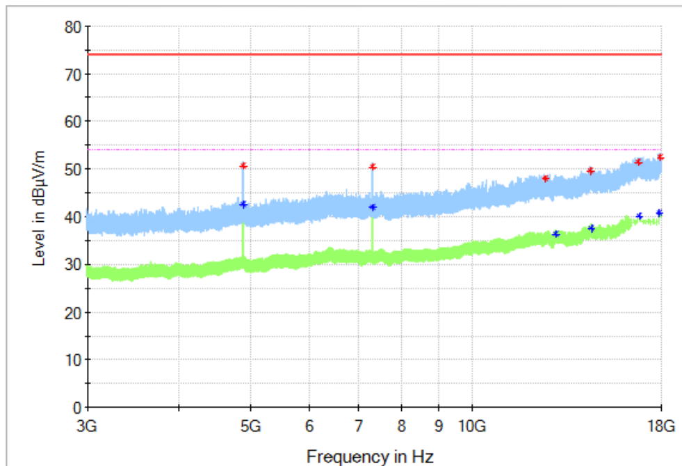
Fig. 52 Radiated Spurious Emission (8DPSK, Ch39, 3 GHz ~18 GHz)
