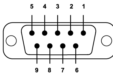
Figure 2.2.1. DB-9 (Female)
