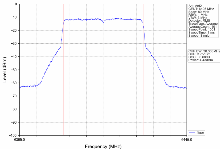
802.11ax(HEW40)_HCH_6405MHz_RU484_Left_Ant2_NTNV
