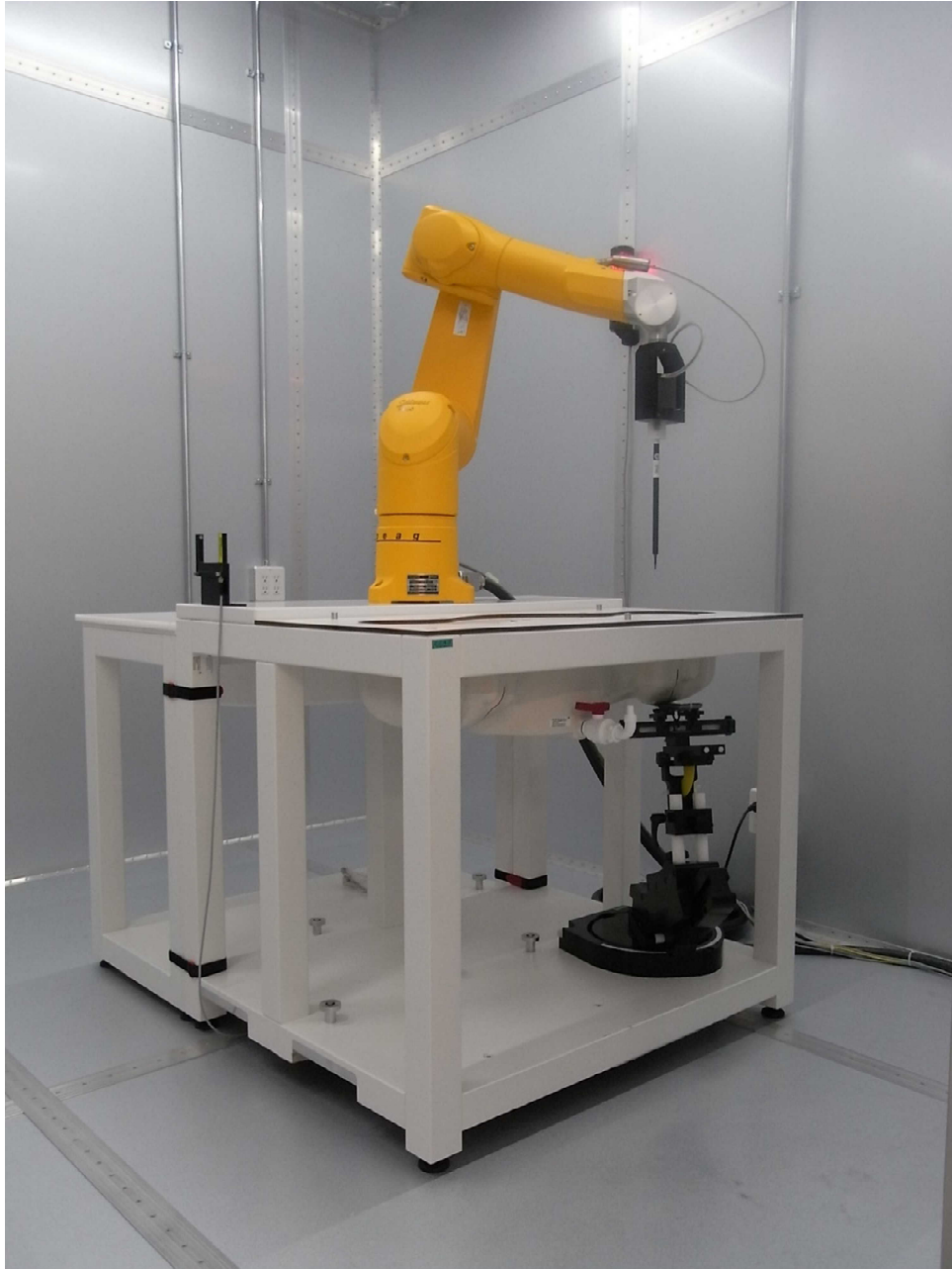
Test setup photo (Head SAR Test photo Left section)
