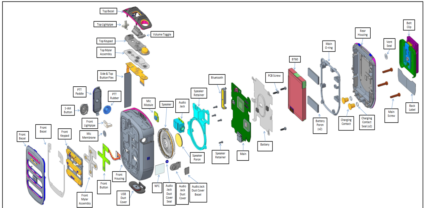
Exploded View
