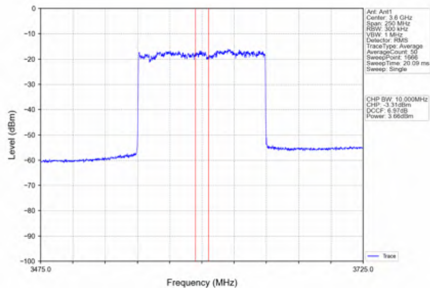
n78d_30kHz_SISO_NTNV_100MHz_CP-OFDM 64 QAM_3600MHz_Inner_Full
