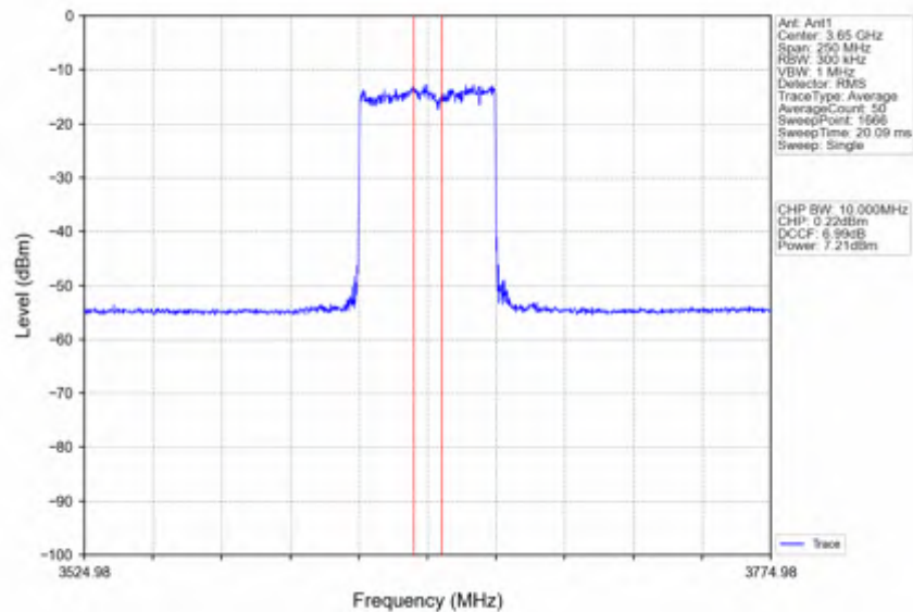
n78d_30kHz_SISO_NTNV_100MHz_CP-OFDM 256 QAM 3649.98MHz_Inner_Full
