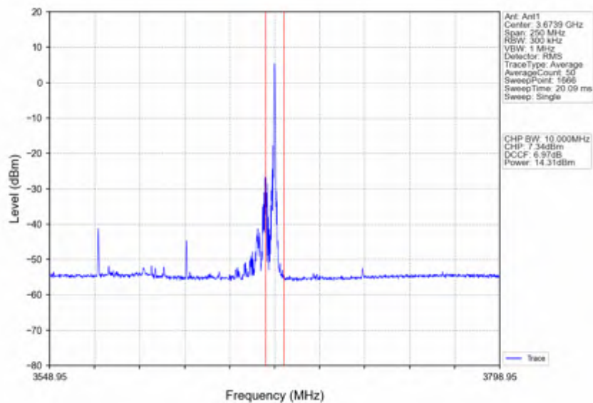
n78d_30kHz_SISO_NTNV_100MHz_CP-OFDM 16 QAM_3624.99MHz_Edge_1RB_Right
