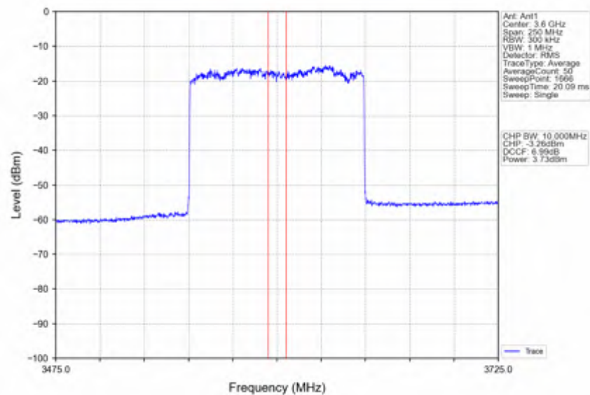
n78d 30kHz SISO NTNV 100MHz CP-OFDM 16 QAM 3600MHz Inner Full
