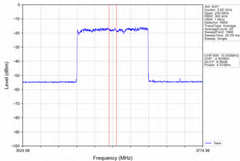
n78d_30kHz_SISO_NTNV_100MHz_CP-OFDM_64_QAM_3649.98MHz_Inner_Full
