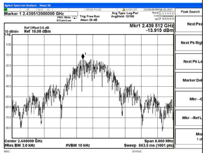
Channel 8 / 2440 MHz
