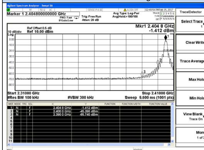
Channel 1 / 2405 MHz
