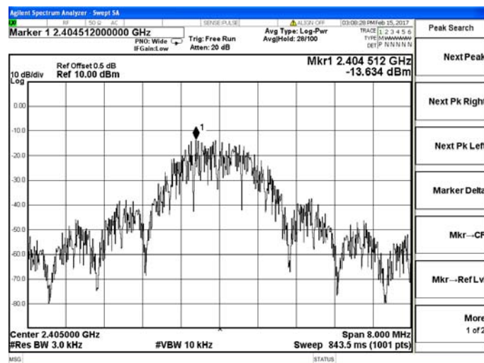
Channel 1 / 2405 MHz
