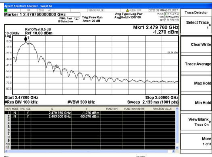
Channel 16 / 2480 MHz
