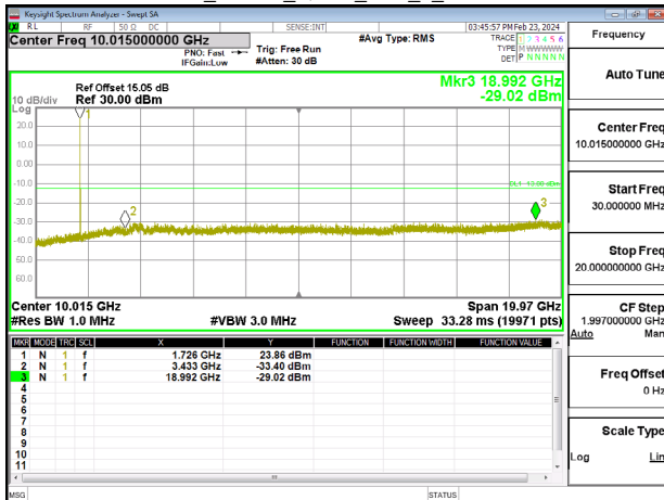
Band4_15MHz_QPSK_RB1_0_CH20175
