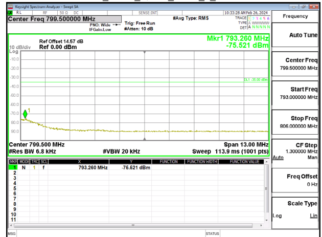
Band13_5MHz_QPSK_RB25_0_CH23255
