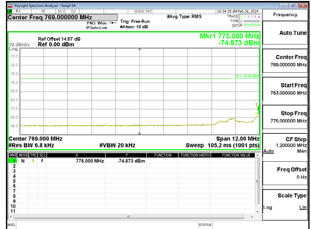
Band13_5MHz_QPSK_RB1_24_CH23255
