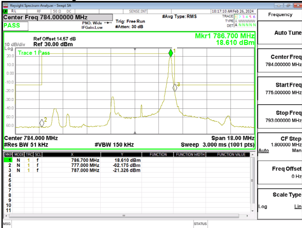
Band Edge_Band13_5MHz_QPSK_RB25_0_CH23205
