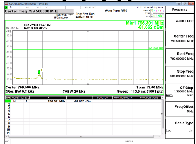
Band13_5MHz_QPSK_RB25_0_CH23205
