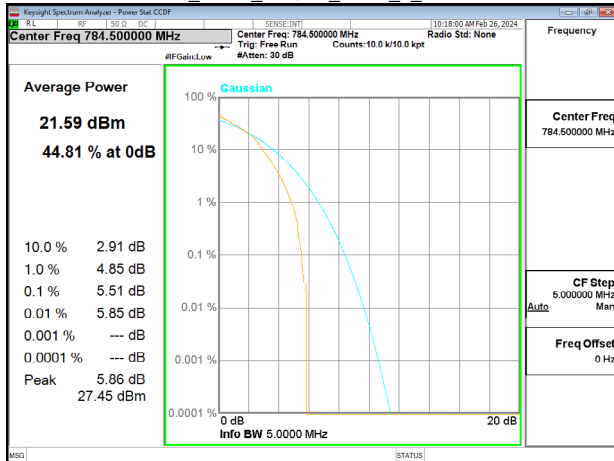
Band13_5MHz_16QAM_RB25_0_CH23255
