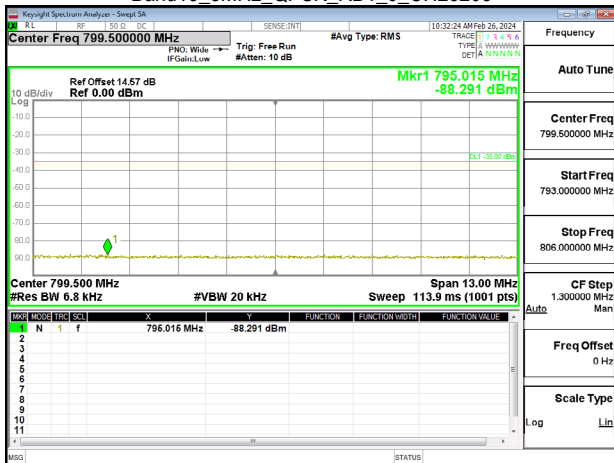
Band13_5MHz_QPSK_RB1_0_CH23205
