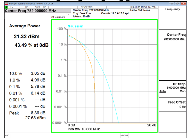
Band13_10MHz_16QAM_RB50_0_CH23230
