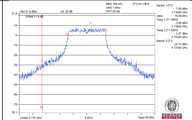
802.11ac(VHT20)_Chain1 / CH149
