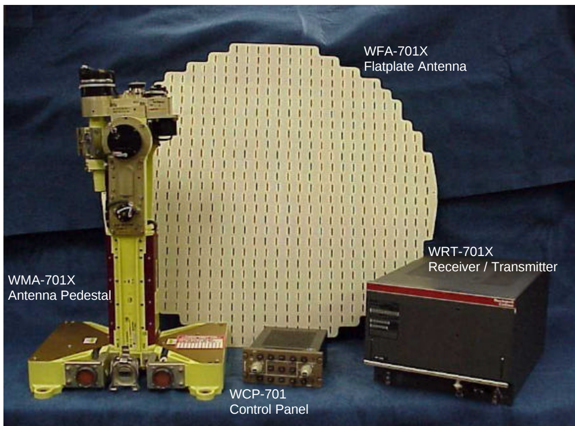
Figure C-1. WXR-701X Family
