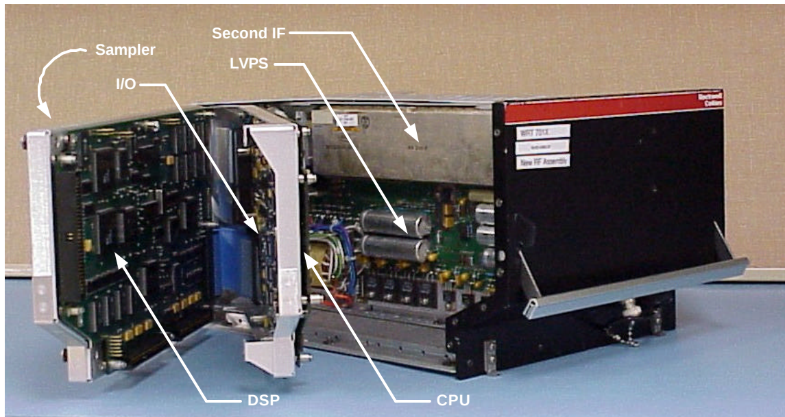
Figure C-7. WRT-701X Left Open
