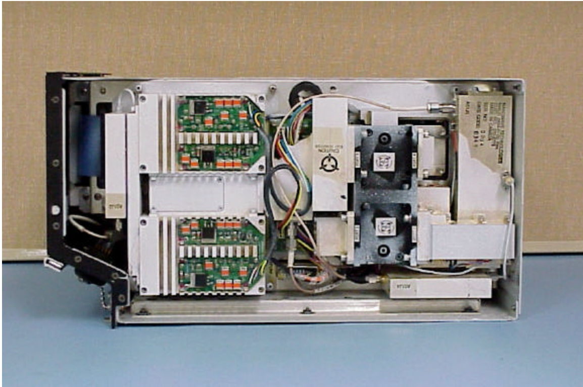
Figure C-4. WRT-701X Right Side
