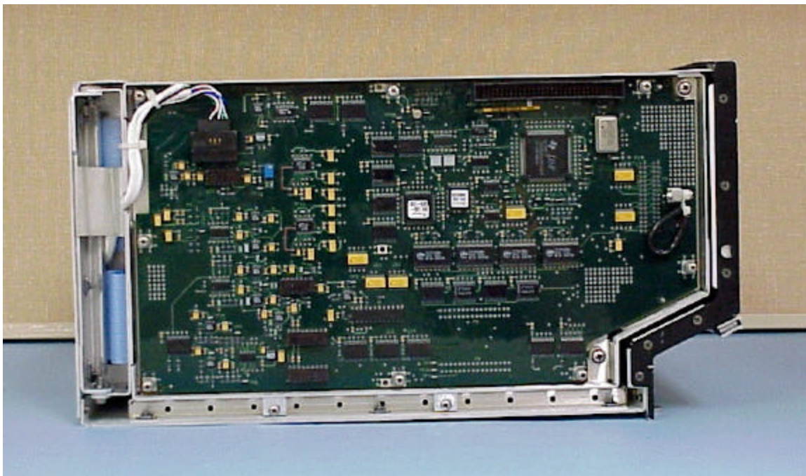
Figure C-5. WRT-701X Left Side
