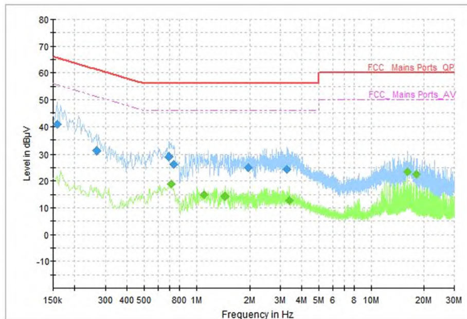
Fig.26 AC Power line Conducted Emission (Traffic)
