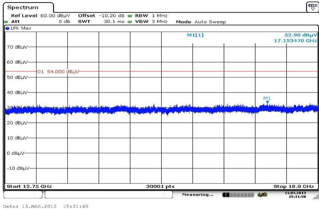
Plot 3: Middle channel, 12.75 GHz to 18 GHz, vertical & horizontal polarization
