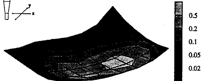
Fig. 8. Distribution of the SAR component normal to the probe axis in the shell phantom measured with a commercial mobile phone.
