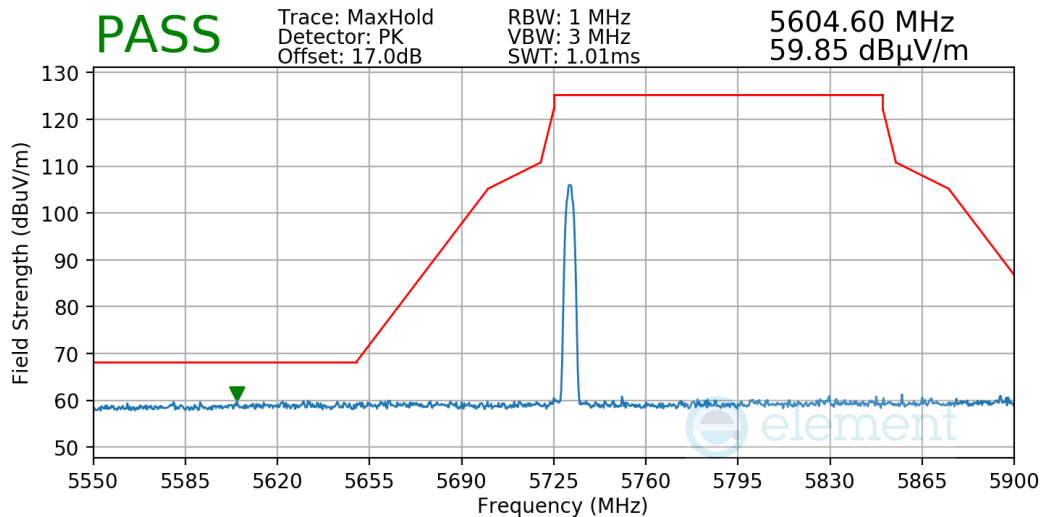
Plot 7-61. Radiated Lower Band Edge Measurement
