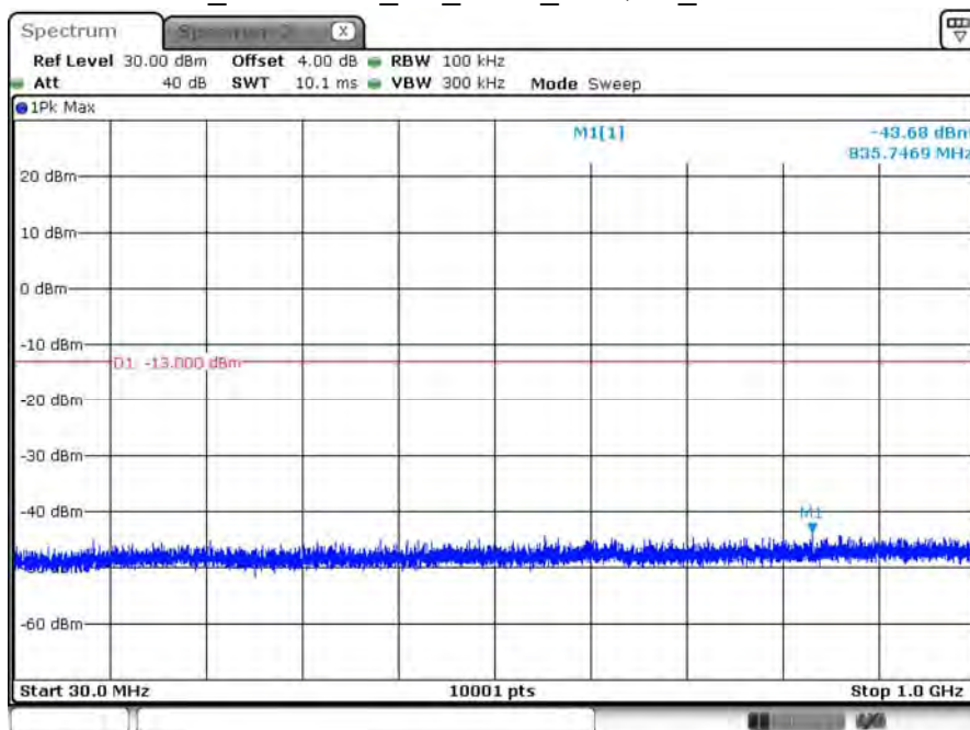
B66_CH132657_3M_1RB7_16-QAM_Below 1G
