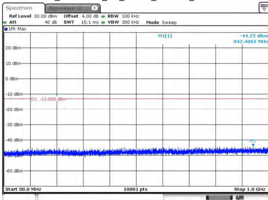
B66_CH132647_5M_1RB12_16-QAM_Below 1G
