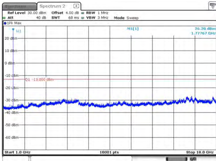
B66_CH132647_5M_1RB12_16-QAM_Above 1G
