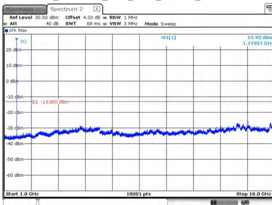
B66_CH132665_1.4M_1RB2_16-QAM_Above 1G
