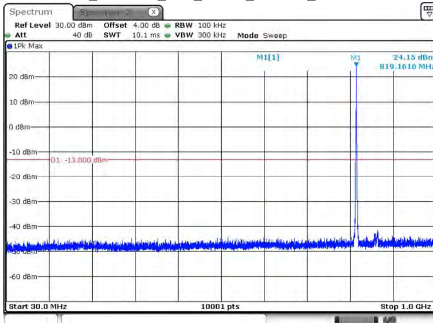
B26_CH26740_10M_1RB24_16-QAM_Below 1G
