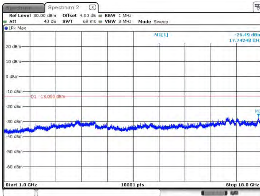
B26_CH26740_10M_1RB24_16-QAM_Above 1G
