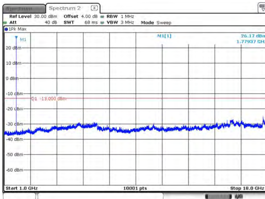
B66_CH132657_3M_1RB7_16-QAM_Above 1G
