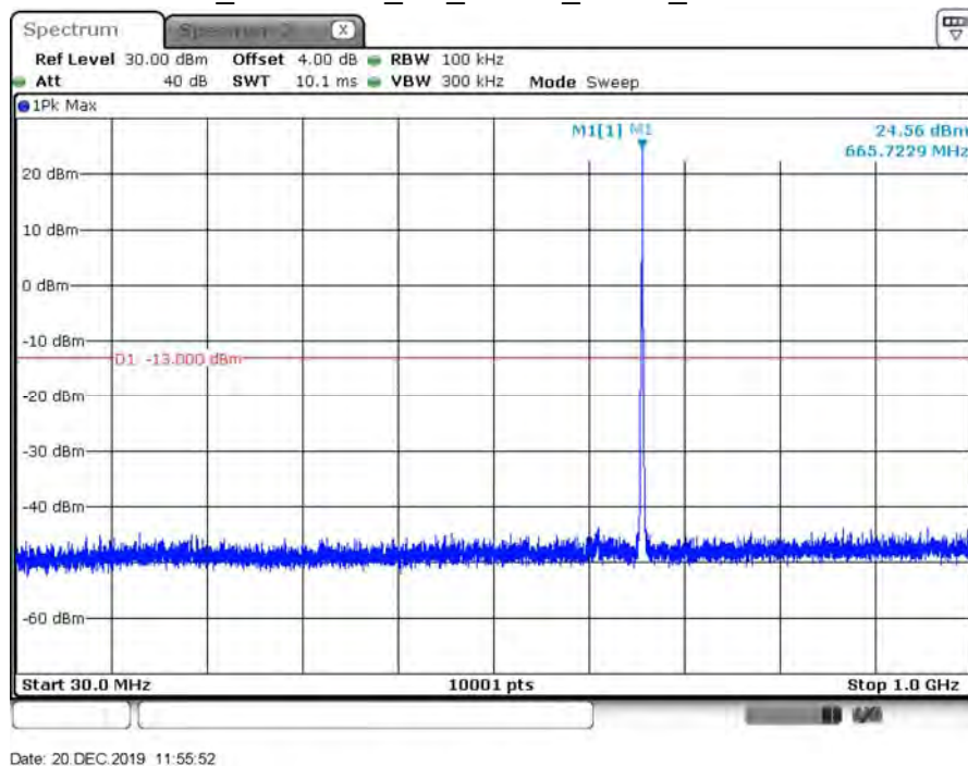
B71_CH113147_5M_1RB12_QPSK_Below 1G
