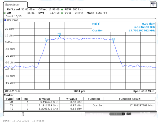
11AC20MIMO-Ant2-5200
