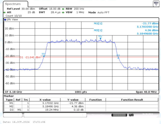
11N20MIMO-Ant2-5180
