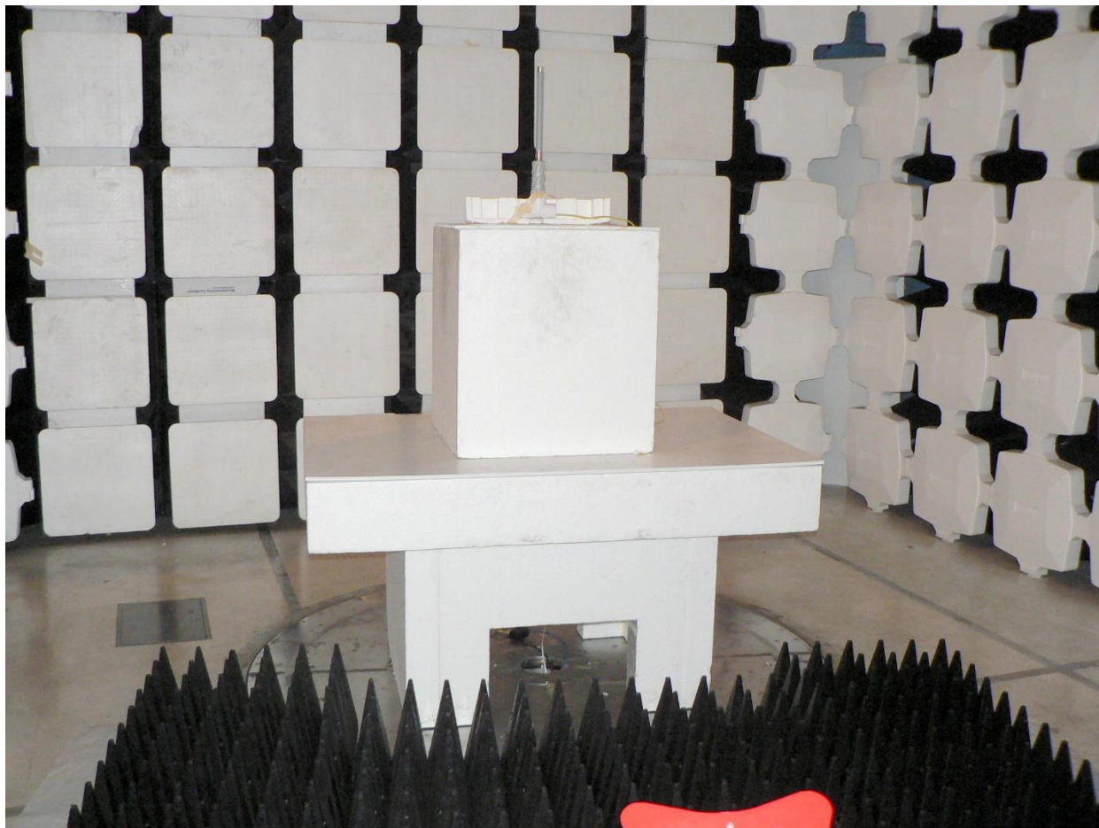
Tx Spurious
