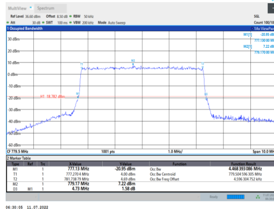
Band13-5MHz-16QAM-23205-25RB#0
