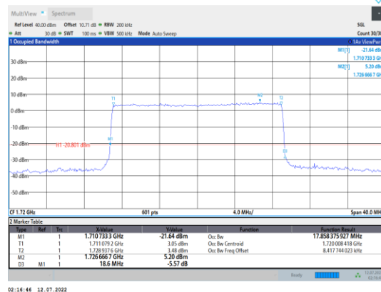
Band66-20MHz-16QAM-132072-100RB#0
