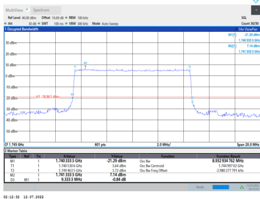
Band66-10MHz-QPSK-132322-50RB#0
