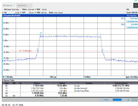
Band66-5MHz-QPSK-132322-25RB#0
