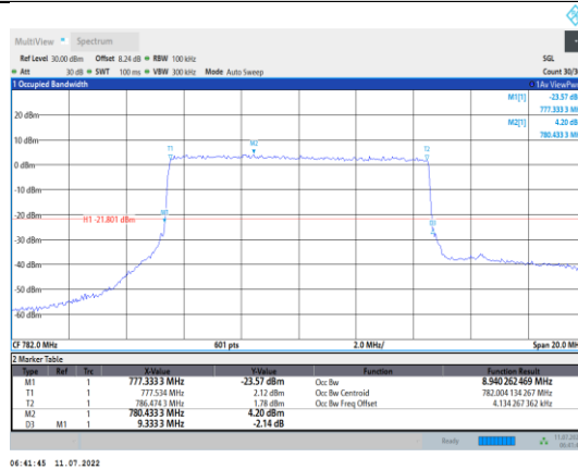
Band13-10MHz-16QAM-23230-50RB#0
