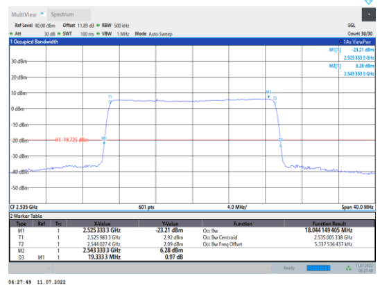
Band7-20MHz-16QAM-21100-100RB#0
