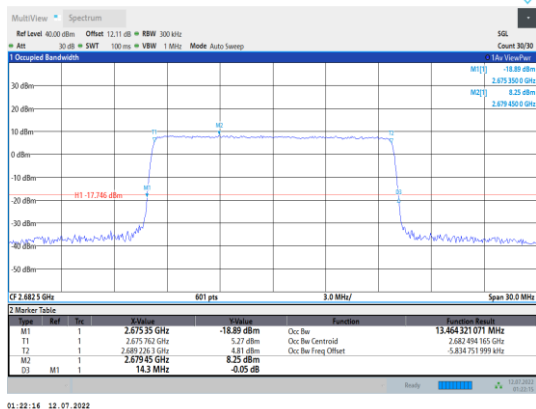
Band41-15MHz-QPSK-41515-75RB#0
