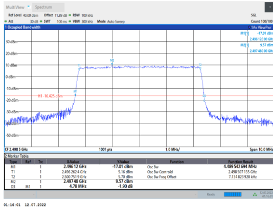
Band41-5MHz-QPSK-39675-25RB#0
