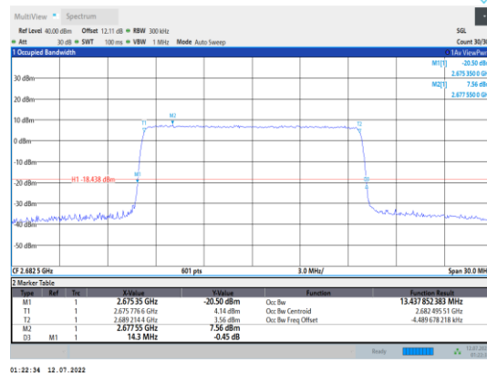
Band41-15MHz-16QAM-41515-75RB#0
