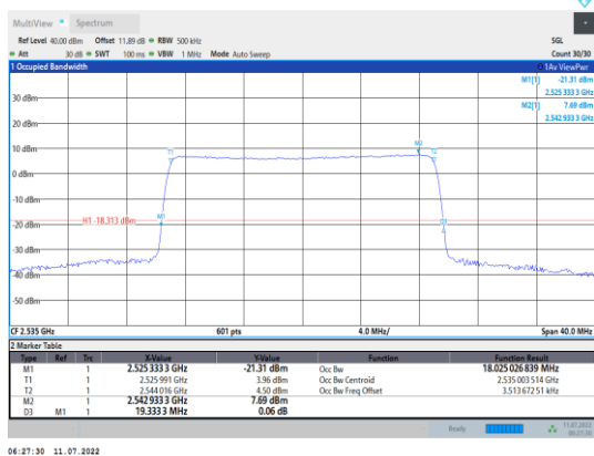
Band7-20MHz-QPSK-21100-100RB#0
