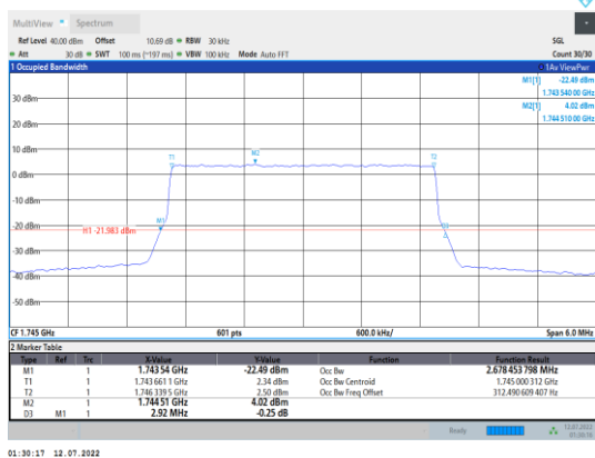
Band66-3MHz-QPSK-132322-15RB#0
