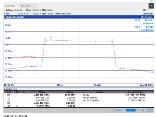
Band7-20MHz-16QAM-21350-100RB#0
