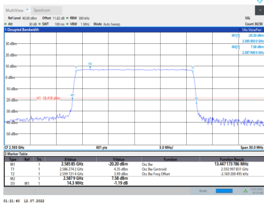
Band41-15MHz-QPSK-40620-75RB#0
