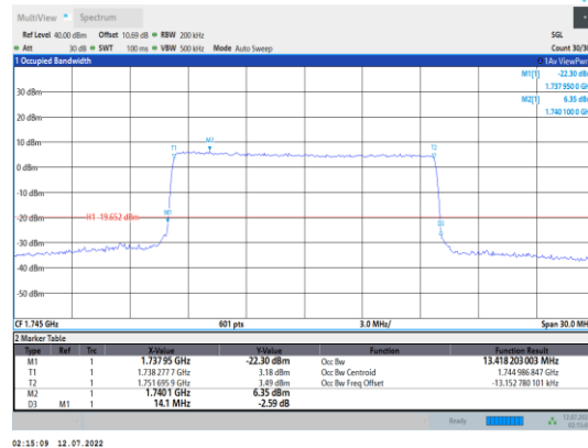
Band66-15MHz-16QAM-132322-75RB#0
