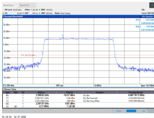
Band41-5MHz-QPSK-40620-25RB#0
