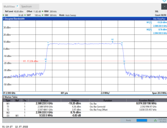
Band41-10MHz-QPSK-40620-50RB#0
