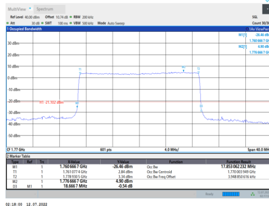
Band66-20MHz-16QAM-132572-100RB#0
