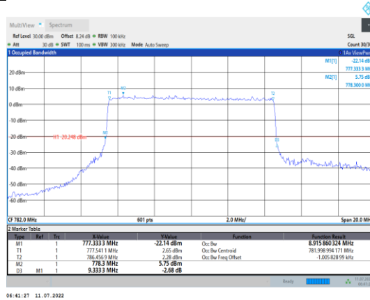
Band13-10MHz-QPSK-23230-50RB#0
