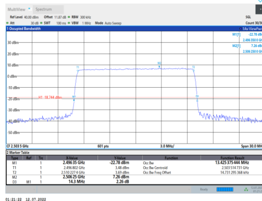
Band41-15MHz-16QAM-39725-75RB#0
