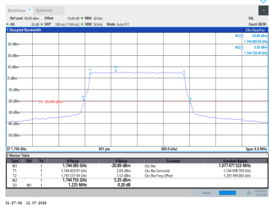
Band66-1.4MHz-16QAM-132322-6RB#0
