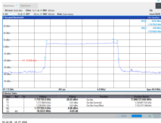
Band66-20MHz-QPSK-132072-100RB#0
