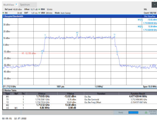
Band66-5MHz-QPSK-131997-25RB#0
