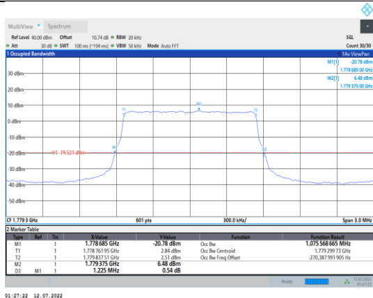
Band66-1.4MHz-QPSK-132665-6RB#0
