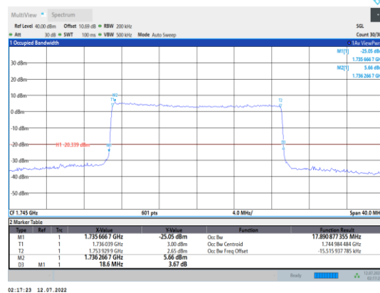
Band66-20MHz-16QAM-132322-100RB#0
