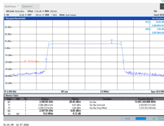
Band41-15MHz-16QAM-40620-75RB#0
