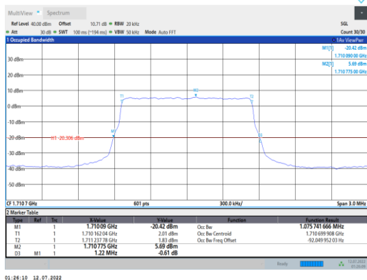
Band66-1.4MHz-QPSK-131979-6RB#0
