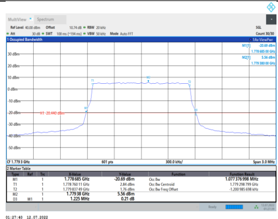
Band66-1.4MHz-16QAM-132665-6RB#0
