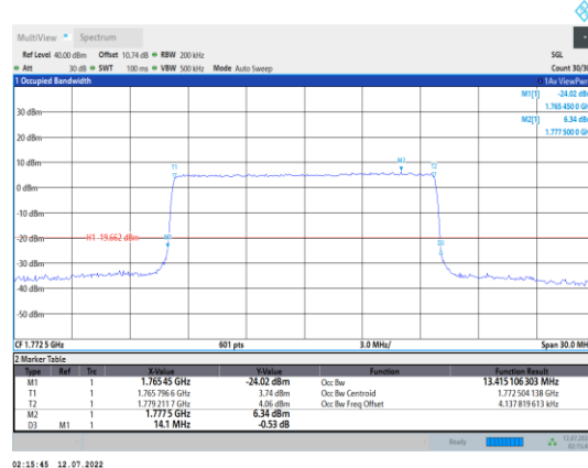
Band66-15MHz-16QAM-132597-75RB#0
