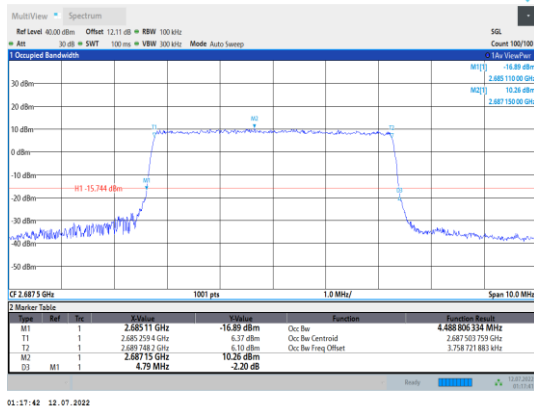
Band41-5MHz-QPSK-41565-25RB#0
