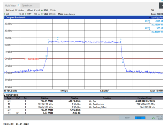
Band13-5MHz-16QAM-23255-25RB#0
