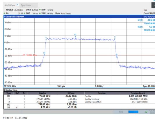
Band13-5MHz-16QAM-23230-25RB#0
