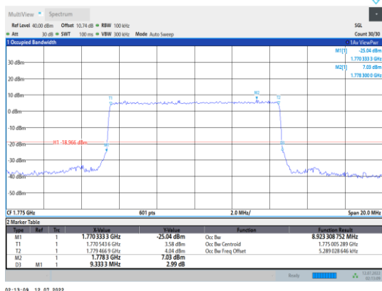
Band66-10MHz-QPSK-132622-50RB#0
