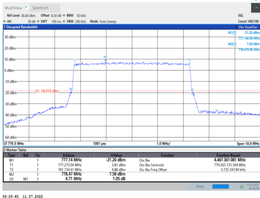
Band13-5MHz-QPSK-23205-25RB#0
