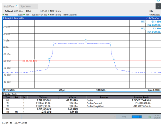
Band66-1.4MHz-QPSK-132322-6RB#0
