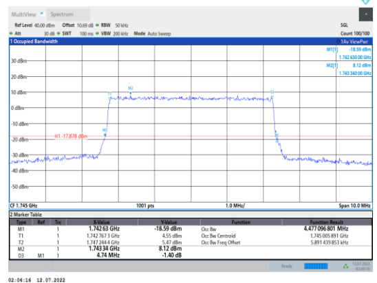
Band66-5MHz-16QAM-132322-25RB#0
