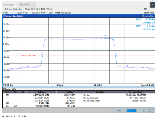
Band7-20MHz-QPSK-20850-100RB#0
