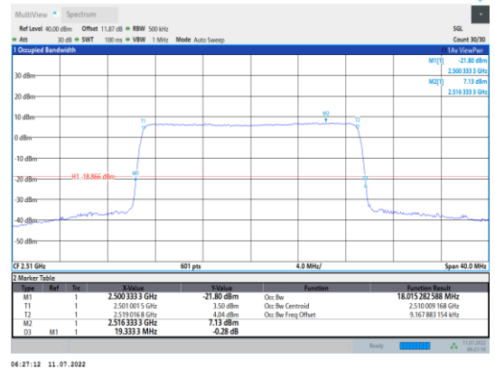
Band7-20MHz-16QAM-20850-100RB#0
