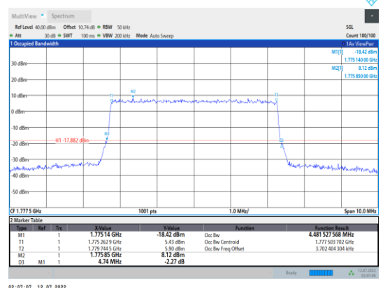
Band66-5MHz-16QAM-132647-25RB#0
