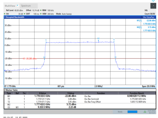
Band66-10MHz-16QAM-132622-50RB#0
