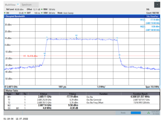
Band41-5MHz-16QAM-41565-25RB#0
