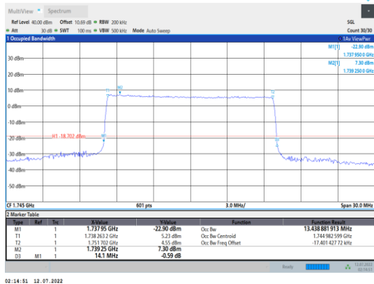
Band66-15MHz-QPSK-132322-75RB#0
