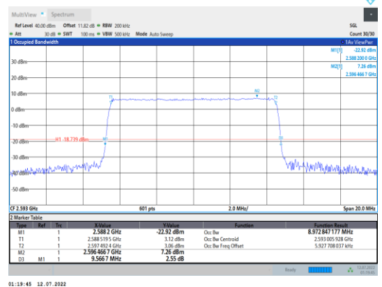
Band41-10MHz-16QAM-40620-50RB#0
