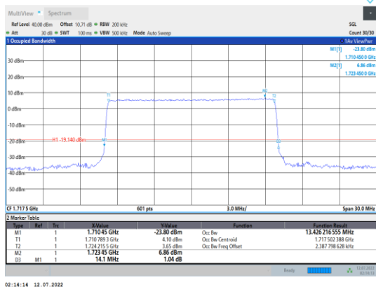
Band66-15MHz-QPSK-132047-75RB#0
