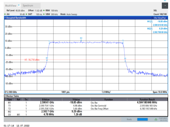
Band41-5MHz-16QAM-40620-25RB#0
