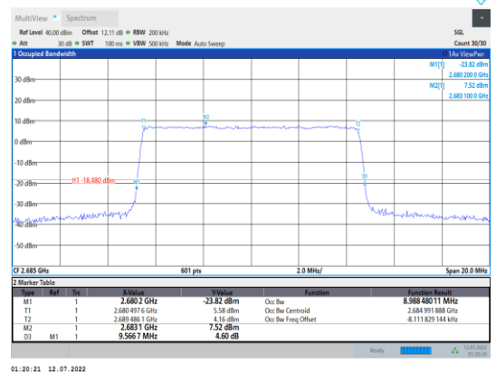
Band41-10MHz-16QAM-41540-50RB#0
