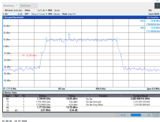
Band66-3MHz-QPSK-131987-15RB#0
