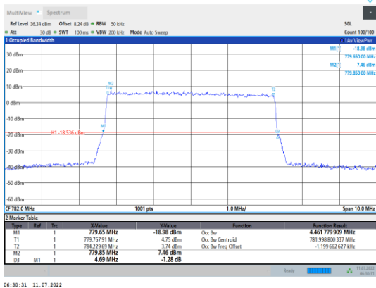
Band13-5MHz-QPSK-23230-25RB#0
