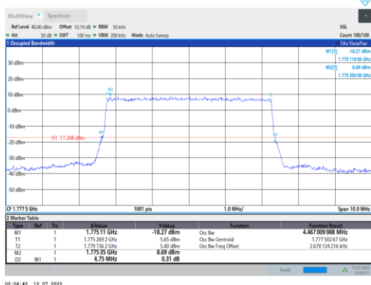
Band66-5MHz-QPSK-132647-25RB#0
