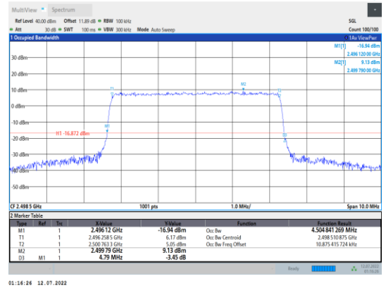
Band41-5MHz-16QAM-39675-25RB#0
