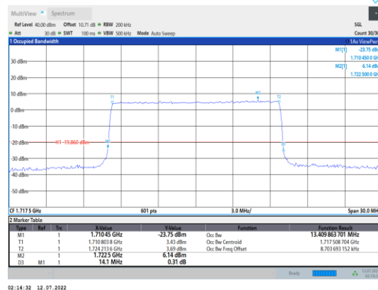
Band66-15MHz-16QAM-132047-75RB#0
