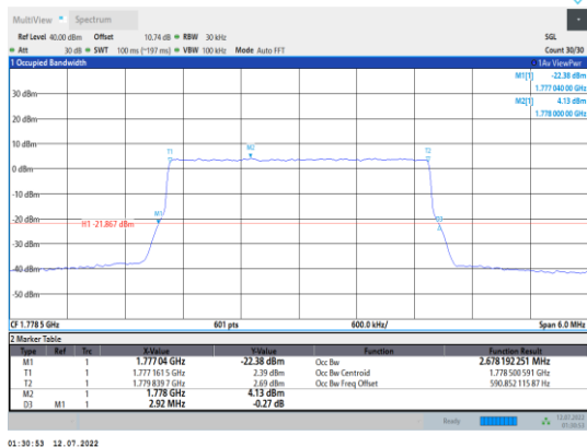
Band66-3MHz-QPSK-132657-15RB#0
