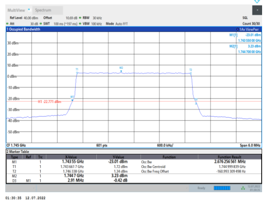
Band66-3MHz-16QAM-132322-15RB#0
