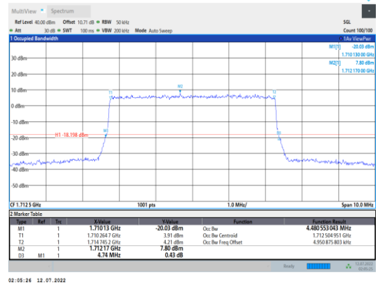
Band66-5MHz-16QAM-131997-25RB#0
