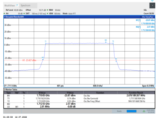
Band66-3MHz-16QAM-131987-15RB#0
