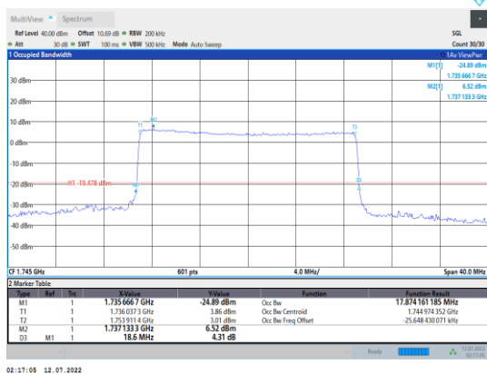
Band66-20MHz-QPSK-132322-100RB#0
