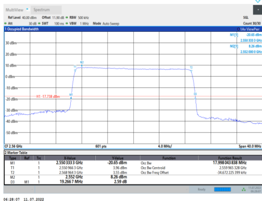
Band7-20MHz-QPSK-21350-100RB#0
