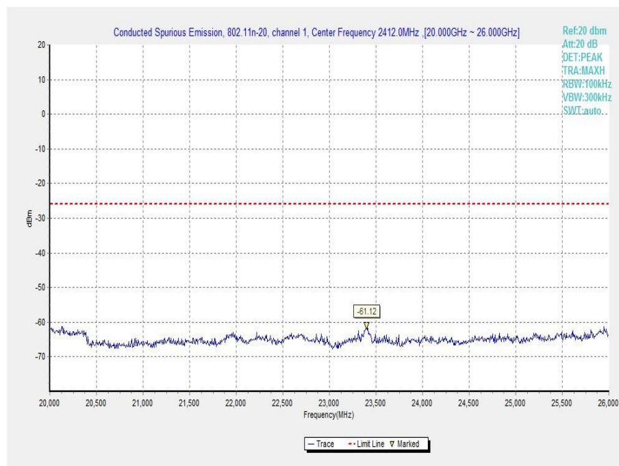
Fig.A.6.1.56 Transmitter Spurious Emission - Conducted (802.11n-HT20, Ch1, 20 GHz-26 GHz)
