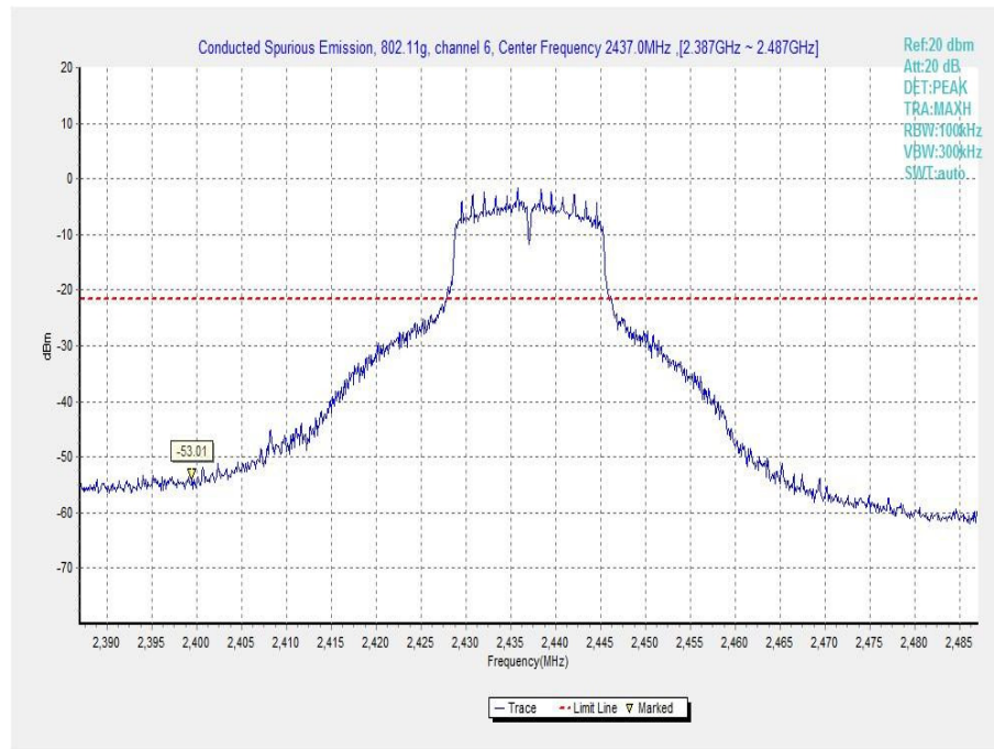
Fig.A.6.1.33 Transmitter Spurious Emission - Conducted (802.11g, Ch6, Center Frequency)
