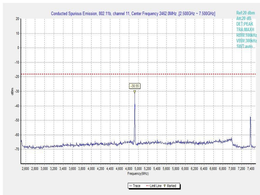
Fig.A.6.1.20 Transmitter Spurious Emission - Conducted (802.11b, Ch11, 2.5 GHz-7.5 GHz)
