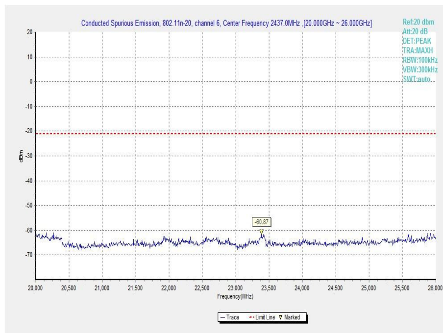
Fig.A.6.1.64 Transmitter Spurious Emission - Conducted (802.11n-HT20, Ch6, 20 GHz-26 GHz)
