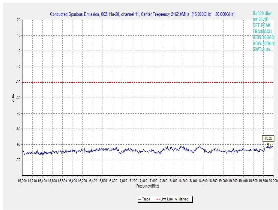
Fig.A.6.1.71 Transmitter Spurious Emission - Conducted (802.11n-HT20, Ch11, 15 GHz-20 GHz)
