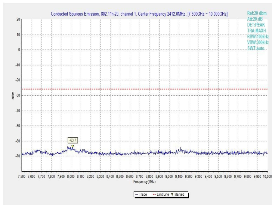
Fig.A.6.1.53 Transmitter Spurious Emission - Conducted (802.11n-HT20, Ch1, 7.5 GHz-10 GHz)
