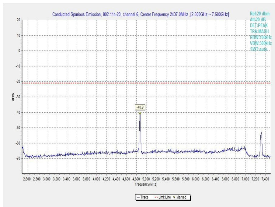
Fig.A.6.1.60 Transmitter Spurious Emission - Conducted (802.11n-HT20, Ch6, 2.5 GHz-7.5 GHz)
