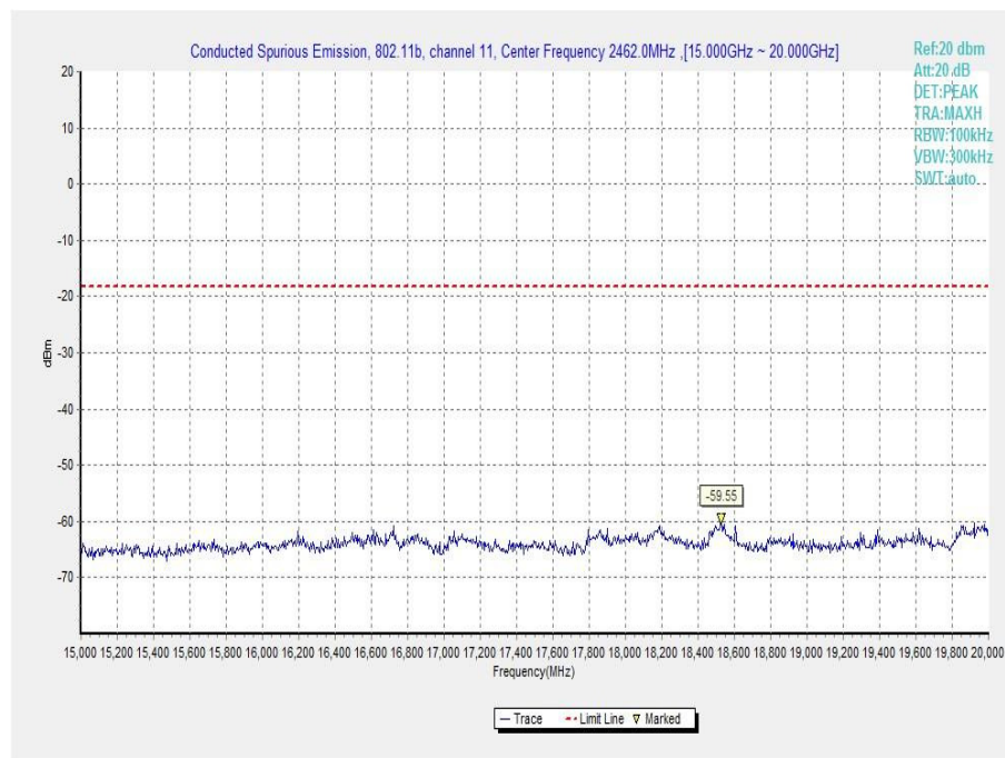
Fig.A.6.1.23 Transmitter Spurious Emission - Conducted (802.11b, Ch11, 15 GHz-20 GHz)
