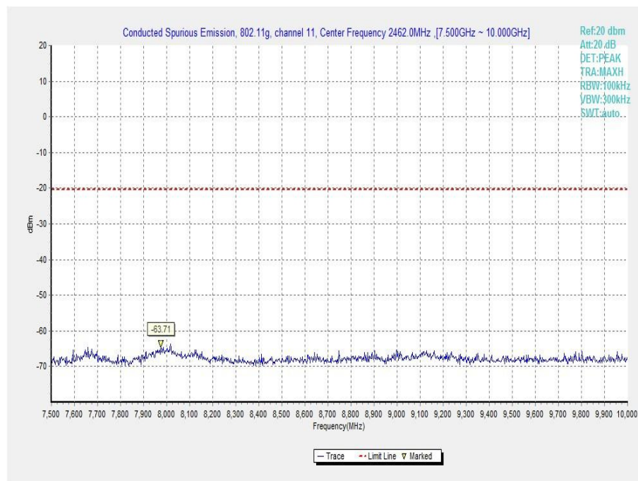
Fig.A.6.1.45 Transmitter Spurious Emission - Conducted (802.11g, Ch11, 7.5 GHz-10 GHz)
