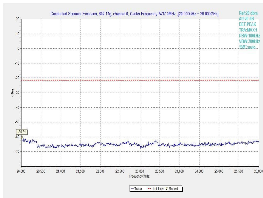
Fig.A.6.1.40 Transmitter Spurious Emission - Conducted (802.11g, Ch6, 20 GHz-26 GHz)
