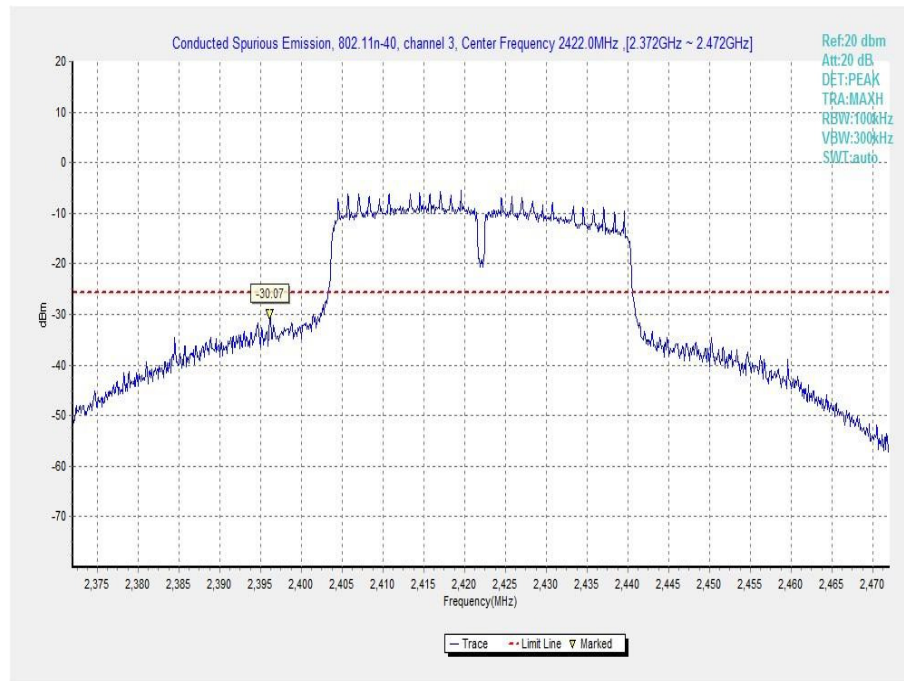
Fig.A.6.1.73 Transmitter Spurious Emission - Conducted (802.11n-HT40, Ch3, Center Frequency)
