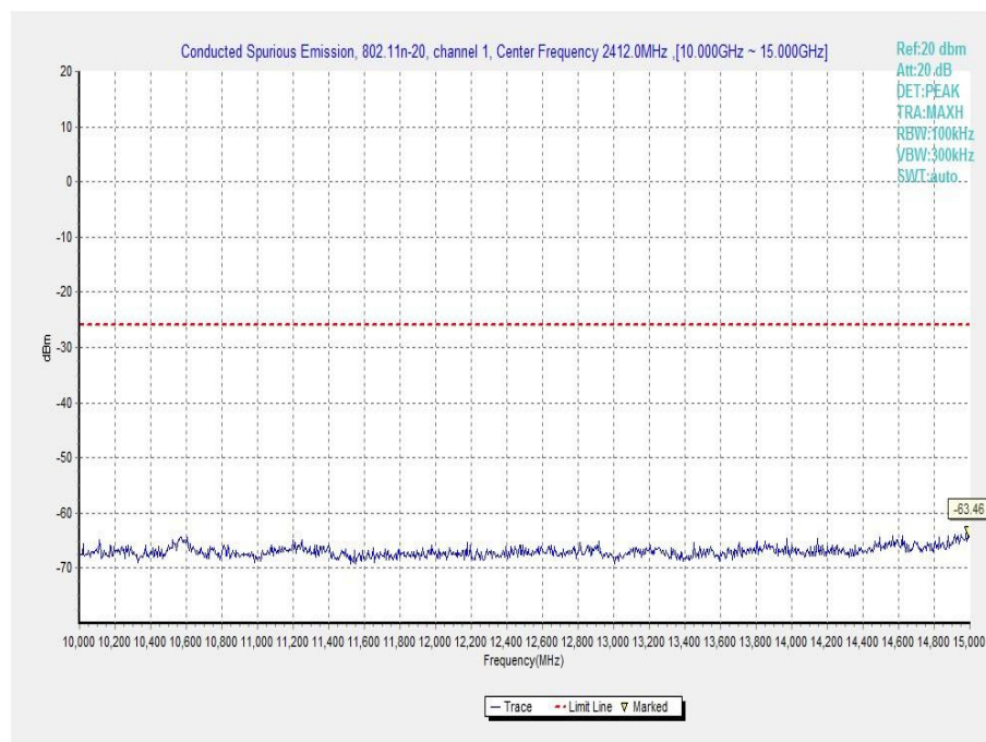
Fig.A.6.1.54 Transmitter Spurious Emission - Conducted (802.11n-HT20, Ch1, 10 GHz-15 GHz)
