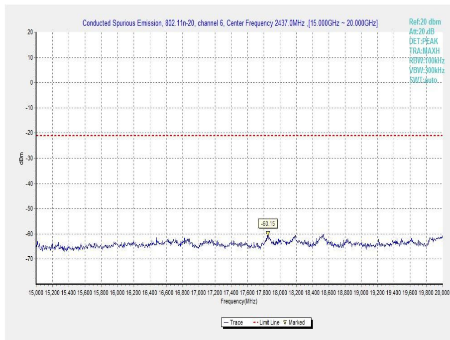
Fig.A.6.1.63 Transmitter Spurious Emission - Conducted (802.11n-HT20, Ch6, 15 GHz-20 GHz)
