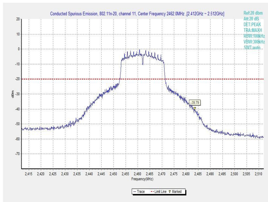
Fig.A.6.1.65 Transmitter Spurious Emission - Conducted (802.11n-HT20, Ch11, Center Frequency)
