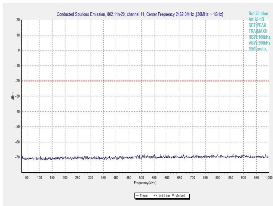
Fig.A.6.1.66 Transmitter Spurious Emission - Conducted (802.11n-HT20, Ch11, 30 MHz-1 GHz)
