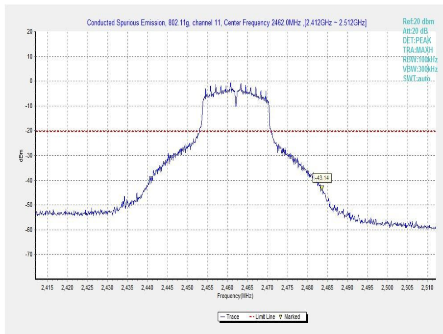
Fig.A.6.1.41 Transmitter Spurious Emission - Conducted (802.11g, Ch11, Center Frequency)
