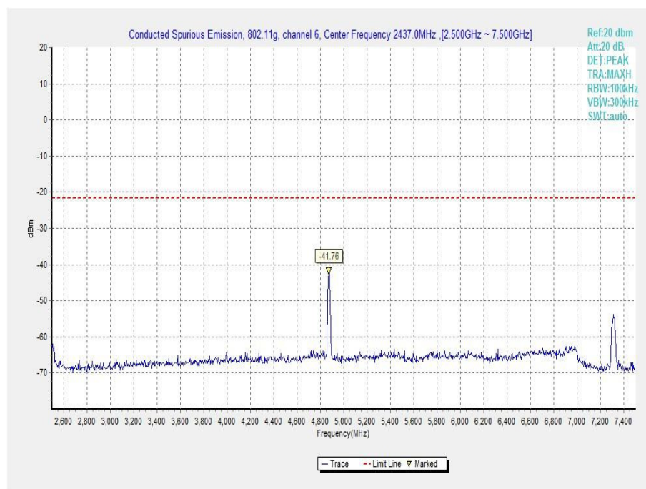
Fig.A.6.1.36 Transmitter Spurious Emission - Conducted (802.11g, Ch6, 2.5 GHz-7.5 GHz)
