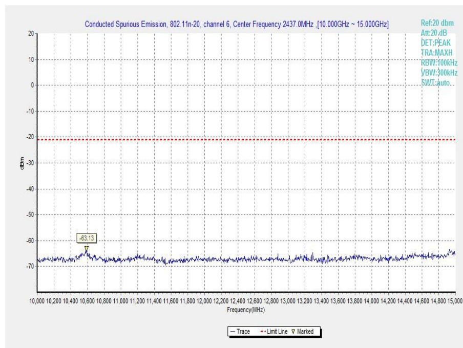
Fig.A.6.1.62 Transmitter Spurious Emission - Conducted (802.11n-HT20, Ch6, 10 GHz-15 GHz)
