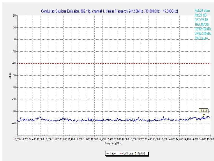
Fig.A.6.1.30 Transmitter Spurious Emission - Conducted (802.11g, Ch1, 10 GHz-15 GHz)
