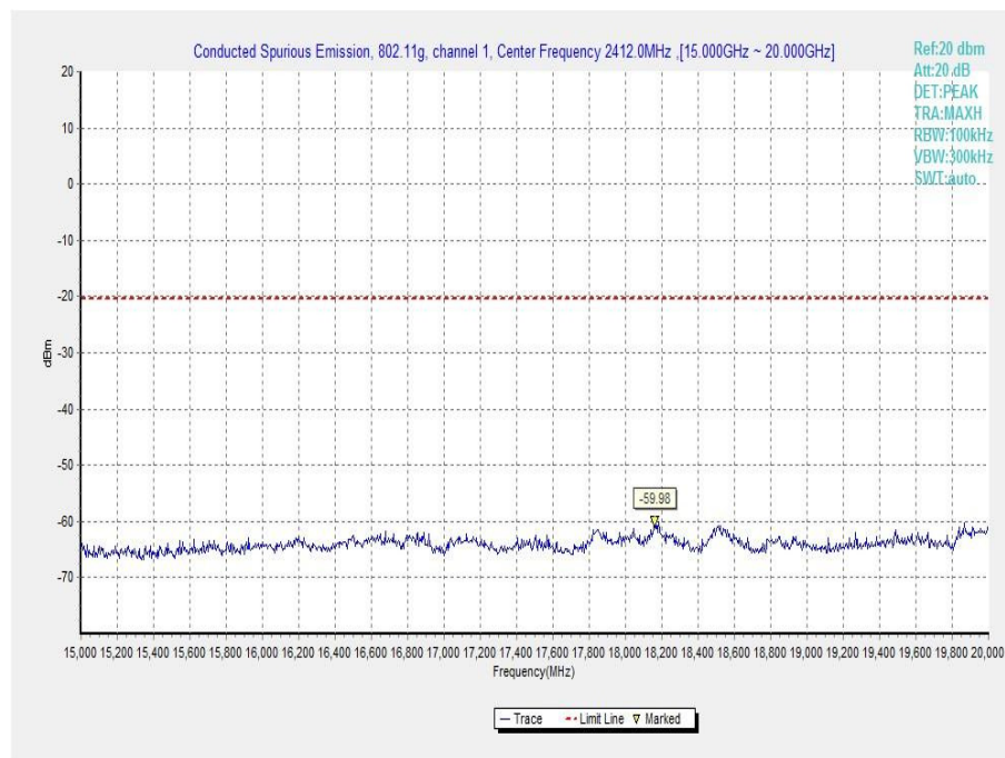
Fig.A.6.1.31 Transmitter Spurious Emission - Conducted (802.11g, Ch1, 15 GHz-20 GHz)
