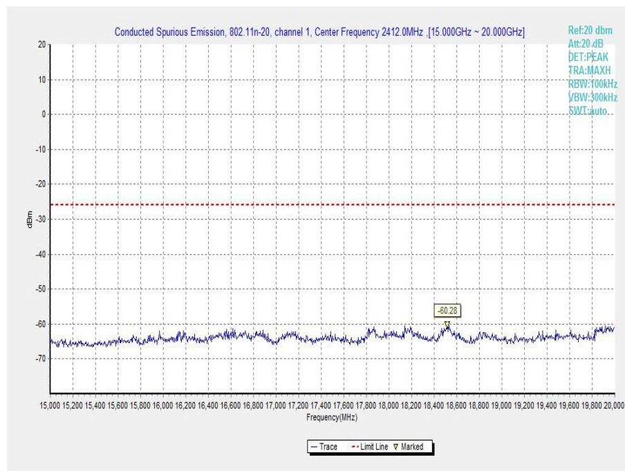
Fig.A.6.1.55 Transmitter Spurious Emission - Conducted (802.11n-HT20, Ch1, 15 GHz-20 GHz)
