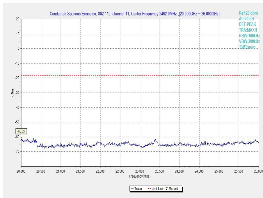
Fig.A.6.1.24 Transmitter Spurious Emission - Conducted (802.11b, Ch11, 20 GHz-26 GHz)
