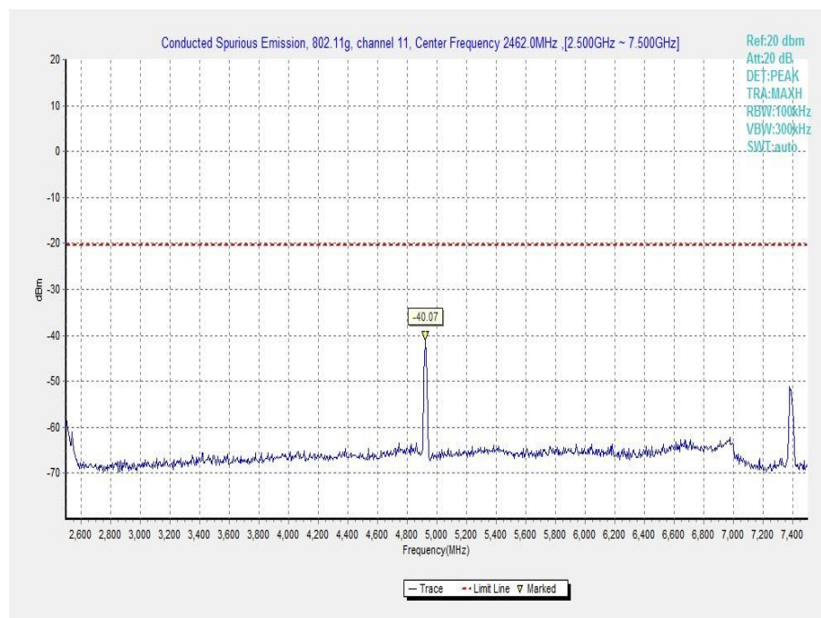
Fig.A.6.1.44 Transmitter Spurious Emission - Conducted (802.11g, Ch11, 2.5 GHz-7.5 GHz)
