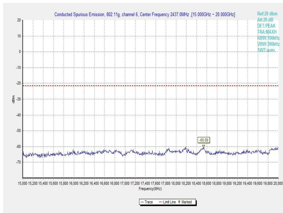
Fig.A.6.1.39 Transmitter Spurious Emission - Conducted (802.11g, Ch6, 15 GHz-20 GHz)
