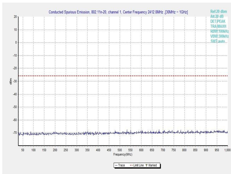
Fig.A.6.1.50 Transmitter Spurious Emission - Conducted (802.11n-HT20, Ch1, 30 MHz-1 GHz)
