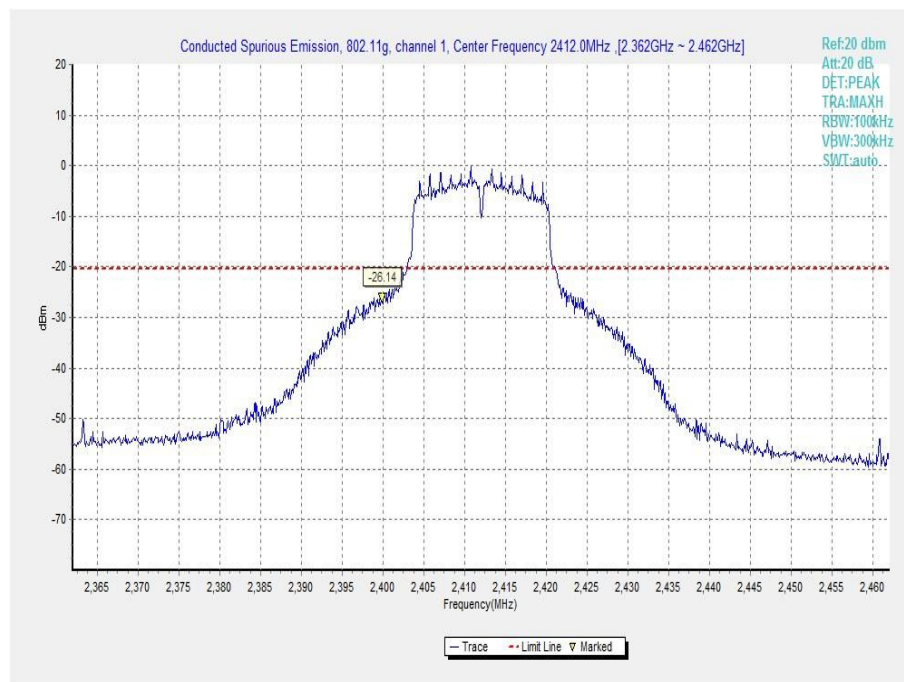
Fig.A.6.1.25 Transmitter Spurious Emission - Conducted (802.11g, Ch1, Center Frequency)
