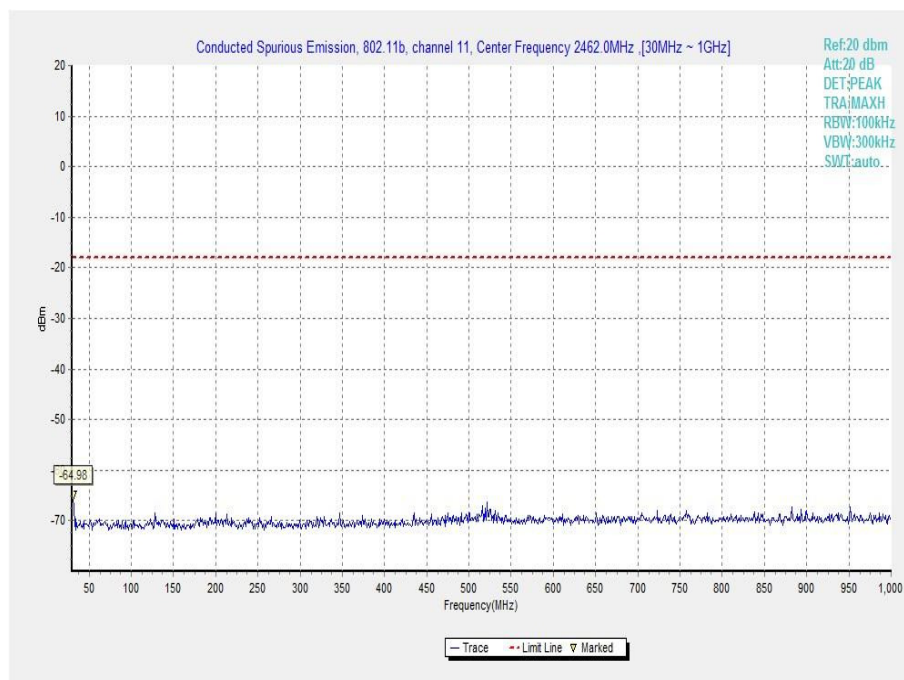
Fig.A.6.1.18 Transmitter Spurious Emission - Conducted (802.11b, Ch11, 30 MHz-1 GHz)
