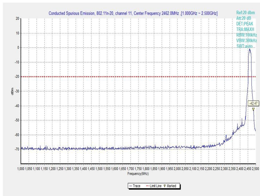
Fig.A.6.1.67 Transmitter Spurious Emission - Conducted (802.11n-HT20, Ch11, 1 GHz-2.5 GHz)
