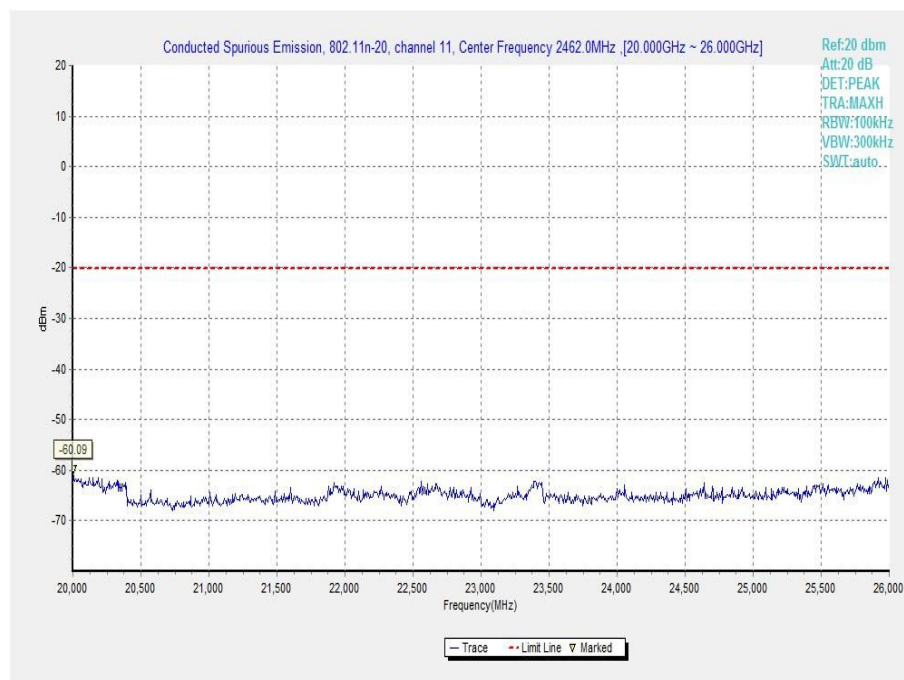
Fig.A.6.1.72 Transmitter Spurious Emission - Conducted (802.11n-HT20, Ch11, 20 GHz-26 GHz)
