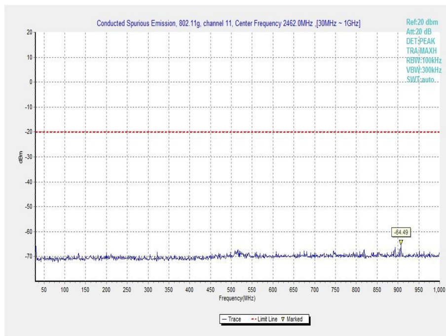
Fig.A.6.1.42 Transmitter Spurious Emission - Conducted (802.11g, Ch11, 30 MHz-1 GHz)
