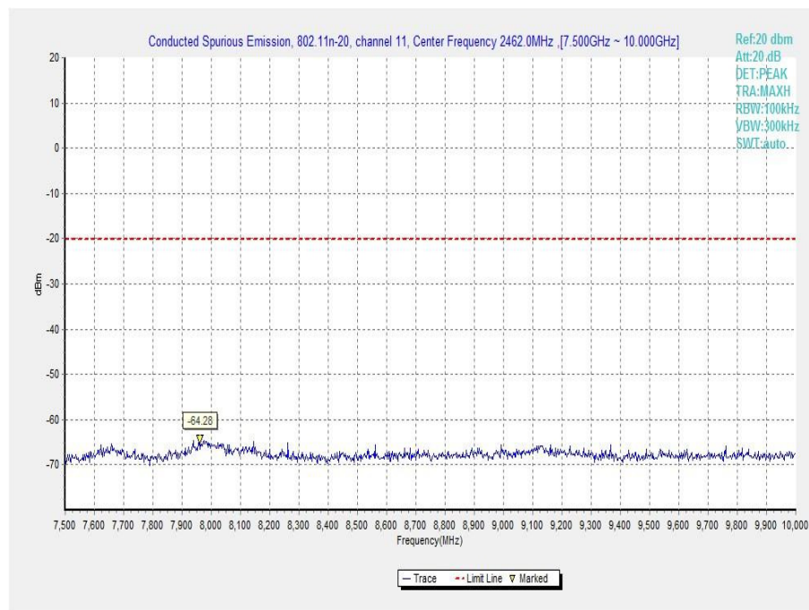
Fig.A.6.1.69 Transmitter Spurious Emission - Conducted (802.11n-HT20, Ch11, 7.5 GHz-10 GHz)
