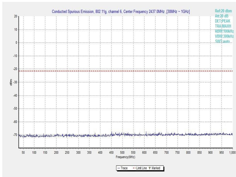
Fig.A.6.1.34 Transmitter Spurious Emission - Conducted (802.11g, Ch6, 30 MHz-1 GHz)
