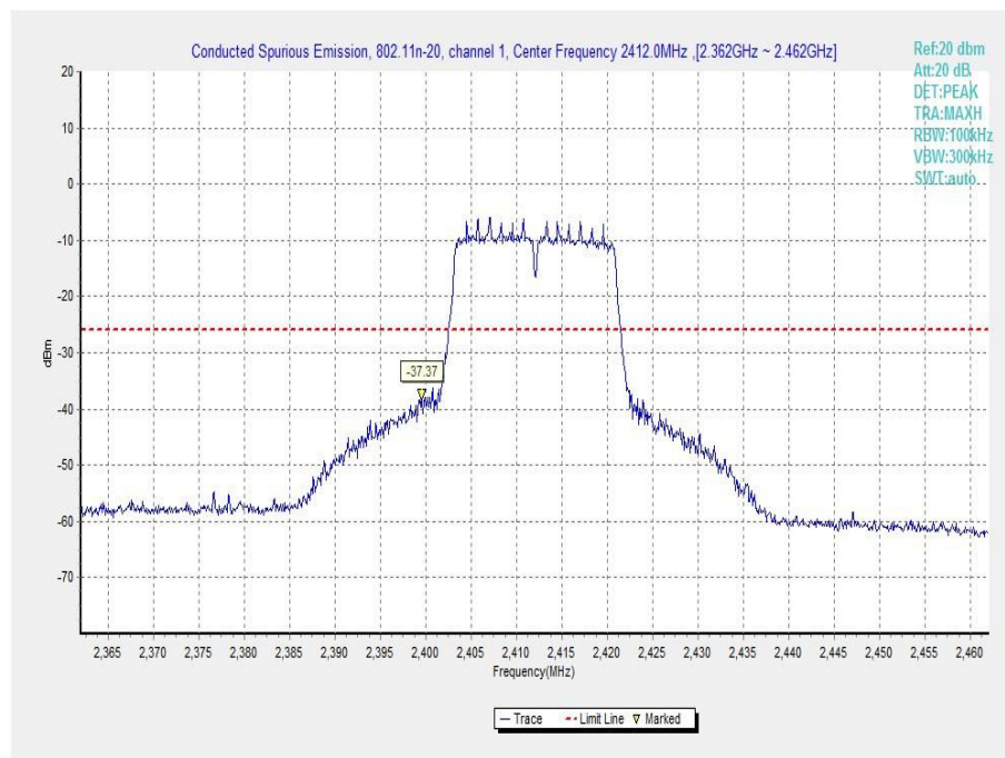
Fig.A.6.1.49 Transmitter Spurious Emission - Conducted (802.11n-HT20, Ch1, Center Frequency)
