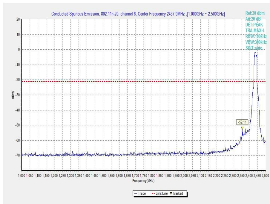
Fig.A.6.1.59 Transmitter Spurious Emission - Conducted (802.11n-HT20, Ch6, 1 GHz-2.5 GHz)
