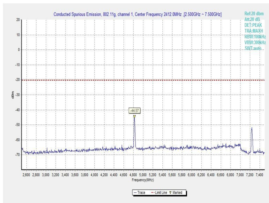
Fig.A.6.1.28 Transmitter Spurious Emission - Conducted (802.11g, Ch1, 2.5 GHz-7.5 GHz)
