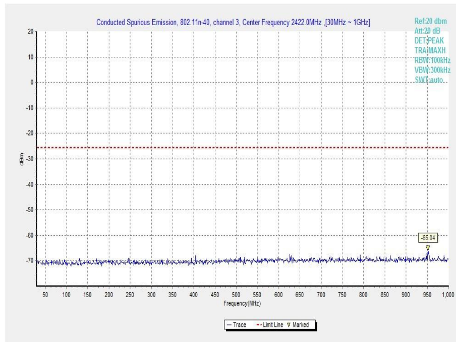
Fig.A.6.1.74 Transmitter Spurious Emission - Conducted (802.11n-HT40, Ch3, 30 MHz-1 GHz)
