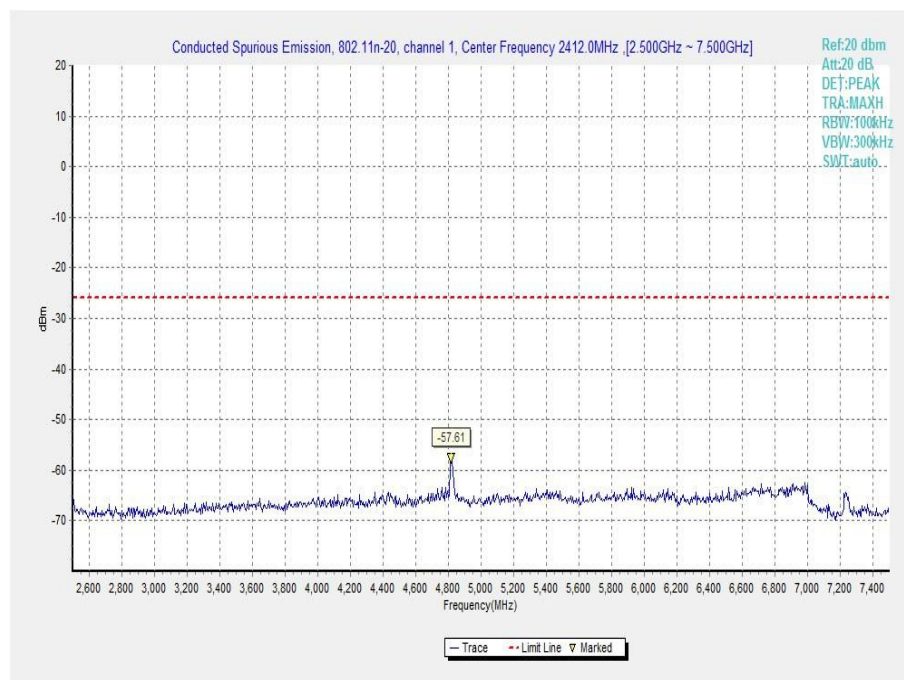
Fig.A.6.1.52 Transmitter Spurious Emission - Conducted (802.11n-HT20, Ch1, 2.5 GHz-7.5 GHz)
