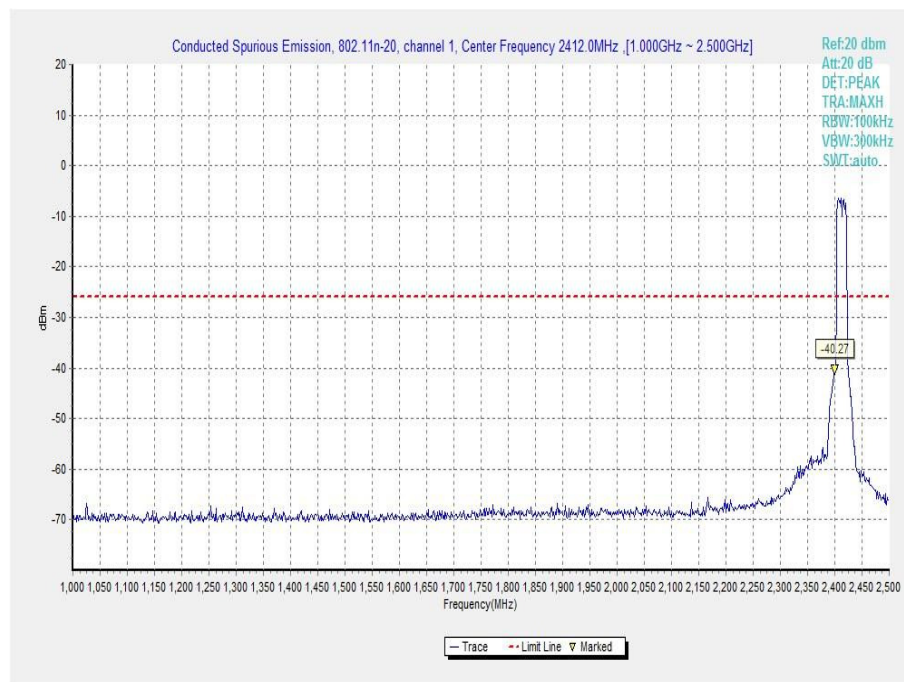
Fig.A.6.1.51 Transmitter Spurious Emission - Conducted (802.11n-HT20, Ch1, 1 GHz-2.5 GHz)
