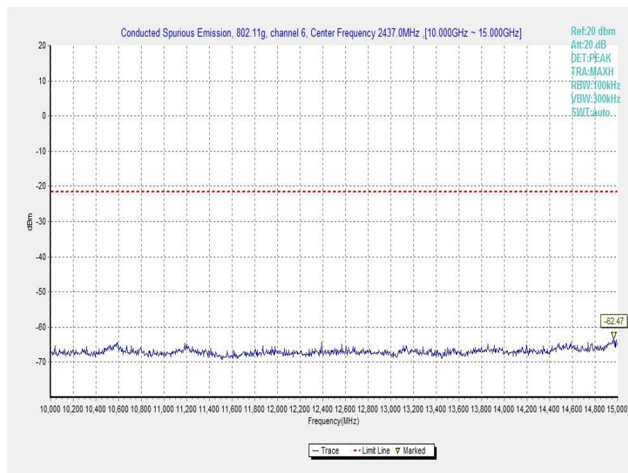
Fig.A.6.1.38 Transmitter Spurious Emission - Conducted (802.11g, Ch6, 10 GHz-15 GHz)
