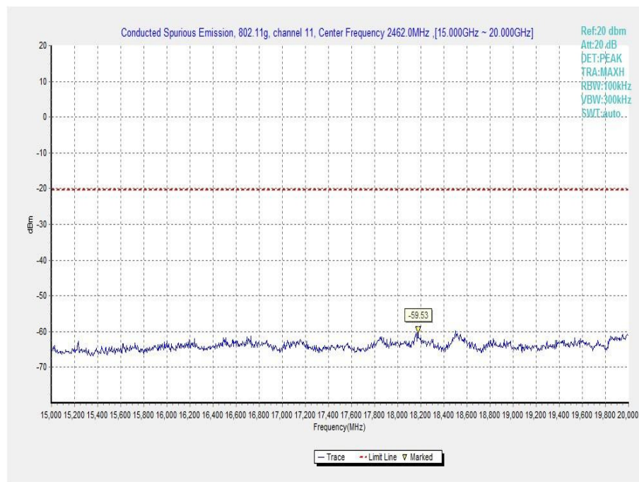
Fig.A.6.1.47 Transmitter Spurious Emission - Conducted (802.11g, Ch11, 15 GHz-20 GHz)
