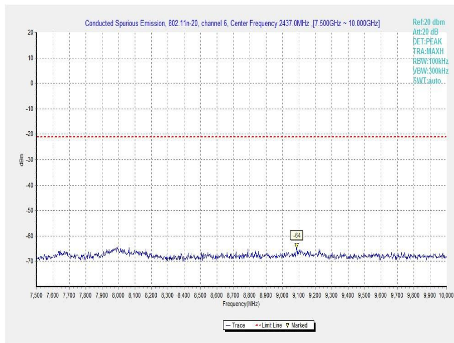
Fig.A.6.1.61 Transmitter Spurious Emission - Conducted (802.11n-HT20, Ch6, 7.5 GHz-10 GHz)
