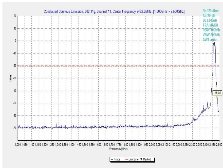
Fig.A.6.1.43 Transmitter Spurious Emission - Conducted (802.11g, Ch11, 1 GHz-2.5 GHz)
