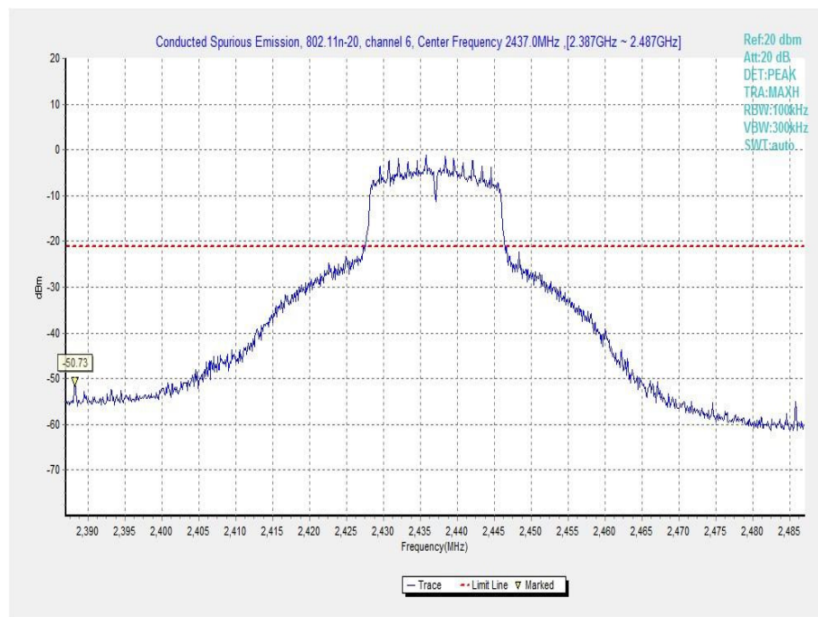
Fig.A.6.1.57 Transmitter Spurious Emission - Conducted (802.11n-HT20, Ch6, Center Frequency)
