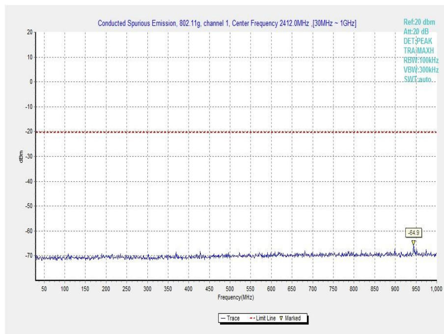
Fig.A.6.1.26 Transmitter Spurious Emission - Conducted (802.11g, Ch1, 30 MHz-1 GHz)
