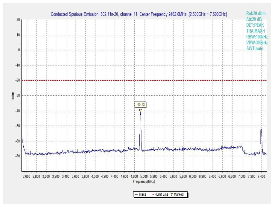
Fig.A.6.1.68 Transmitter Spurious Emission - Conducted (802.11n-HT20, Ch11, 2.5 GHz-7.5 GHz)
