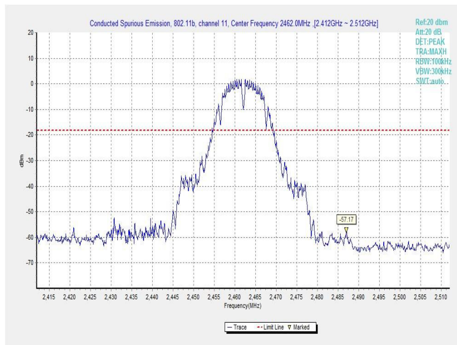
Fig.A.6.1.17 Transmitter Spurious Emission - Conducted (802.11b, Ch11, Center Frequency)
