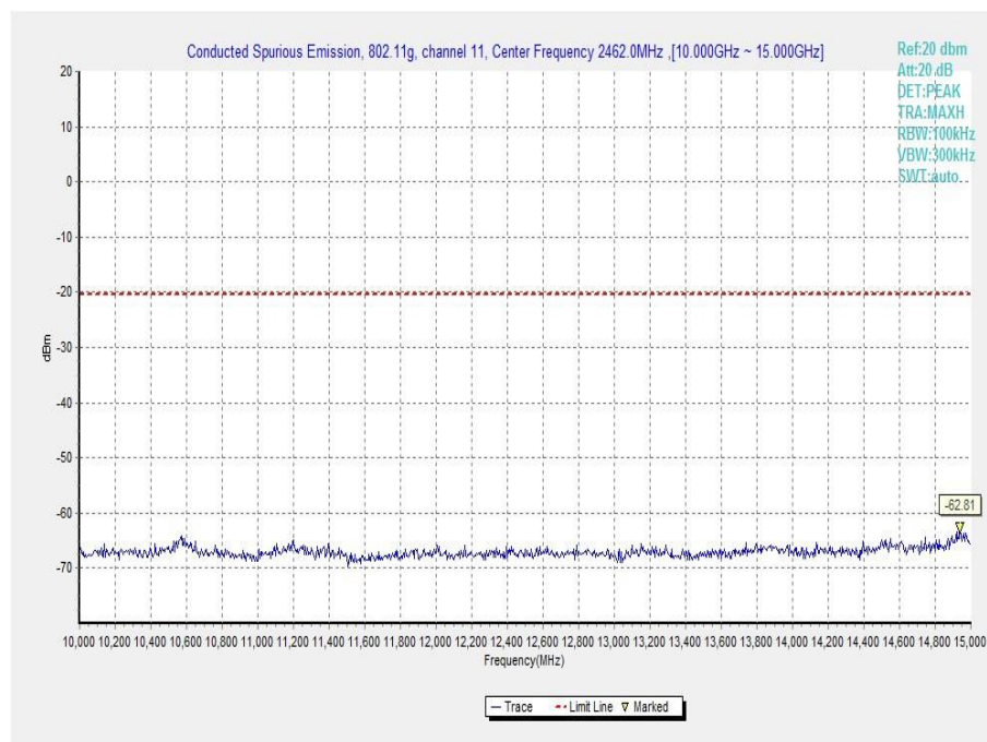
Fig.A.6.1.46 Transmitter Spurious Emission - Conducted (802.11g, Ch11, 10 GHz-15 GHz)
