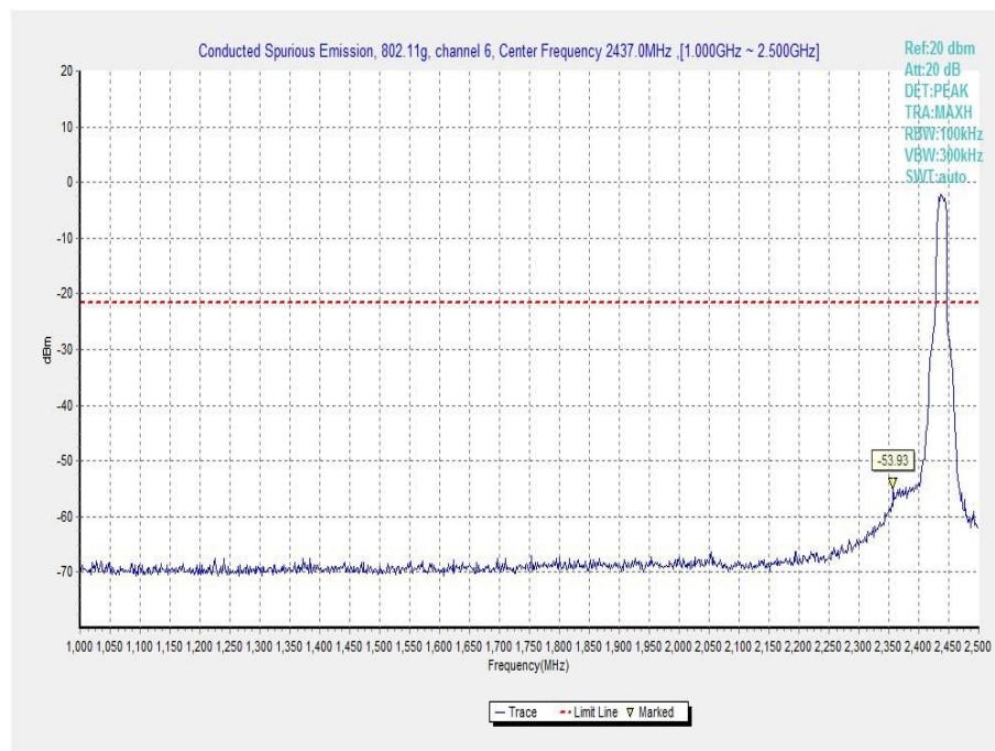
Fig.A.6.1.35 Transmitter Spurious Emission - Conducted (802.11g, Ch6, 1 GHz-2.5 GHz)
