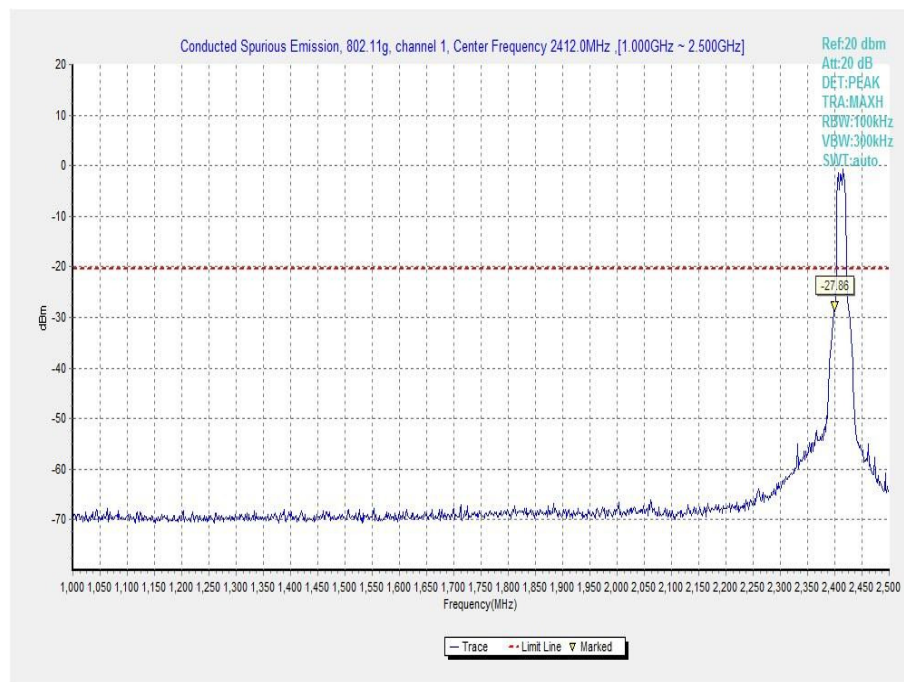
Fig.A.6.1.27 Transmitter Spurious Emission - Conducted (802.11g, Ch1, 1 GHz-2.5 GHz)
