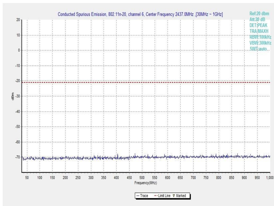
Fig.A.6.1.58 Transmitter Spurious Emission - Conducted (802.11n-HT20, Ch6, 30 MHz-1 GHz)
