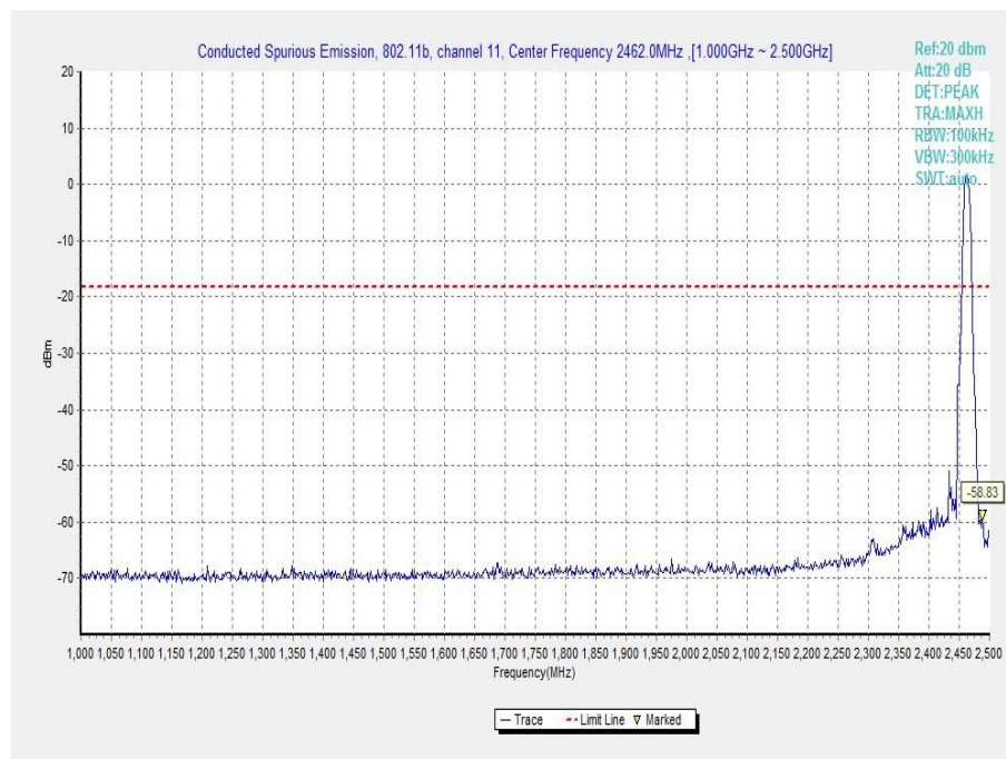
Fig.A.6.1.19 Transmitter Spurious Emission - Conducted (802.11b, Ch11, 1 GHz-2.5 GHz)
