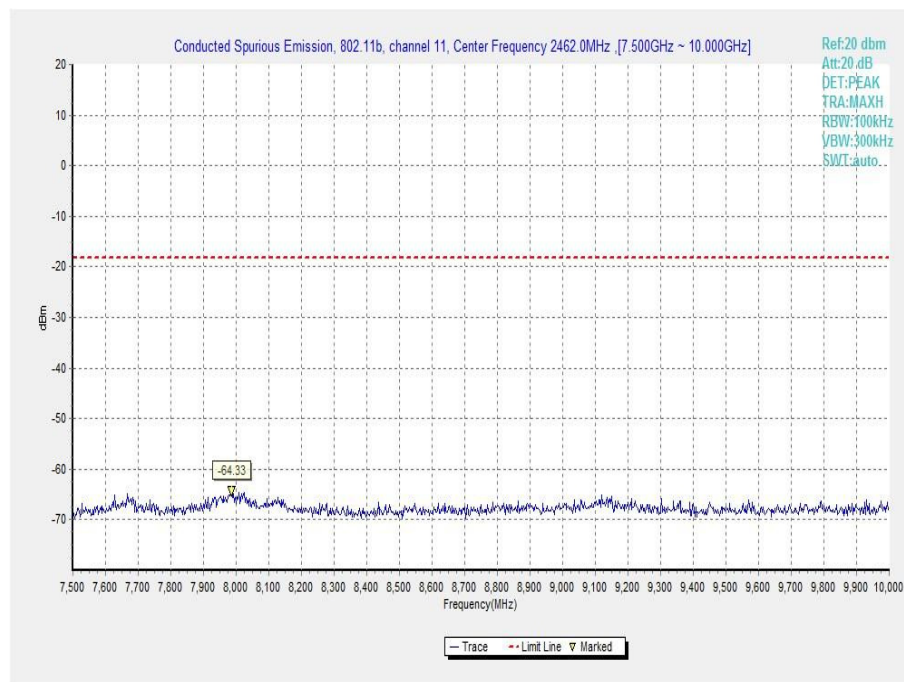
Fig.A.6.1.21 Transmitter Spurious Emission - Conducted (802.11b, Ch11, 7.5 GHz-10 GHz)
