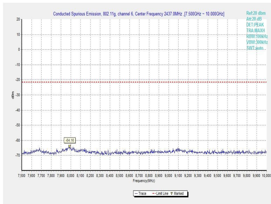
Fig.A.6.1.37 Transmitter Spurious Emission - Conducted (802.11g, Ch6, 7.5 GHz-10 GHz)
