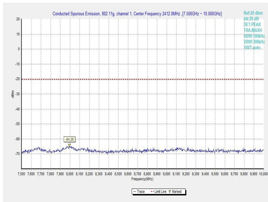
Fig.A.6.1.29 Transmitter Spurious Emission - Conducted (802.11g, Ch1, 7.5 GHz-10 GHz)
