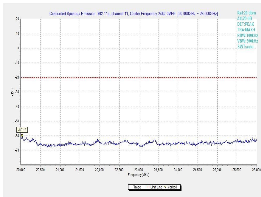
Fig.A.6.1.48 Transmitter Spurious Emission - Conducted (802.11g, Ch11, 20 GHz-26 GHz)
