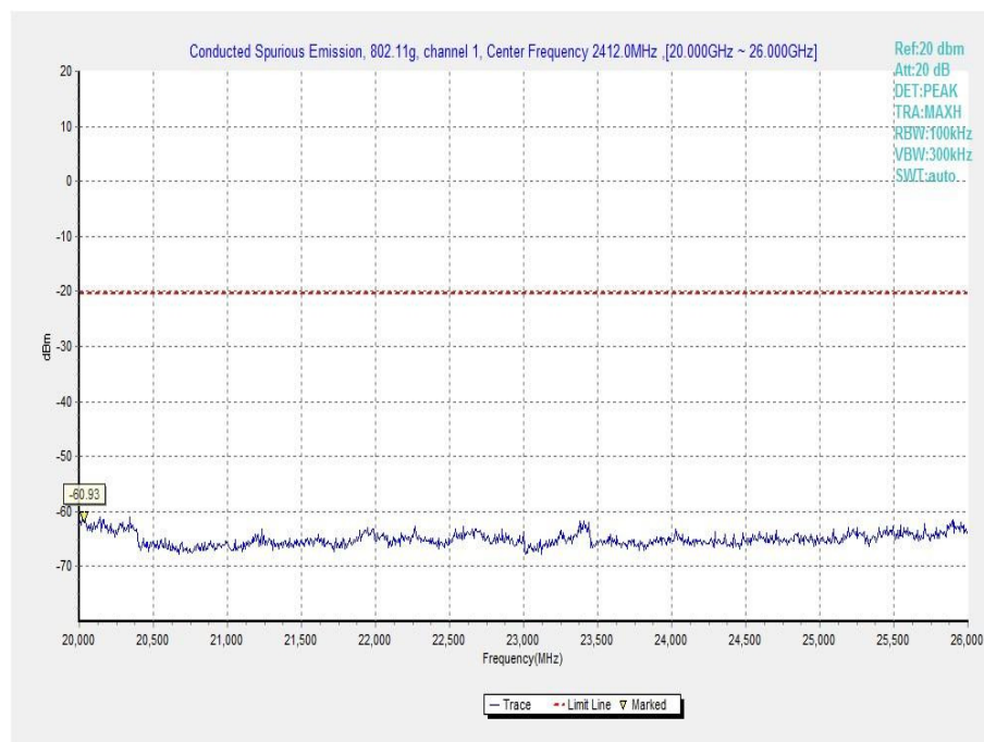
Fig.A.6.1.32 Transmitter Spurious Emission - Conducted (802.11g, Ch1, 20 GHz-26 GHz)
