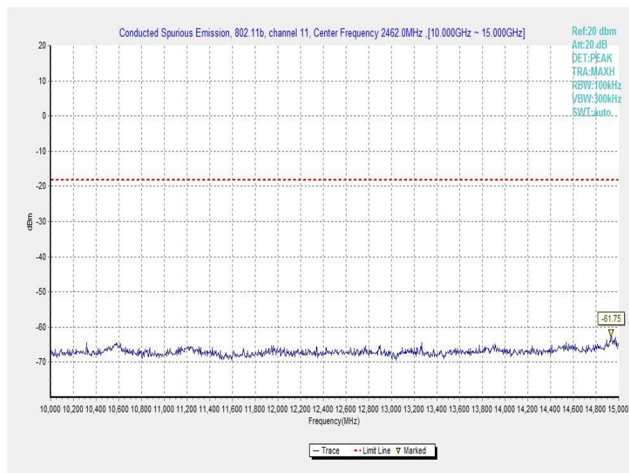
Fig.A.6.1.22 Transmitter Spurious Emission - Conducted (802.11b, Ch11, 10 GHz-15 GHz)
