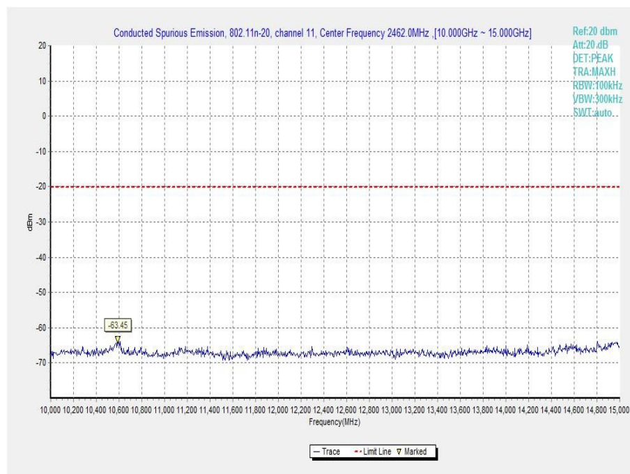
Fig.A.6.1.70 Transmitter Spurious Emission - Conducted (802.11n-HT20, Ch11, 10 GHz-15 GHz)
