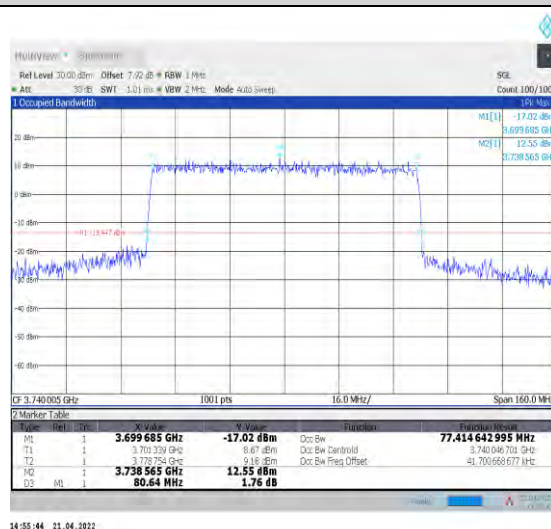
1-N77-3700-3980--30-80-L-8-CP-64QAM-Outer_Full- 217@0-Ant0-77.415-80.640-≤80-PASS
