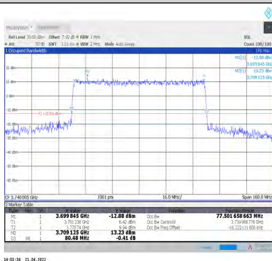
1-N77-3700-3980--30-80-L-7-CP-16QAM-Outer_Full -217@0-Ant0-77.502-80.480-≤80-PASS
