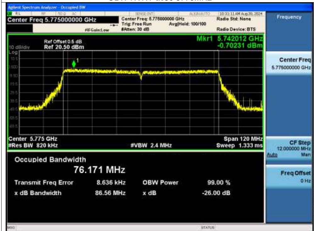
OBW NVNT ac80 5775MHz
