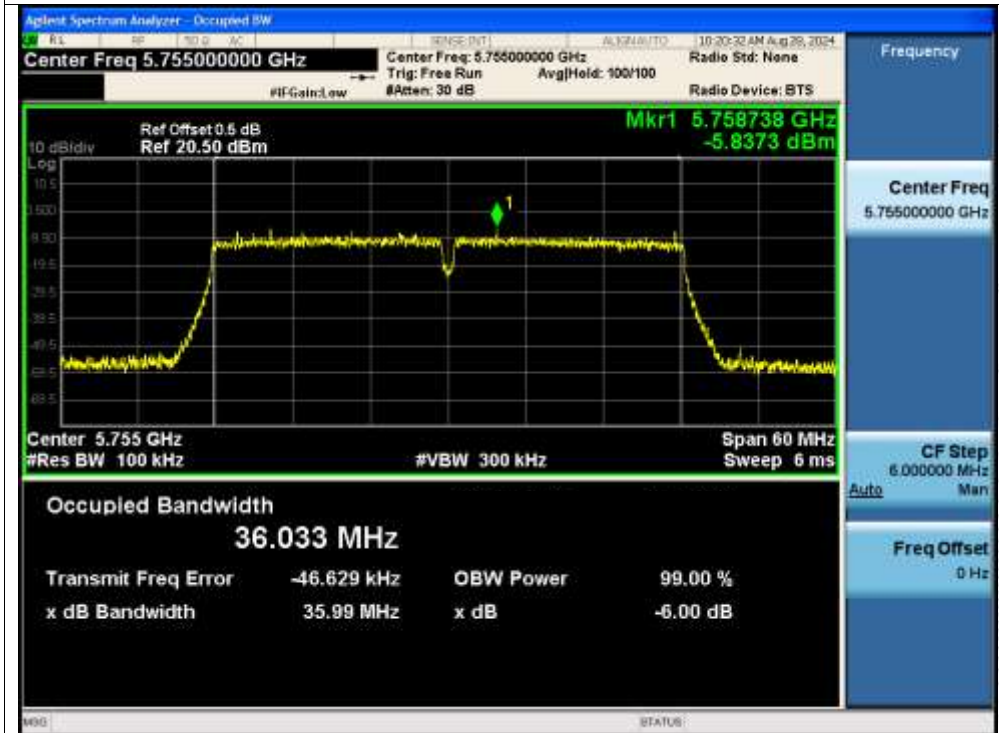
-6dB Bandwidth NVNT ac40 5755MHz
