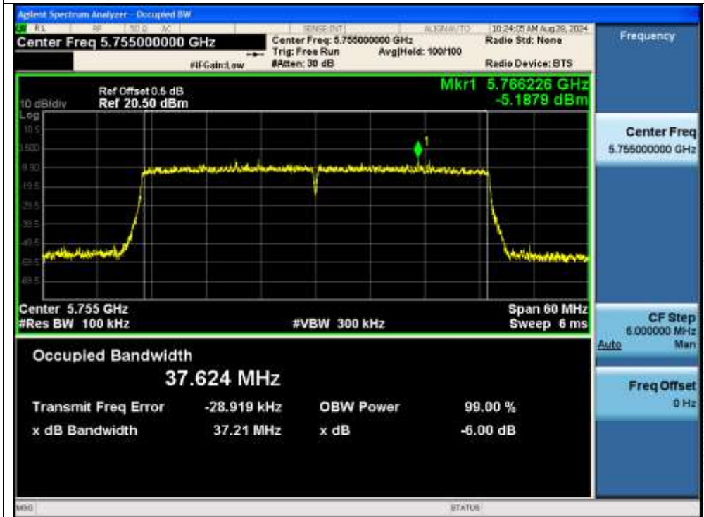
-6dB Bandwidth NVNT ax40 5755MHz
