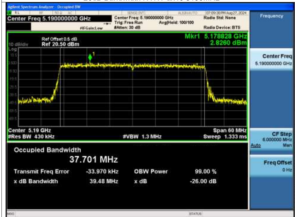
-26dB Bandwidth NVNT ax40 5190MHz
