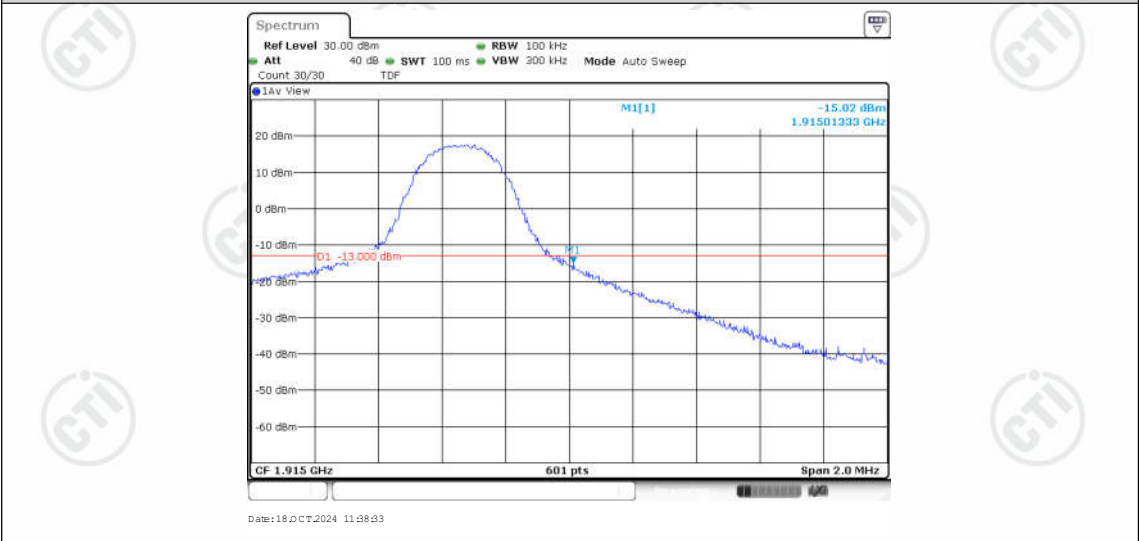
Band25-5MHz-QPSK-26665-1RB#24
