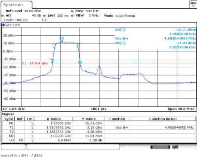
Band25-20MHz-16QAM-26140-25RB#0-4.955
