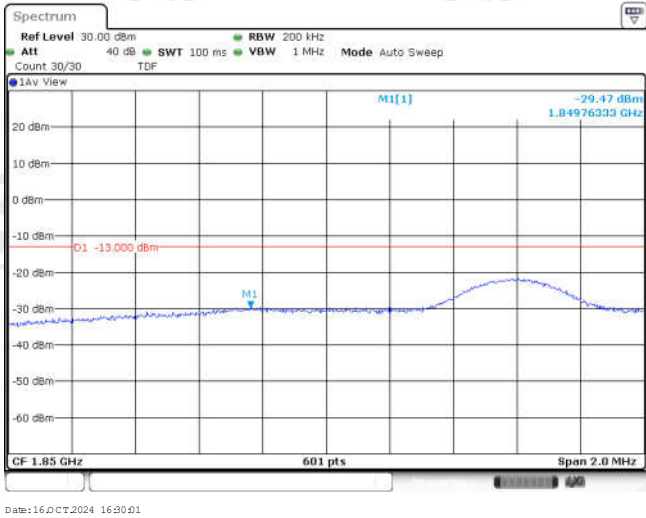
Band25-10MHz-QPSK-26090-1RB#49
