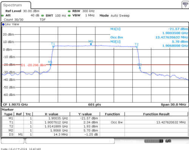
Band25-15MHz-QPSK-26615-75RB#0-13.428
