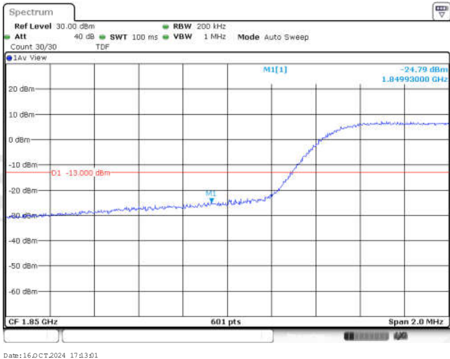
Band25-10MHz-16QAM-26090-25RB#0
