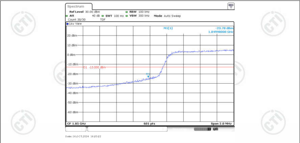
Band25-5MHz-QPSK-26065-25RB#0
