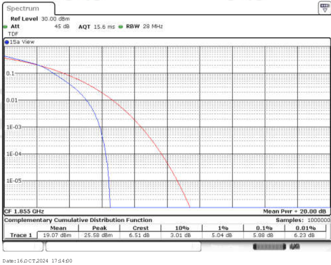
Band25-10MHz-16QAM-26090-25RB#0
