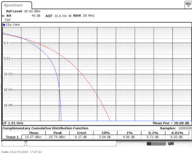
Band25-10MHz-16QAM-26640-25RB#0
