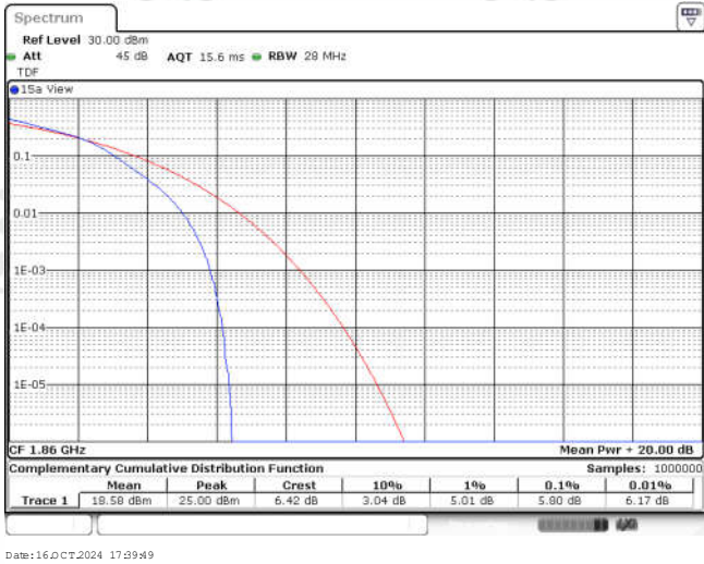
Band25-20MHz-16QAM-26140-25RB#0
