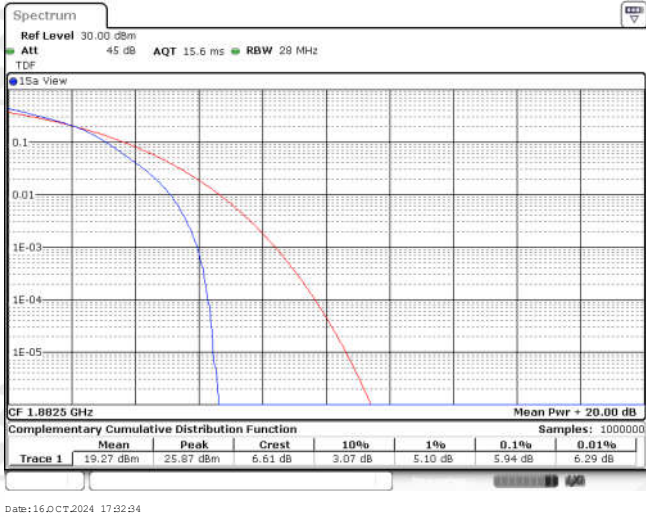
Band25-15MHz-16QAM-26365-25RB#0
