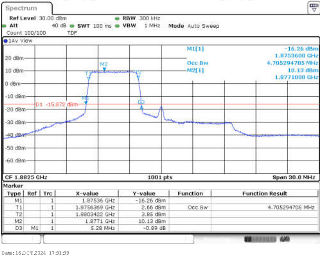
Band25-15MHz-16QAM-26365-25RB#0-4.705
