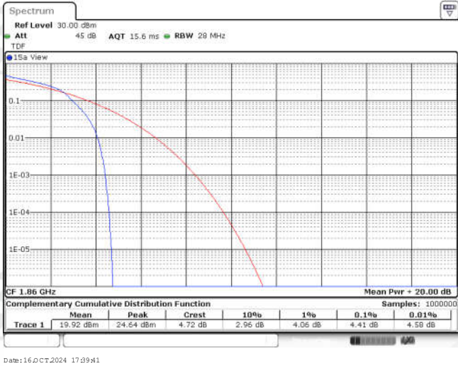
Band25-20MHz-16QAM-26140-1RB#0
