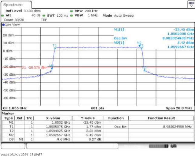
Band25-10MHz-QPSK-26090-50RB#0-8.985
