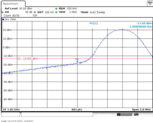
Band25-10MHz-QPSK-26090-1RB#0
