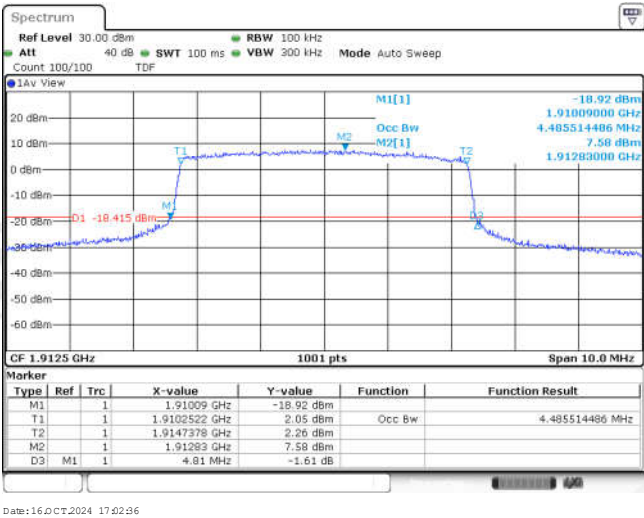
Band25-5MHz-16QAM-26665-25RB#0-4.486
