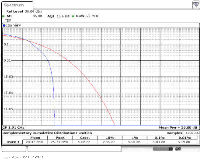
Band25-10MHz-16QAM-26640-1RB#0
