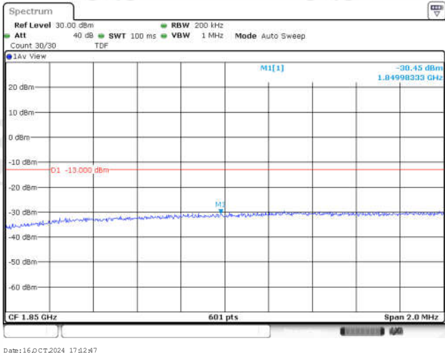
Band25-10MHz-16QAM-26090-1RB#24
