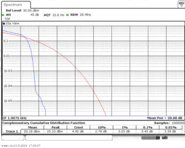
Band25-15MHz-16QAM-26615-1RB#0
