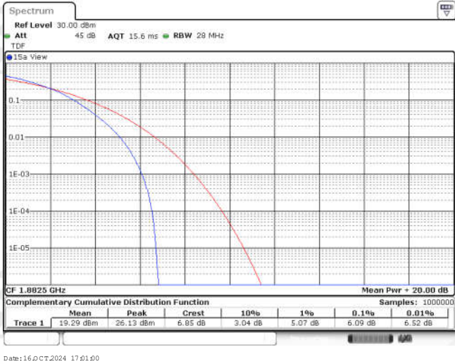
Band25-5MHz-16QAM-26365-25RB#0
