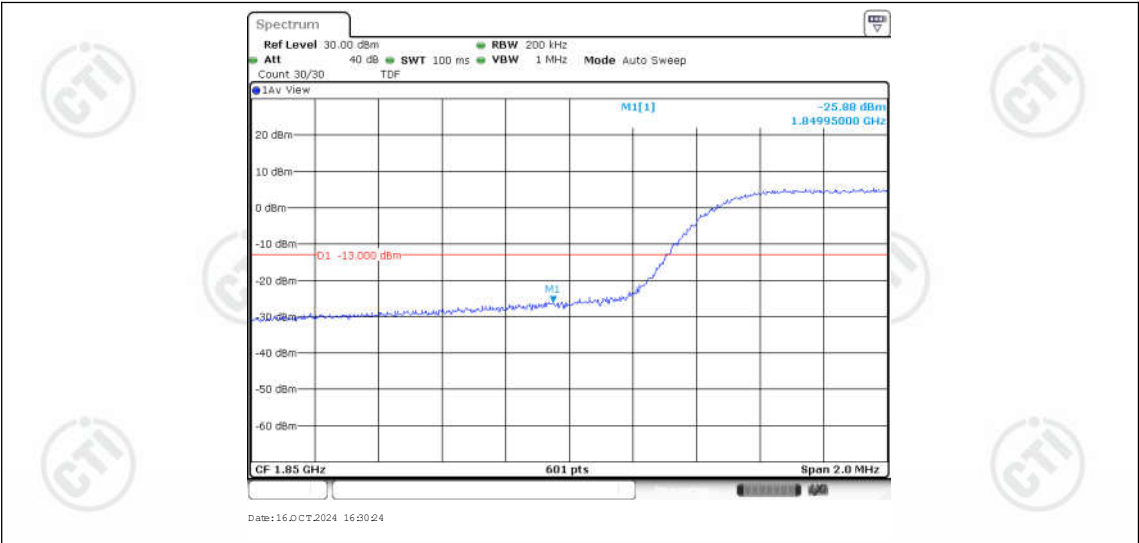
Band25-10MHz-QPSK-26090-50RB#0
