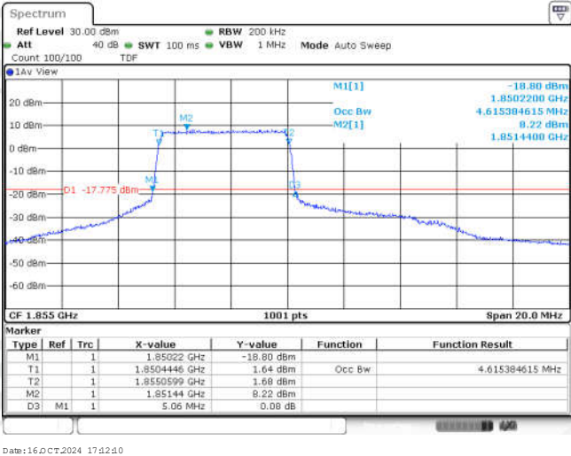
Band25-10MHz-16QAM-26090-25RB#0-4.615
