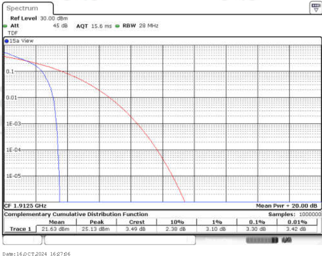
Band25-5MHz-QPSK-26665-1RB#0
