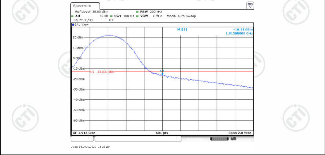
Band25-10MHz-QPSK-26640-1RB#49
