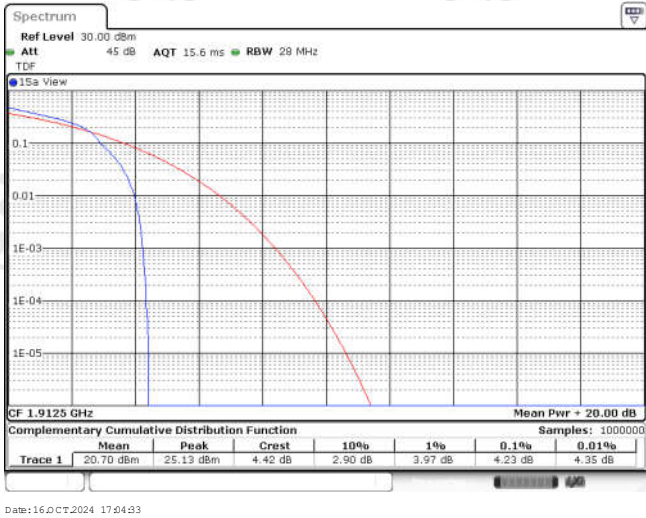
Band25-5MHz-16QAM-26665-1RB#0
