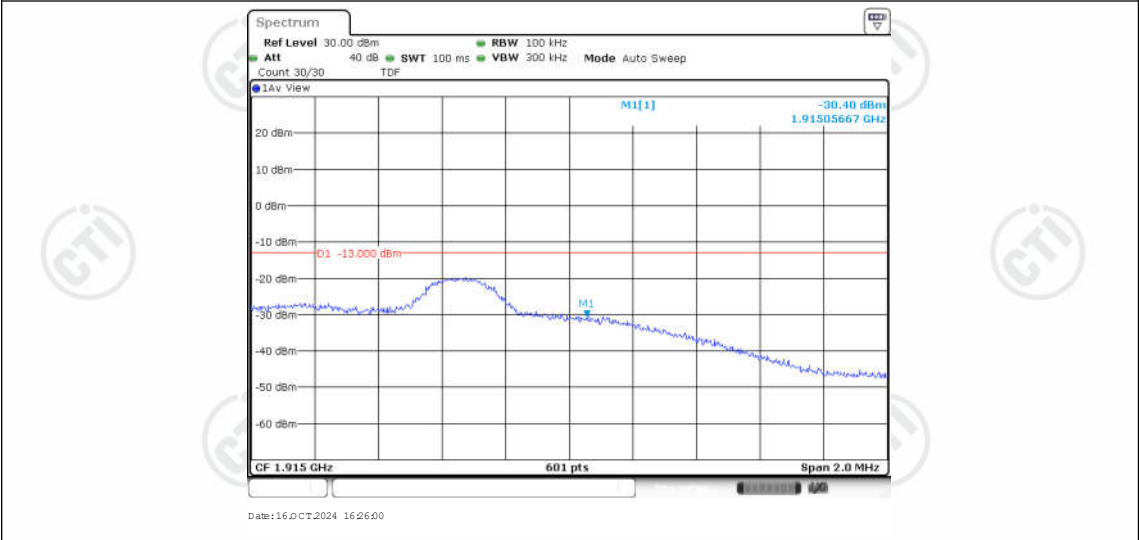
Band25-5MHz-QPSK-26665-1RB#0
