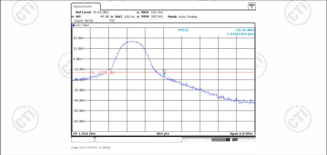
Band25-5MHz-16QAM-26665-1RB#24
