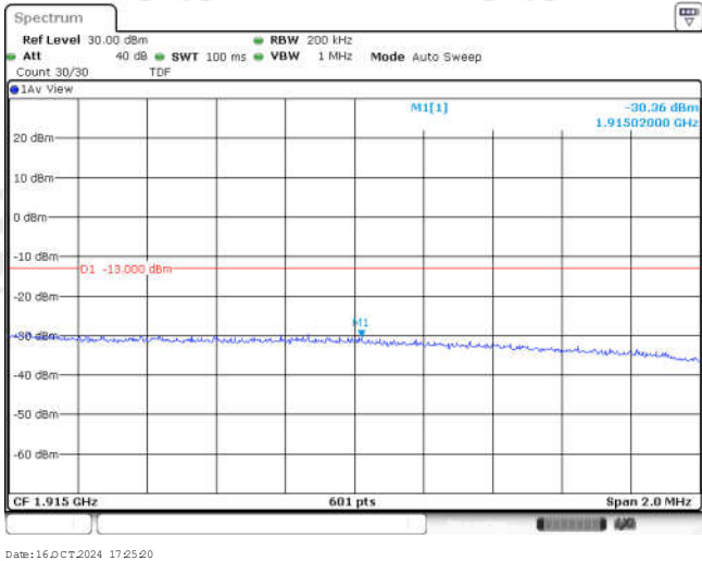
Band25-10MHz-16QAM-26640-1RB#24
