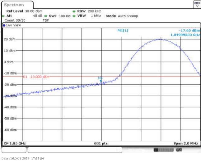
Band25-10MHz-16QAM-26090-1RB#0
