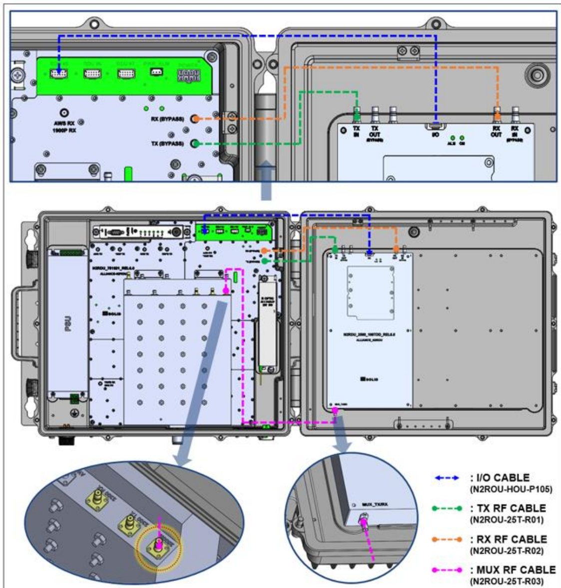
Figure 4.15 –N2RDU_2500_100TDD Cabling
