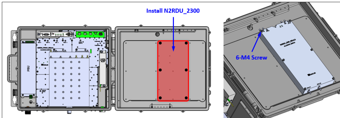
Figure 4.21 – Install N2RDU_2300
