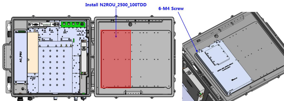
Figure 4.14 – Install N2RDU_2500TDD
