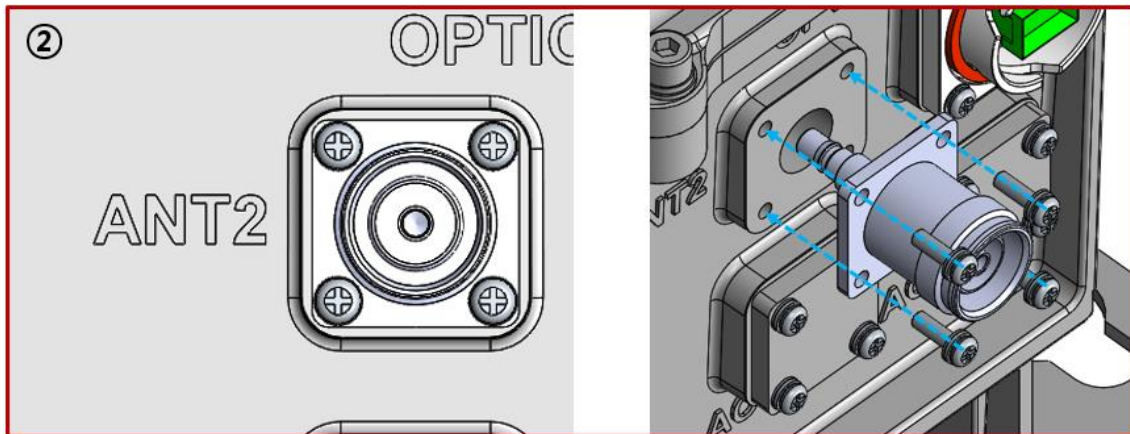
Figure 4.26 – Installing MIMO Antenna Adaptor
