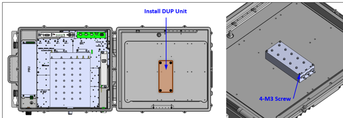
Figure 4.17 – Install DUP Module
