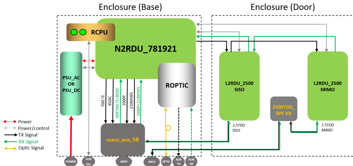
Figure 3.3 – N2ROU Block Diagram (2.5TDD MIMO Supported)
