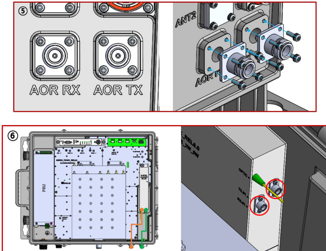
Figure 4.27 – Preliminary Work for Installing AOR
