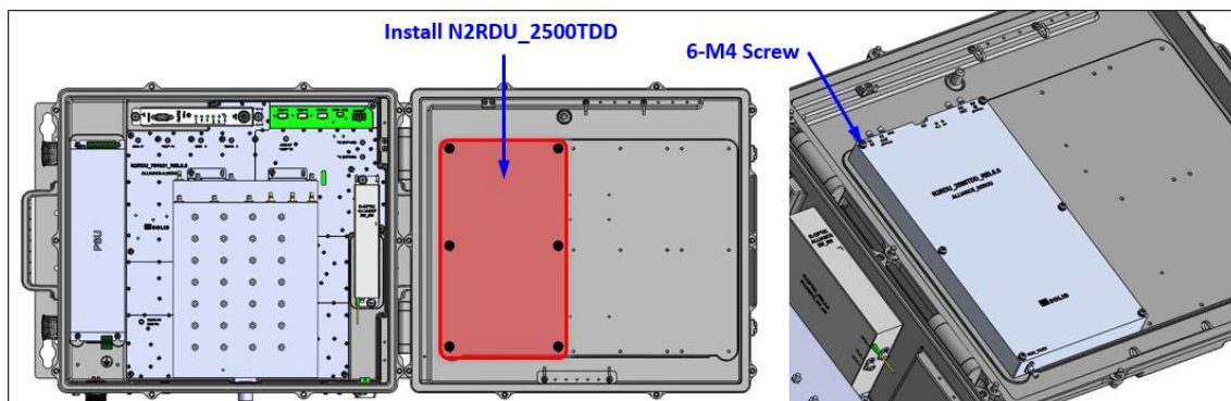
Figure 4.12 – Install N2RDU_2500TDD
