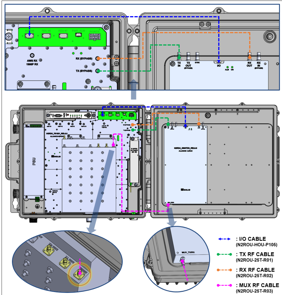
Figure 4.13 –N2RDU_2500TDD Cabling
