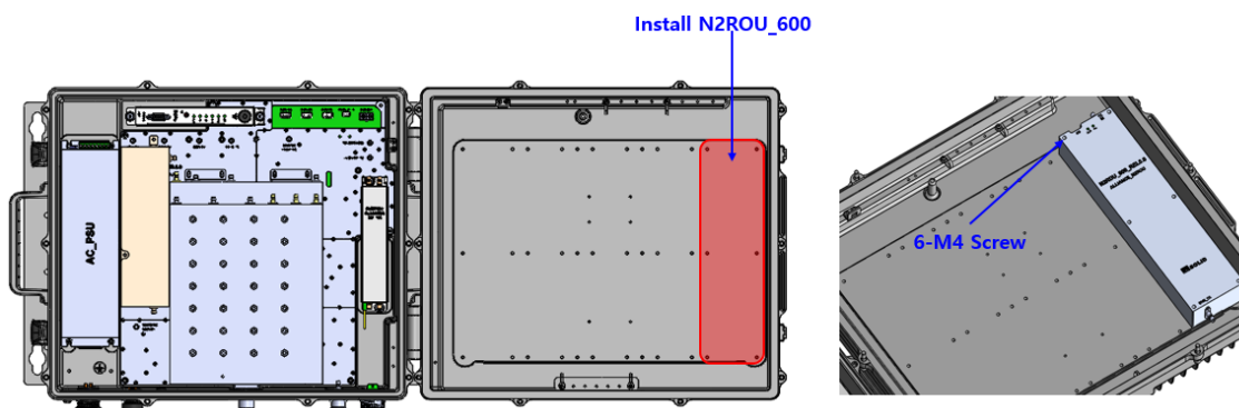
Figure 4.24 – Install N2RDU_600
