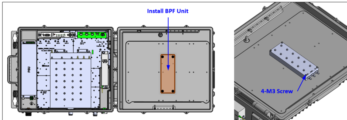
Figure 4.19 – Install BPF Module
