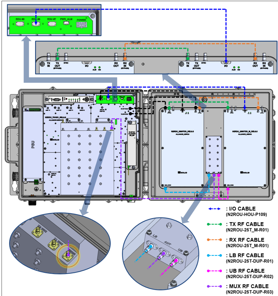
Figure 4.18 – Cabling of N2ROU_2500TDD_M (2500TDD Band Expansion)
