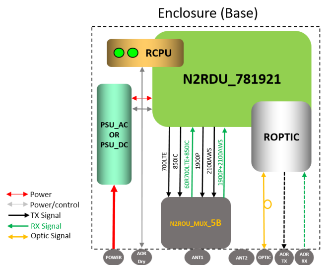
Figure 3.1 – N2ROU Block Diagram (4 Bands)
