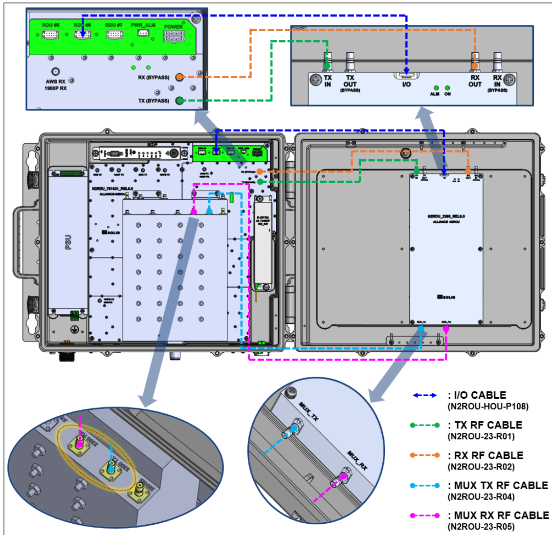
Figure 4.22 – Cabling of N2RDU_2300 (Solely used)
