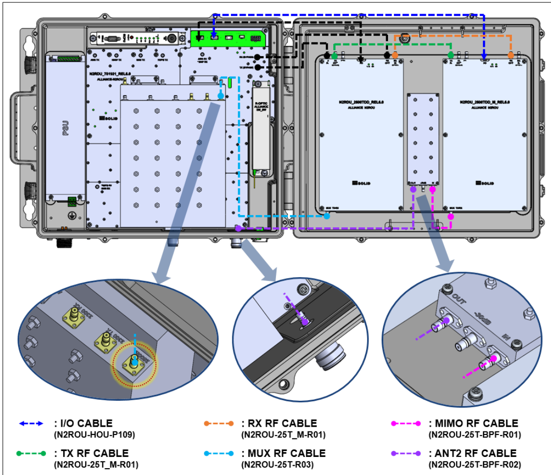
Figure 4.20 –N2ROU_2500TDD_M (2500TDD MIMO Supported) Cabling
