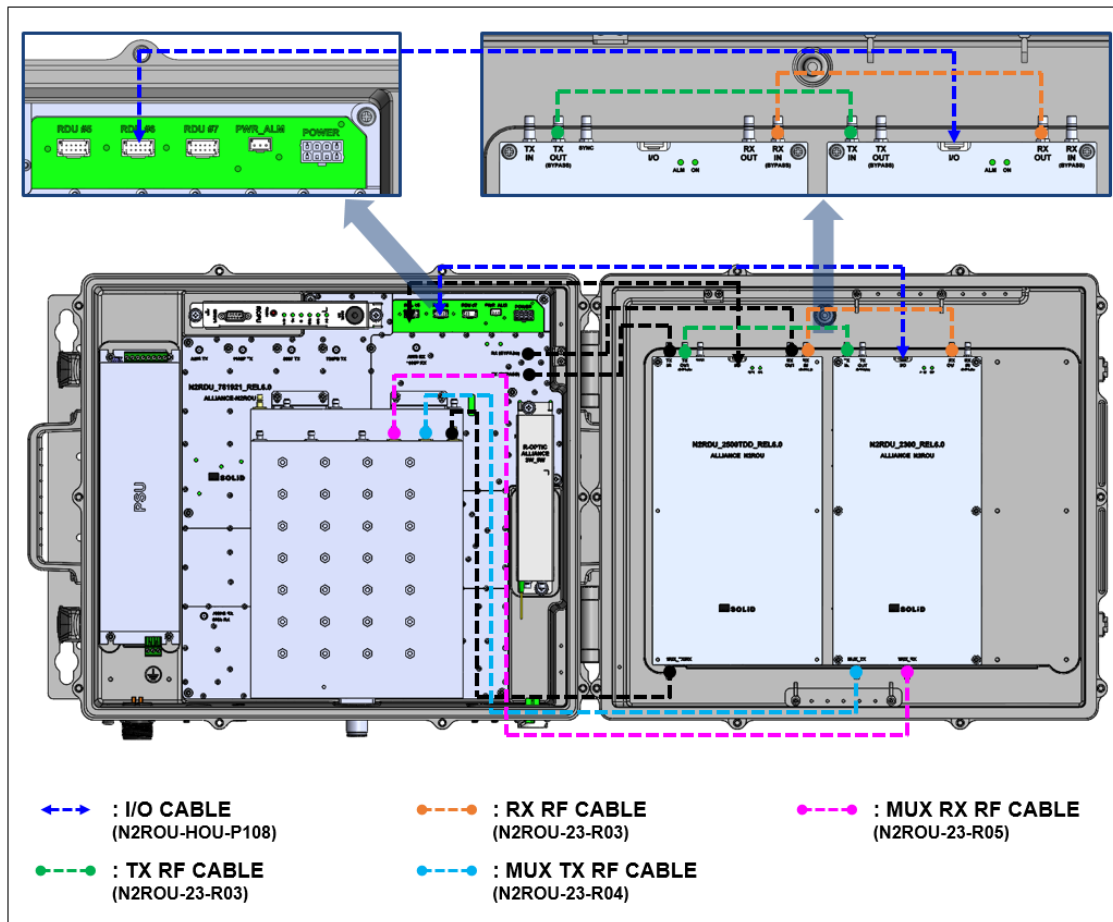
Figure 4.23 – Cabling of N2RDU_2300 (Used with N2RDU_250TDD)
