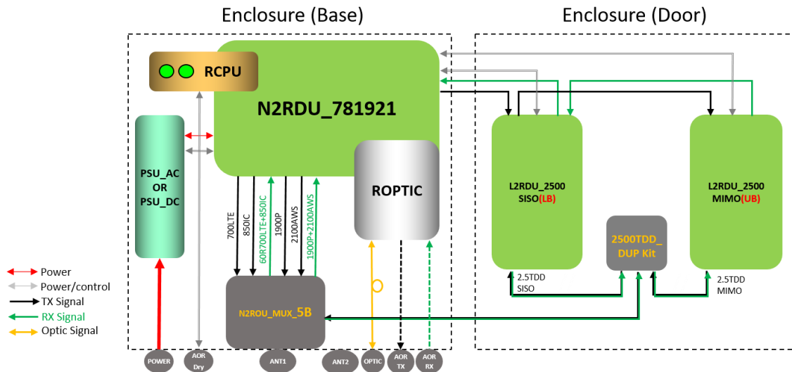
Figure 3.4 – N2ROU Block Diagram (2.5TDD Band Expansion)
