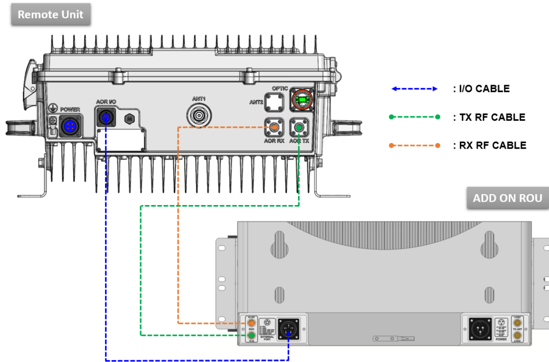
Figure 4.28 – Connecting Diagram between N2ROU and AOR
