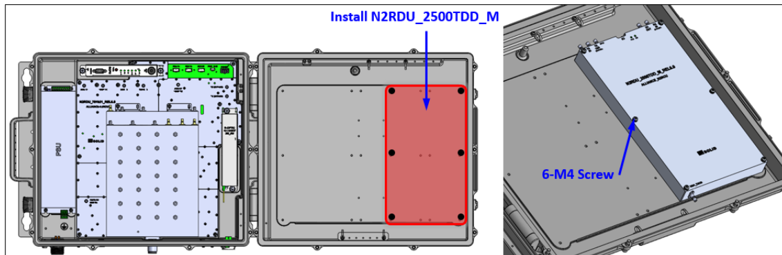
Figure 4.16 – Install N2RDU_2500TDD_M
