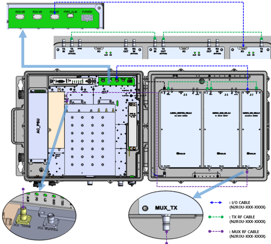
Figure 4.25 – Cabling of N2RDU_600(Used with N2RDU_2300WCS, 2.5TDD)
