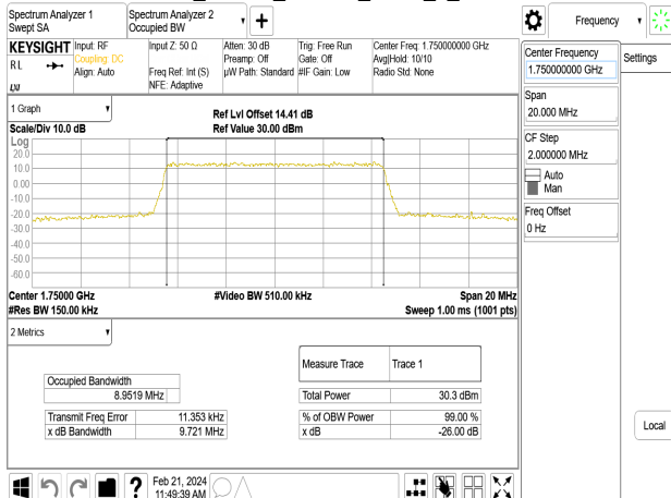
Band4_10MHz_16QAM_RB50_0_CH20350
