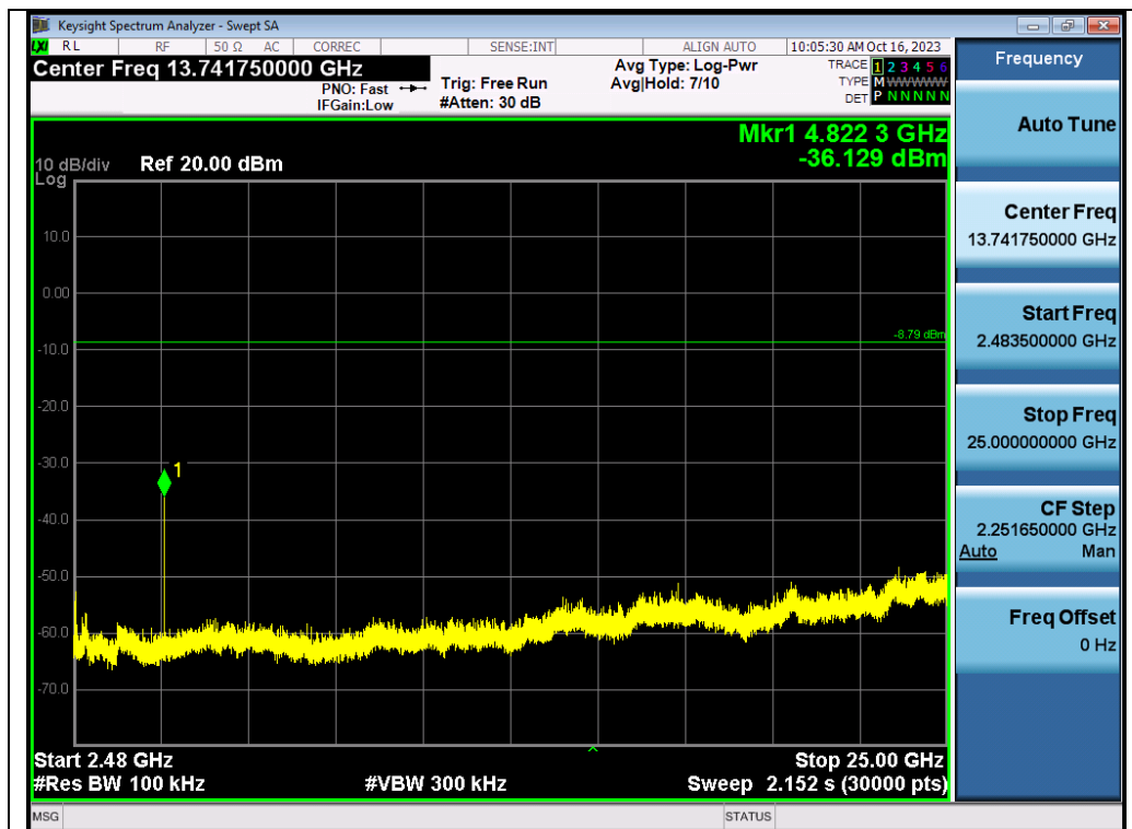
Test_Graph_GFSK_ANT1_2410_Higher Band Emissions
