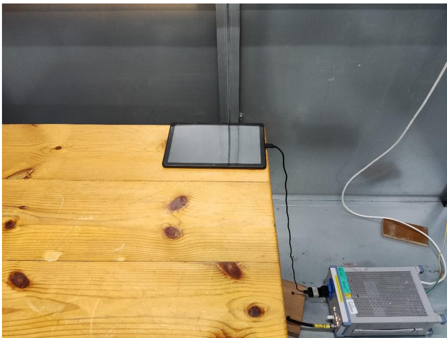
10. Conducted Emission (Part 15B, Camera/Video Player)
