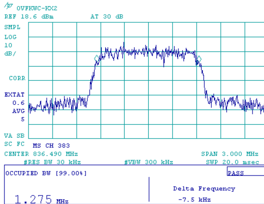
Figure 8-8 CDMA 800 at RC1
