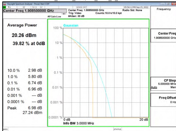
Band2_3MHz_16QAM_RB6_0_CH19185
