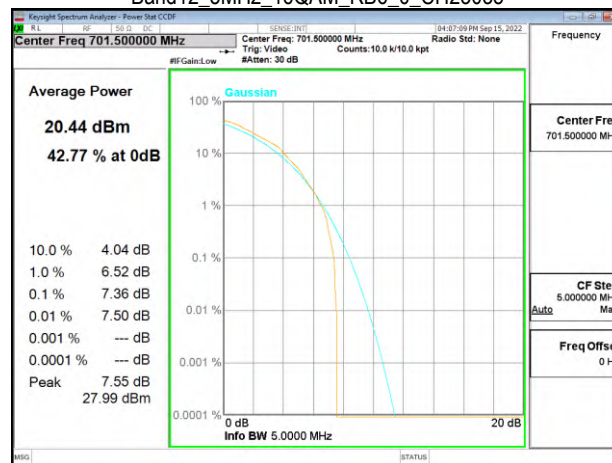
Band12_5MHz_16QAM_RB6_0_CH23095
