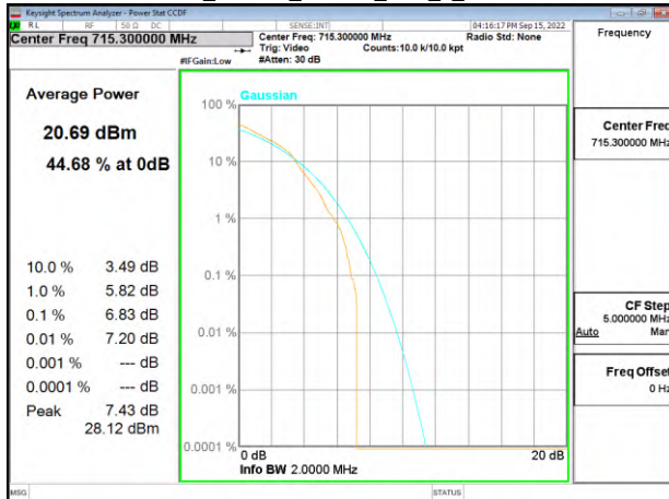
Band12_1.4MHz_16QAM_RB6_0_CH23173
