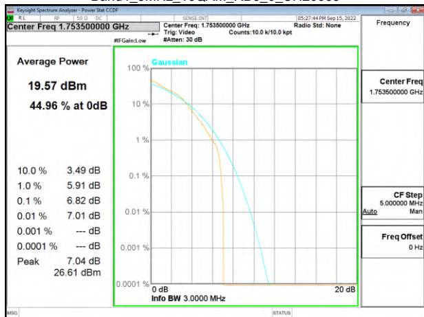
Band4_3MHz_16QAM_RB6_0_CH20385
