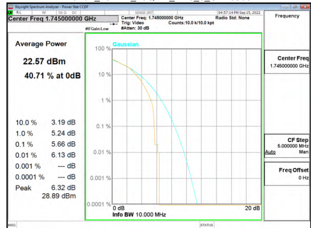
Band4_20MHz_16QAM_RB6_0_CH20300
