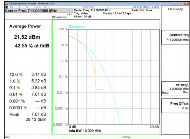
Band12_10MHz_16QAM_RB6_0_CH23130
