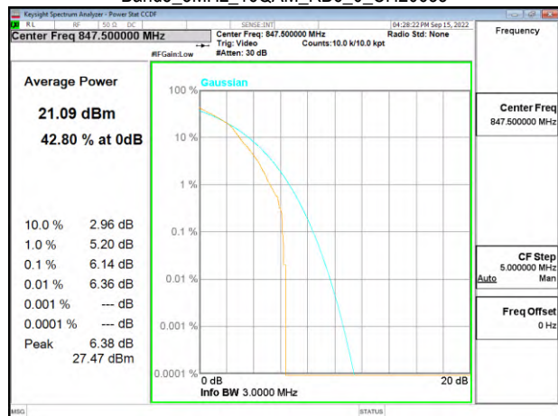
Band5_3MHz_16QAM_RB6_0_CH20635
