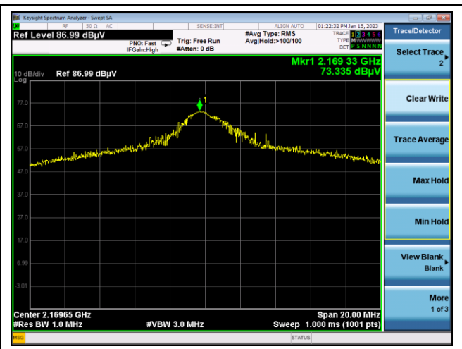
5 th harmonic
