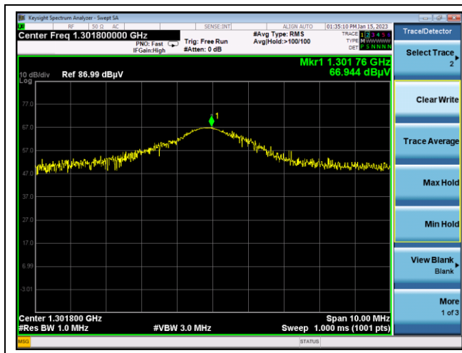
3 rd harmonic
