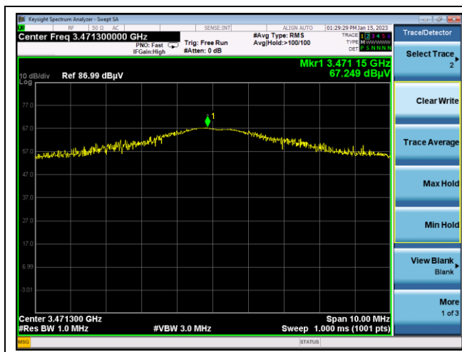
8 th harmonic
