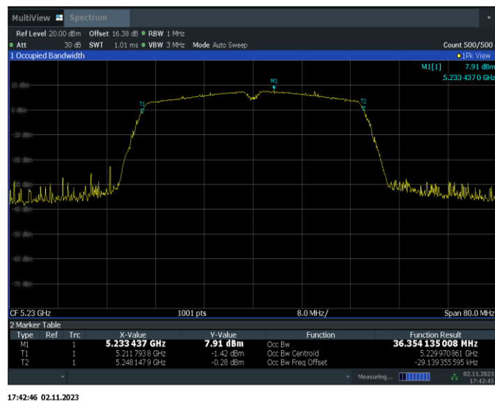
Fig.67 99% Occupied bandwidth (802.11ac-VHT40, 5230MHz)
