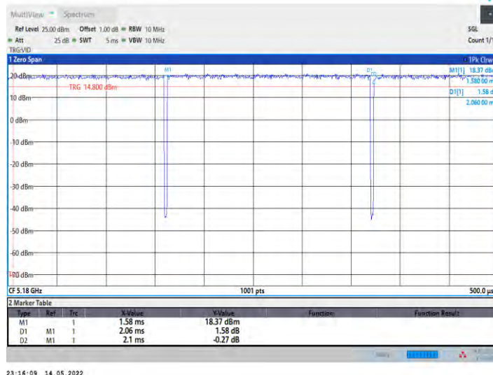
11n20SISO_Ant0_5180
