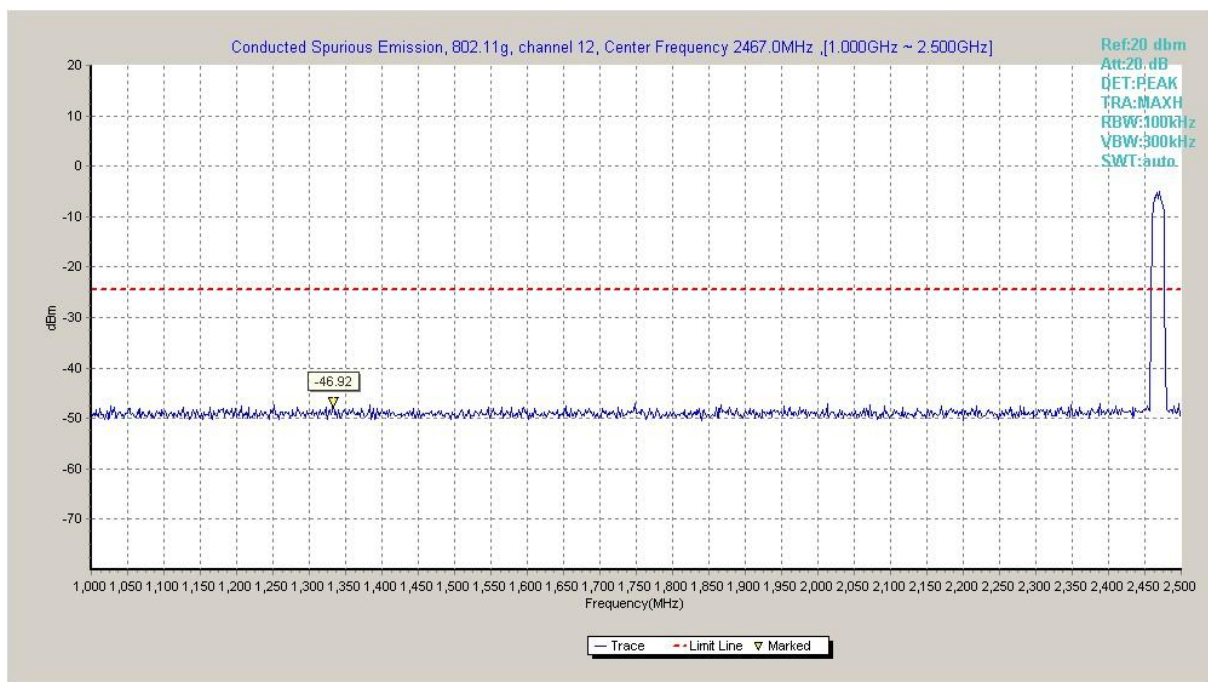
Fig.A.6.1.67 Transmitter Spurious Emission - Conducted (802.11g, Ch12, 1 GHz-2.5 GHz)
